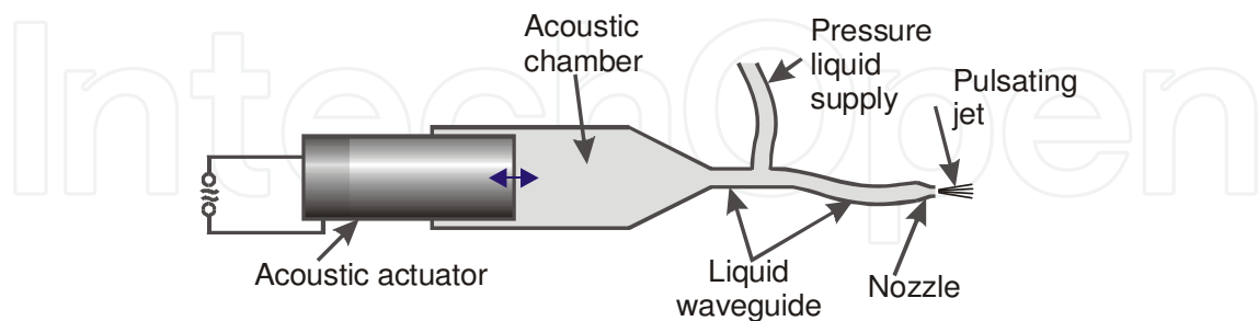
Fig. 3. Schematic drawing of the high-pressure system with integrated acoustic generator of pressure pulsations
