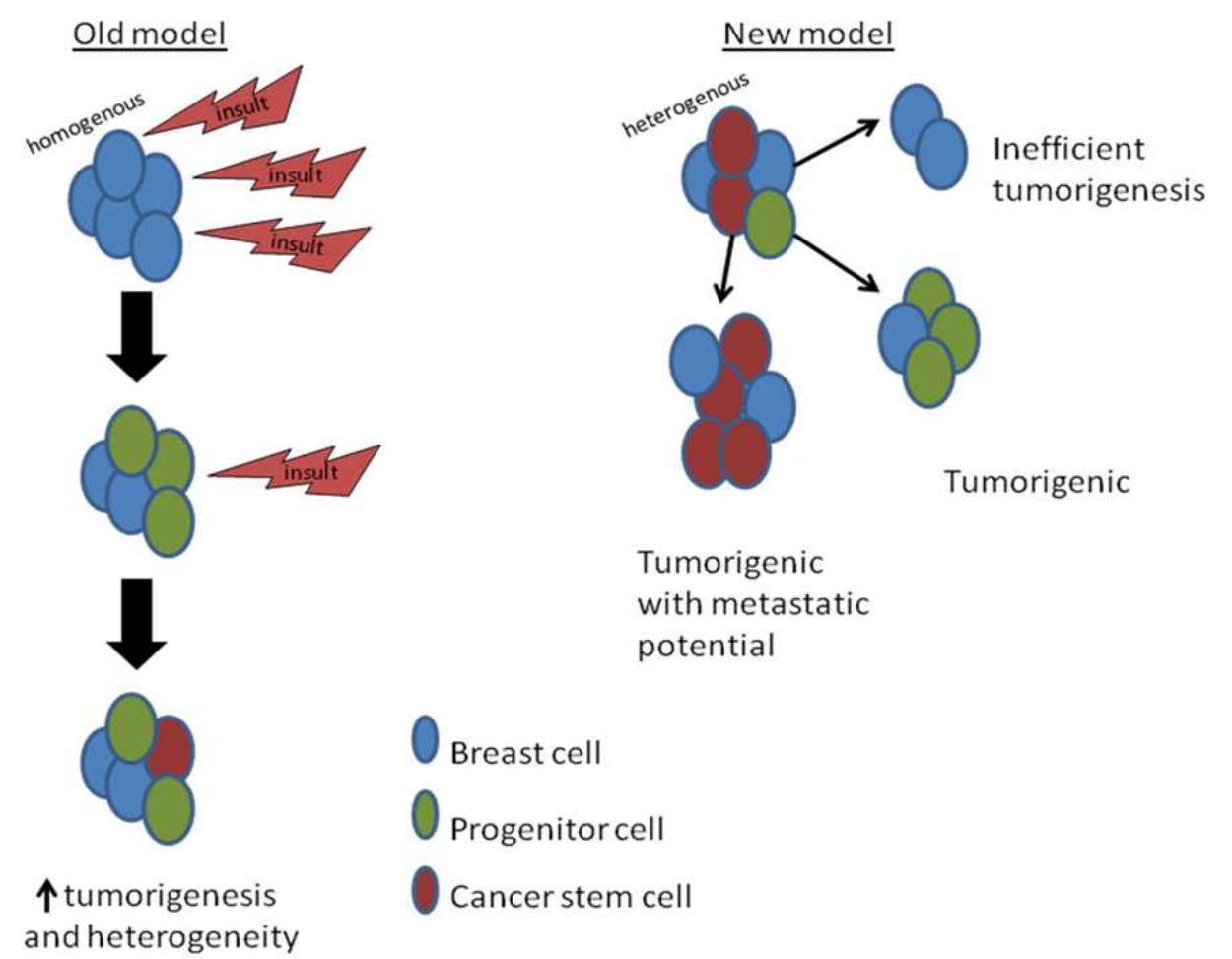
Fig. 3. Theories of breast cancer progression. The old model of breast cancer progression assumed that all breast cells have equal potential to become tumorigenic with repetitive insults. The new model contends that the breast cells are heterogenous from the start with differing potentials for tumorigenesis, thus resulting in heterogenous breast cancers.
