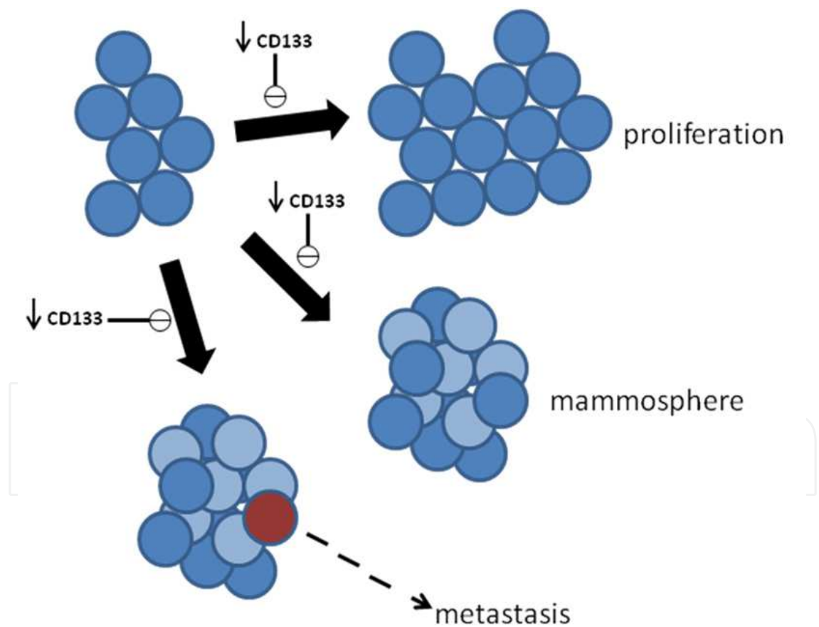
Fig. 2. Role of CD133 in breast cancer. CD133 downregulation results in poor mammosphere formation, less metastasis, and less proliferation, suggesting a potential target for breast cancer treatment. Furthermore, CD133 is more specific to breast cancer stem cells than many other markers such as CD44, showing additional importance in the role of cancer progression and characterization.
