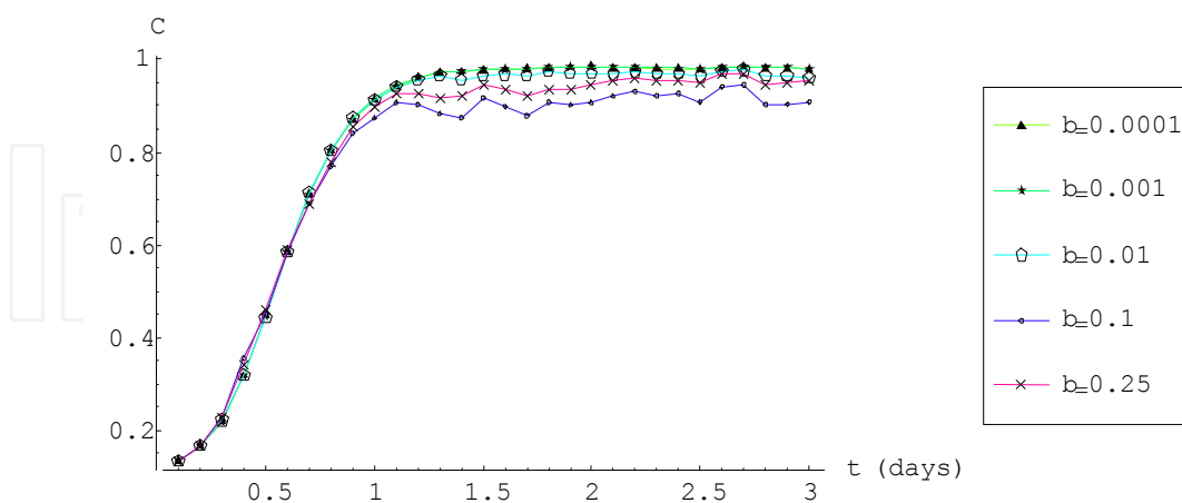
Figure 3.5. Concentration profiles at x = 0.5 \text{ m} for \sigma^2 = 0.001 .
