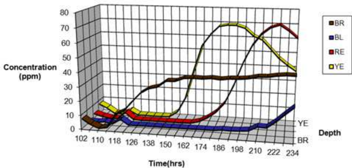
Figure 3.20. Concentration profiles at Row 5 - Well B.
