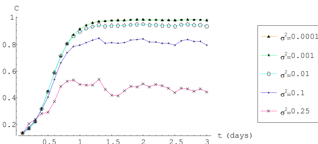
Figure 3.10. Concentration profiles at x = 0.5 m for b = 0.001 .
