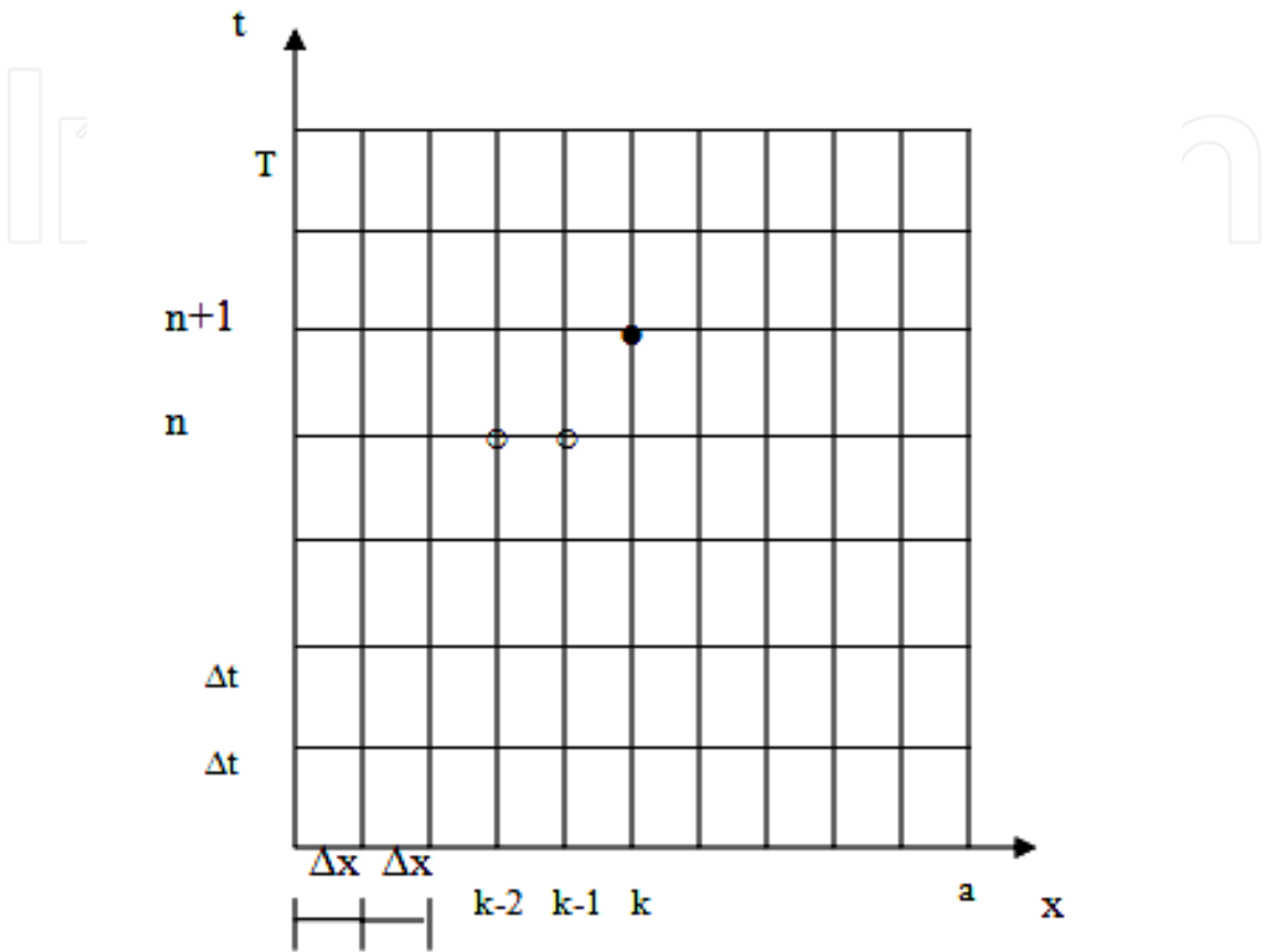
Figure 3.2. An explicit space-time scheme used for the computational solution.
