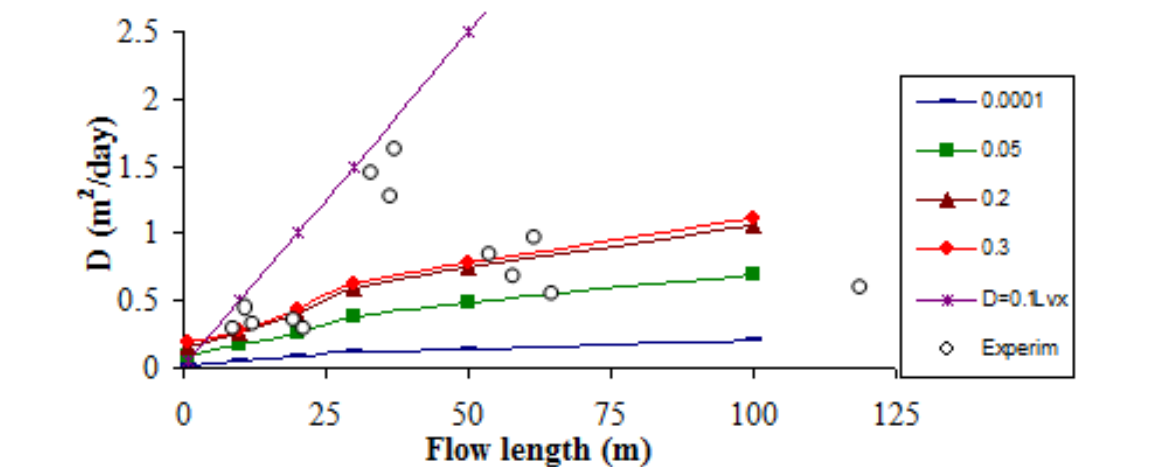
Figure 3.36. Estimated D values for b = 0.01 m for range of \sigma^2 (0.0001 - 0.3), D = 0.1 L v , and reliable field measurements observed by Gelhar (1986) for different flow lengths.
