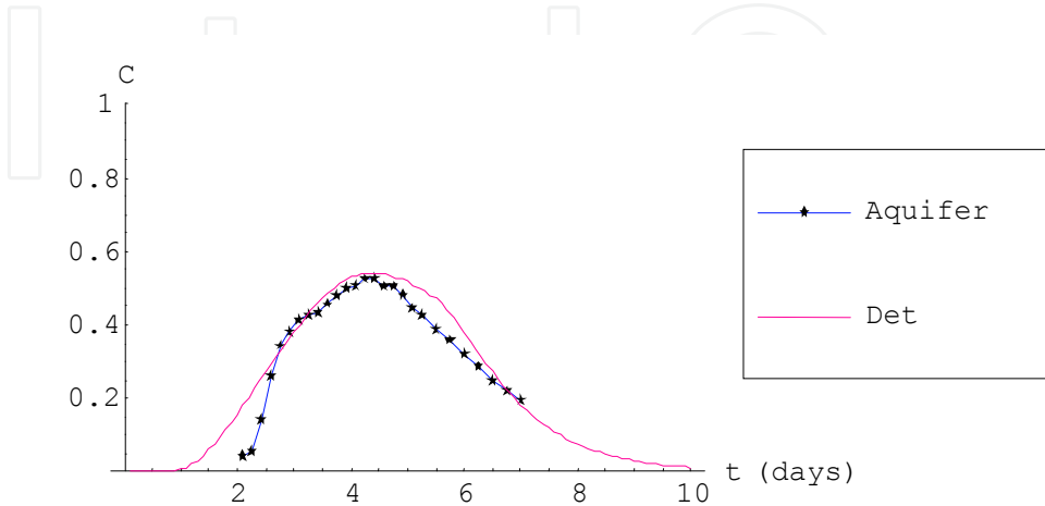
Figure 3.16. Concentration profiles of 2-D deterministic advection-dispersion model ( D = 0.15 \text{ m}^2/\text{day} ) and the experimental aquifer.
