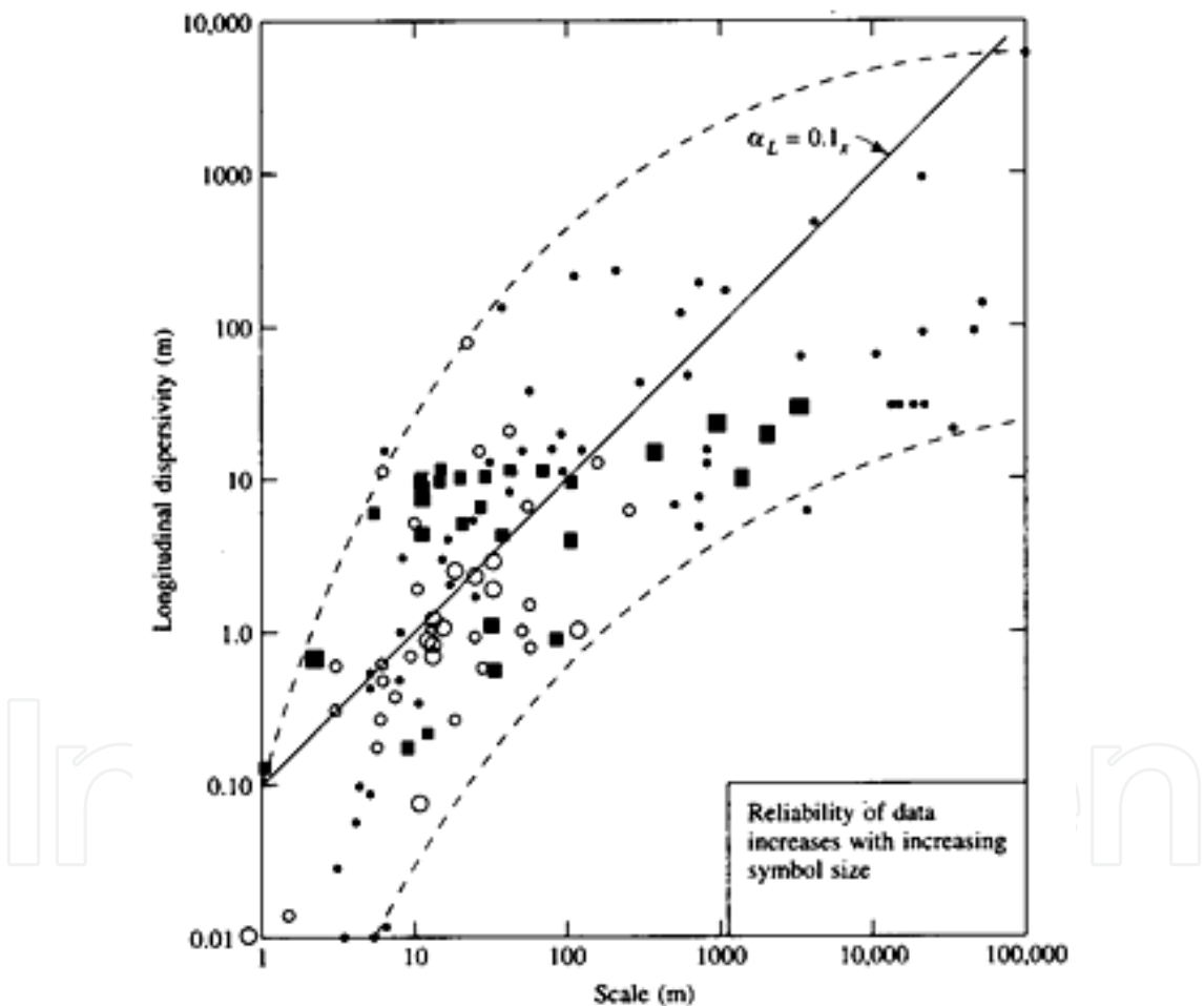
Figure 3.34. Field measured values of longitudinal dispersivity as a function of the scale of measurement. The largest circles represent the most reliable data. The estimated dispersivity from the SSTM are given by the squares. (Source: Gelhar (1986).)
