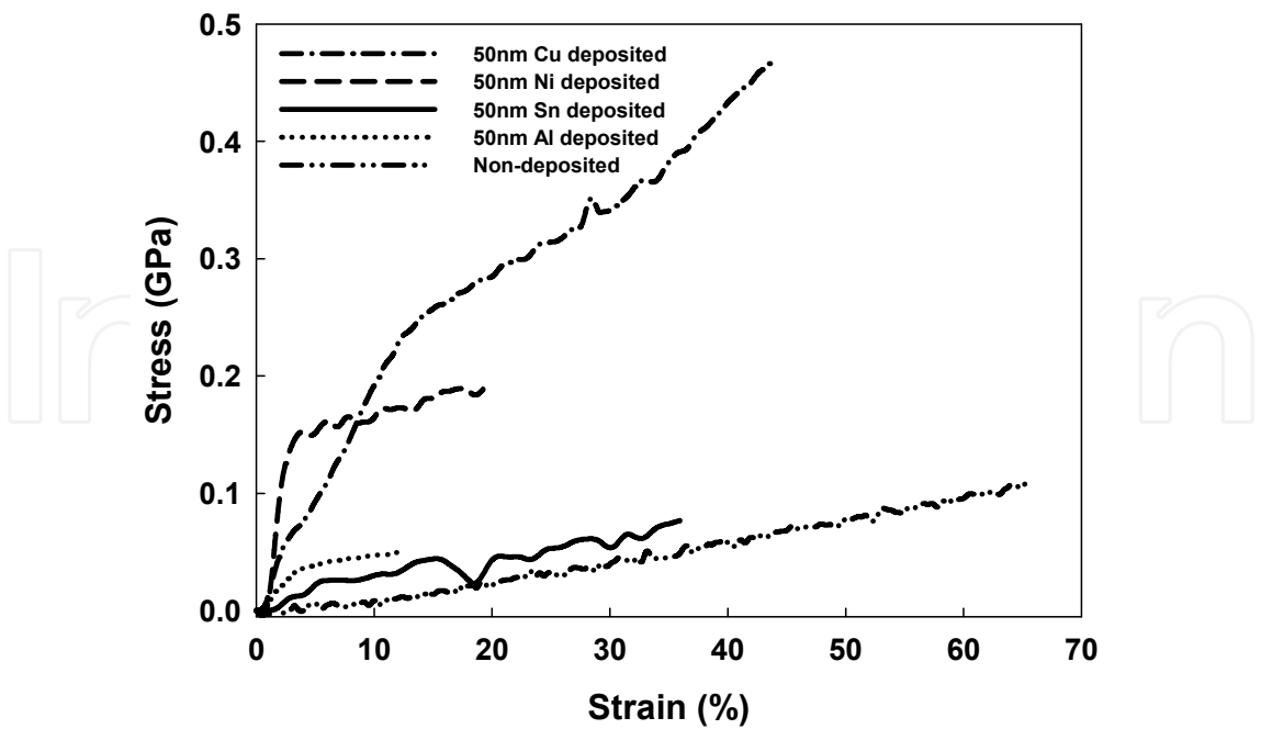
Fig. 14. Stress–strain curves of Cu-deposited (dash-dot line), Ni-deposited (medium dash line), Sn-deposited (solid line), Al-deposited (dotted line), and pure (dash-dot-dot line) single PU nanofibers (load: 10 mN, loading speed: 15 \text{mm s}^{-1} ).
