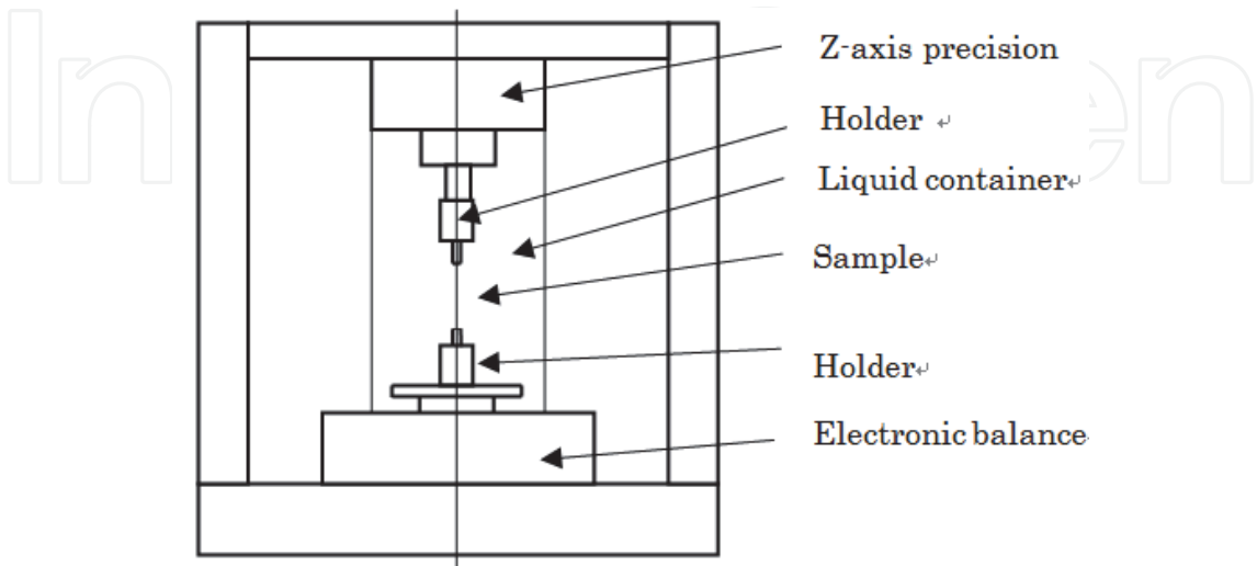
Fig. 11. Specially developed tensile test machine.
