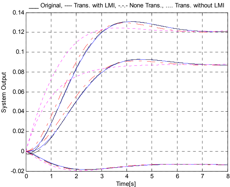
Fig. 9. Reduced 3 rd order models (.... transformed without LMI, -.-.- non-transformed, ---- transformed with LMI) output responses to a step input along with the non reduced ( ____ original) system output response. The LMI-transformed curve fits almost exactly on the original response.
