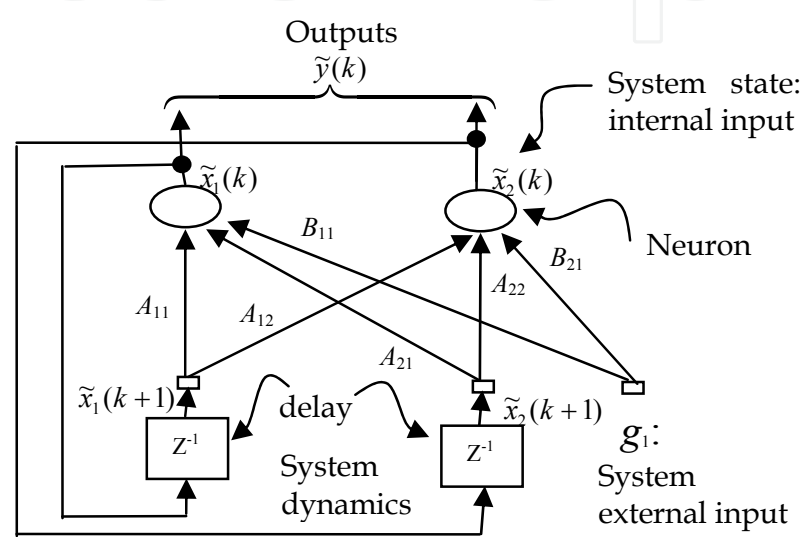
Fig. 3. The utilized 2 nd order recurrent neural network architecture, where the identified matrices are given by \{ \tilde{A}_d = \begin{bmatrix} A_{11} & A_{12} \\ A_{21} & A_{22} \end{bmatrix}, \tilde{B}_d = \begin{bmatrix} B_{11} \\ B_{21} \end{bmatrix} \} and that W = \begin{bmatrix} \tilde{A}_d & \tilde{B}_d \end{bmatrix} .
