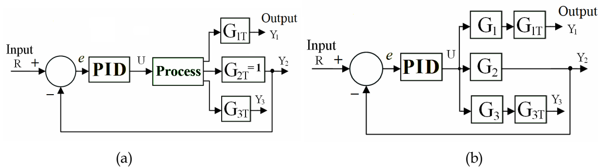
Fig. 14. Closed-loop feedback single-input multiple-output (SIMO) system with a PID controller: (a) a generic SIMO diagram, and (b) a detailed SIMO diagram. As shown in Figure 14, the tuning process is accomplished using G_{1T} and G_{3T} . For example, for the 1 st output:
