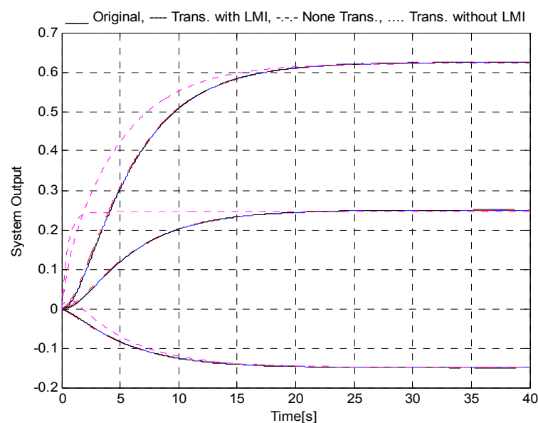
Fig. 11. Reduced 3 rd order models (.... transformed without LMI, -.-.- non-transformed, ---- transformed with LMI) output responses to a step input along with the non reduced ( ____ original) system output response. The LMI-transformed curve fits almost exactly on the original response.
