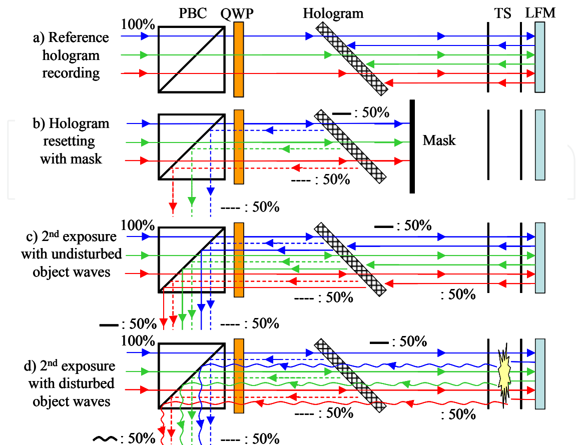
Fig. 8. Formation of colour interference fringes in optical setup
