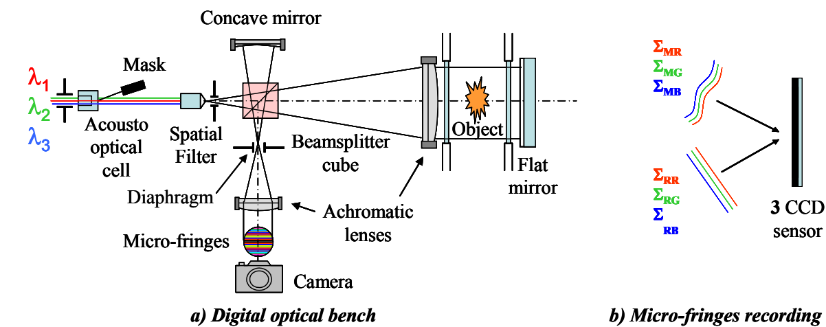
Fig. 13. Digital colour holographic interferometer – Formation of spatial carrier frequencies
