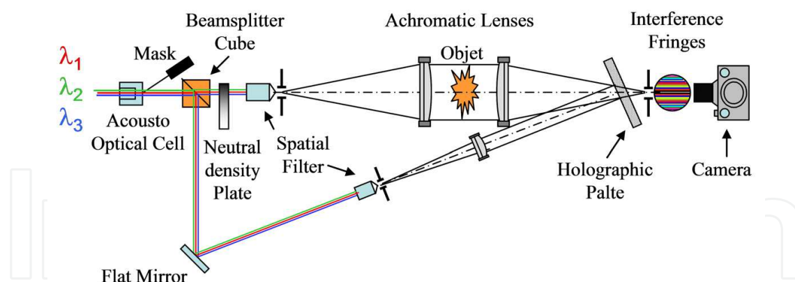
Fig. 3. Real-time colour holographic interferometry setup (Transmission mode)
