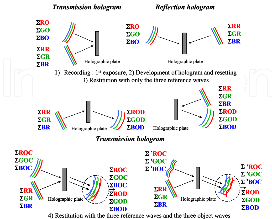
Fig. 2. Formation of colour interference fringes
