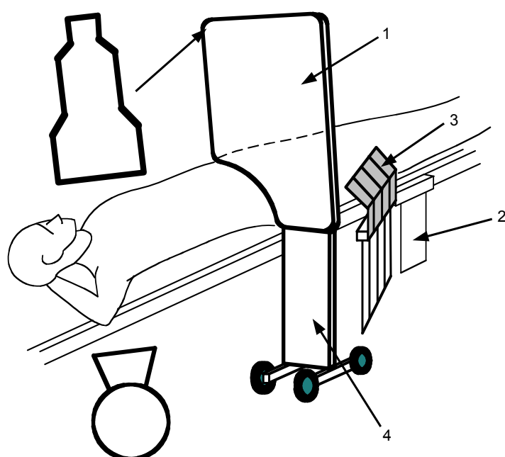
Fig. 1. Example of operator shielding with various devices (1 leaded glass, 2 and 3 leaded curtains, 4 leaded wall; 1 and 4 being on a mobile barrier)
