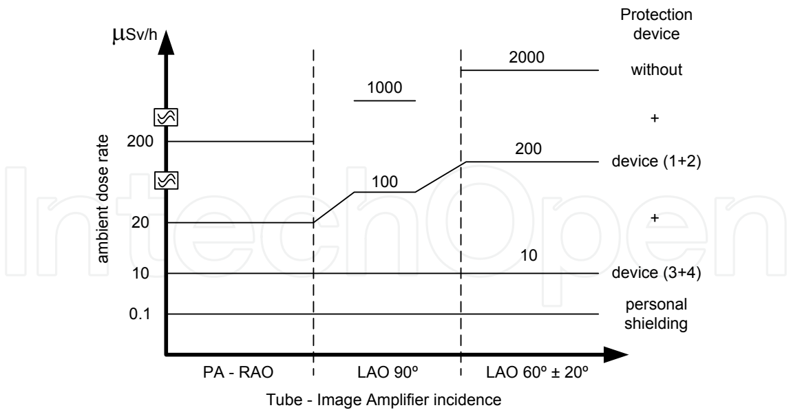
Fig. 2. Mean ambient dose rate to the operator ( \mu\text{Sv.h}^{-1} ) for different tube-image amplifier orientations. The dose rate corresponds to an examination in the cardiac area of a Rando phantom, representative of a 70 kg standard patient, the operator being at about 1 m from the central beam impinging the phantom (situation presented in Figure 1). Without any radiation protection device, the dose rate is in the range of 2 to 0.2 mSv.h -1 . As expected, the LAO angulations are the ones which potentially deliver the highest dose to the operator. The addition of the protection devices 1 and 2 allows a reduction of the ambient dose rate at operator's level by a factor of 10. A further reduction is obtained by completing the shielding with devices 3 and 4. Finally, the use of personal shielding devices (i.e. lead apron, thyroid shield and leaded glasses) reduces the ambient dose rate to about 0.1 \mu\text{Sv.h}^{-1} (adapted from Kuon et al., 2002).
