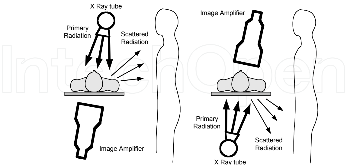
Fig. 3. The schematics show the influence of the tube-image amplifier orientation on the operator's exposure. When the tube is below the table, exposure to the legs and the lower part of the abdomen is the highest. When the tube is above the table, exposure to the face, neck and chest is the highest.
