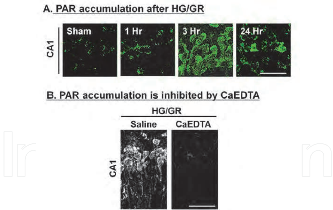
Fig. 6. Hypoglycemia/ glucose reperfusion-induced poly(ADP-ribose) formation in CA1 hippocampus in rats. A) Poly(ADP-ribose) immunoreactivity was only modestly increased at termination of immediately after HG/GR (0 hr), but was markedly increased at 3 hr after insult, and then slowly declined after that point in the hippocampal CA1 and DG area. Scale bar is 50 \mu m. B) Poly(ADP-ribose) formation was reduced by administration of zinc chelator, CaEDTA, at the time of glucose correction. Scale bar is 50 \mu m.
