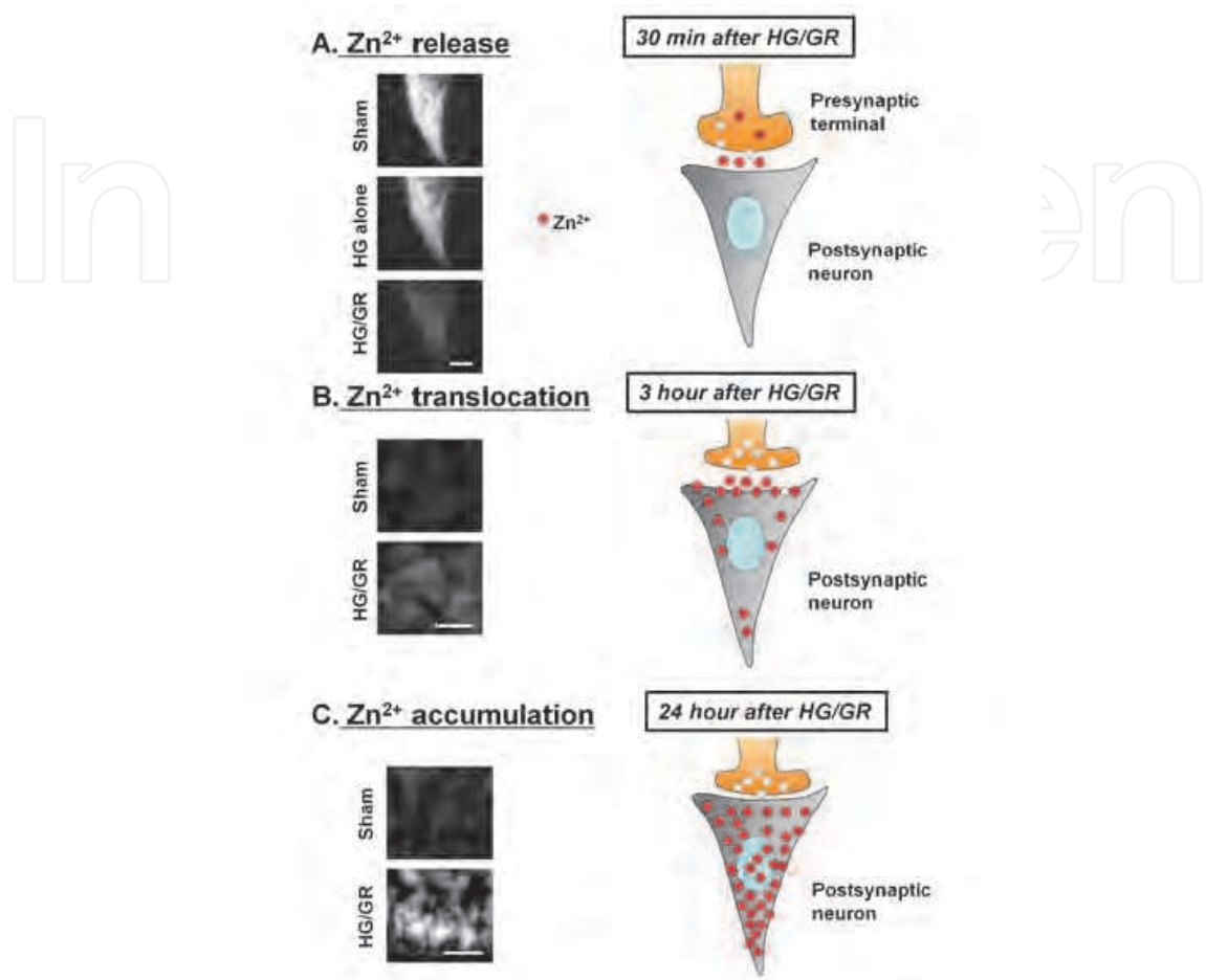
Fig. 1. Vesicular zinc release and translocation after hypoglycemia. A) TSQ fluorescent images show vesicular zinc release from presynaptic terminals of hippocampal mossy fibers after hypoglycemia/ glucose reperfusion (HG/GR). Intense TSQ fluorescent signal (white color in the figure) in the mossy fiber of sham operated rats indicates high vesicular zinc contents in the vesicle. However, the diminished TSQ fluorescent intensity in the HG/GR rats indicates that bulk of vesicular zinc has been released and therefore presynaptic vesicular zinc contents are reduced at the time when the brain section was evaluated. TSQ fluorescent intensity in mossy fiber is decreased after 60 minutes of hypoglycemia (HG alone). TSQ fluorescent intensity is further decreased after 30 minutes hypoglycemia and 30 minutes glucose reperfusion (HG/GR), which represents mossy fiber vesicular zinc release from presynaptic terminals. A schematic drawing represents vesicular zinc release from presynaptic terminals after HG/GR. B) TSQ fluorescent images show zinc translocation into postsynaptic neurons of hippocampal CA1 pyramidal neurons 3 hours after hypoglycemia. Zinc accumulation in the intracellular space can be detected in this early time point. A schematic drawing represents intracellular zinc accumulation 3 hours after HG/GR. C) TSQ fluorescent images show zinc accumulation into postsynaptic neurons 24 hours after HG/GR. Intense zinc accumulation in the intracellular space is detected in this time point. A schematic drawing represents intracellular zinc accumulation 24 hours after HG/GR. Scale bar in (A) is 200 \mu m and in (B) and (C) are 20 \mu m.
