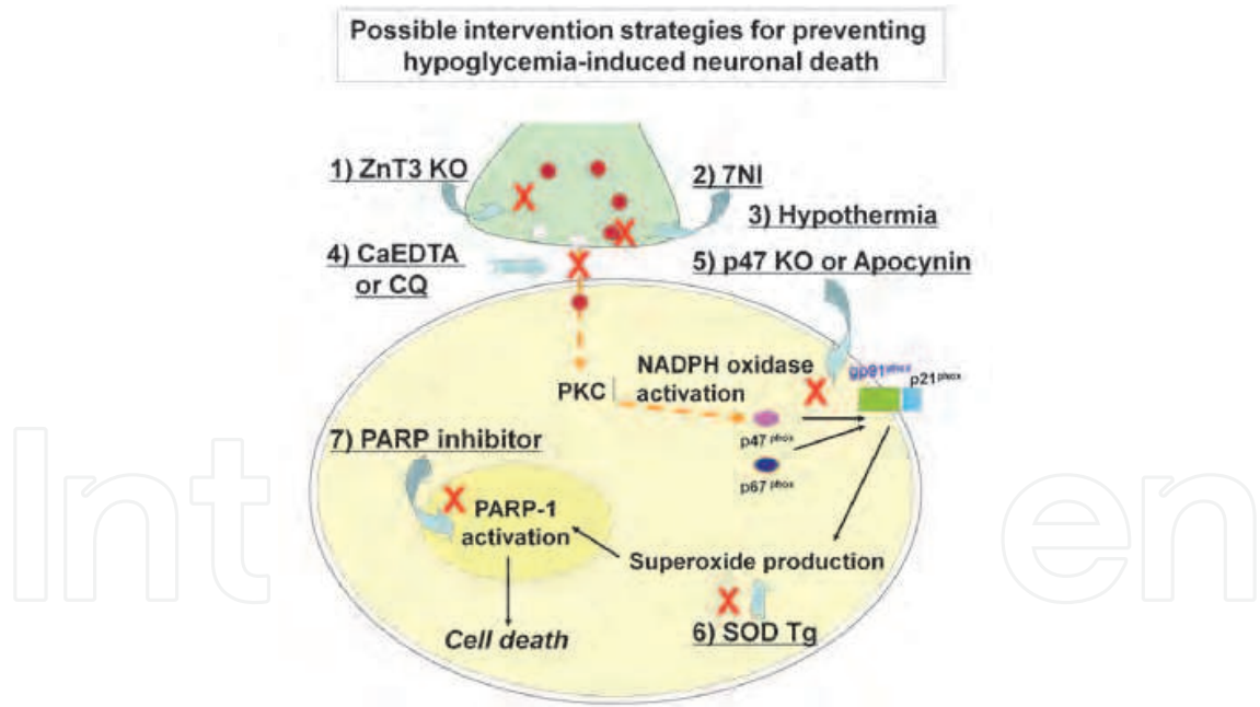
Fig. 9. Proposed intervention strategies for preventing hypoglycemia/ glucose reperfusion-induced neuron death. This schematic drawing indicates that hypoglycemia/ glucose reperfusion-induced neuron death can be prevented by several intervention methods. 1) Vesicular zinc content modulation by gene or chemical manipulation. 2) Vesicular zinc release inhibition by NO inhibitor. 3) Vesicular zinc release inhibition by hypothermia. 4) Zinc chelation in the extracellular space. 5) Inhibition of NADPH oxidase activation. 6) Scavenging or dismutating of reactive oxygen species. 7) Inhibition of PARP-1 activation. Round red colored dot represents ionic zinc. Symbol X represents intervention.
