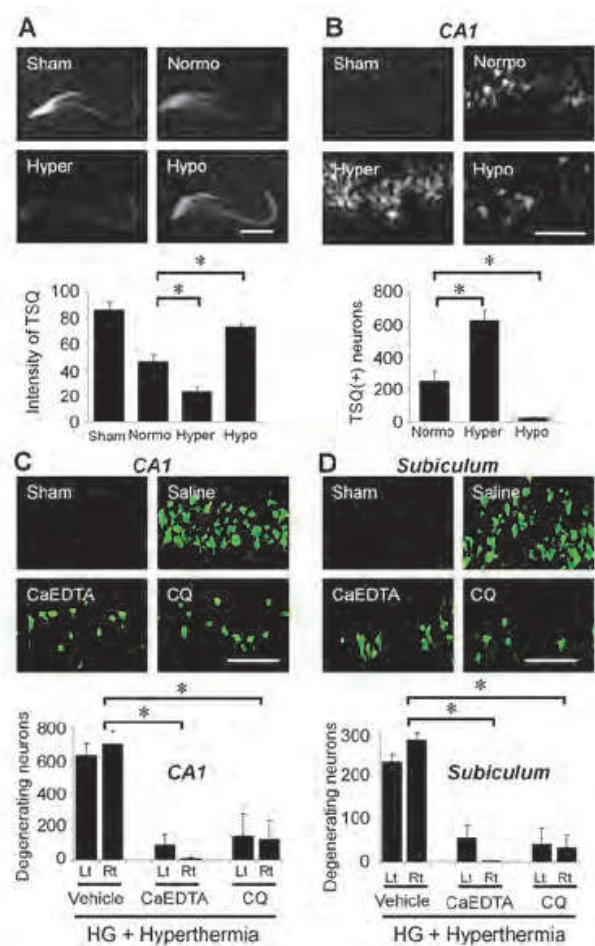
Fig. 8. Temperature dependent hypoglycemic neuronal death is mediated by zinc release and translocation. (A-D) Vesicular zinc release and translocation is aggravated by hyperthermia but is prevented by hypothermia. (A) represents TSQ fluorescence images of hippocampus from sham operated (Sham) and hypoglycemia (HG) experienced rats. Hypothermia group (Hypo) almost completely prevented synaptic zinc release. Scale bar = 500 \mu m. (B) Bar graph shows quantitated TSQ fluorescence intensity from hilus area. Data are mean + s.e.m. (n=7-12). * P < 0.05 compared with normothermic reperfusion group. (C) Photomicrographs of TSQ fluorescence staining shows zinc accumulation in the hippocampal CA1 neurons after hypoglycemia. Scale bar = 100 \mu m. (D) Bar graph shows quantitated TSQ (+) neurons in the CA1 area. Data are mean \pm s.e.m. (n = 5-7). * p < 0.05 compared with normothermic glucose reperfusion group. (E-H) Zinc chelators, CaEDTA or clioquinol (CQ), prevents hypoglycemia-induced neuronal death. (E and G). FJB (+) neurons were reduced by CaEDTA or CQ injection even after hyperthermic reperfusion. Scale bar = 100 \mu m. (F and G) graphs represent quantitated neuronal death in the hippocampal CA1 and subiculum area after hypoglycemia. Data are the mean \pm s.e.m (n=5-7) * p < 0.05 compared with saline treated rats. Part of this figure is modified from our previous published paper (Suh et al., JCBFM, 2010).
