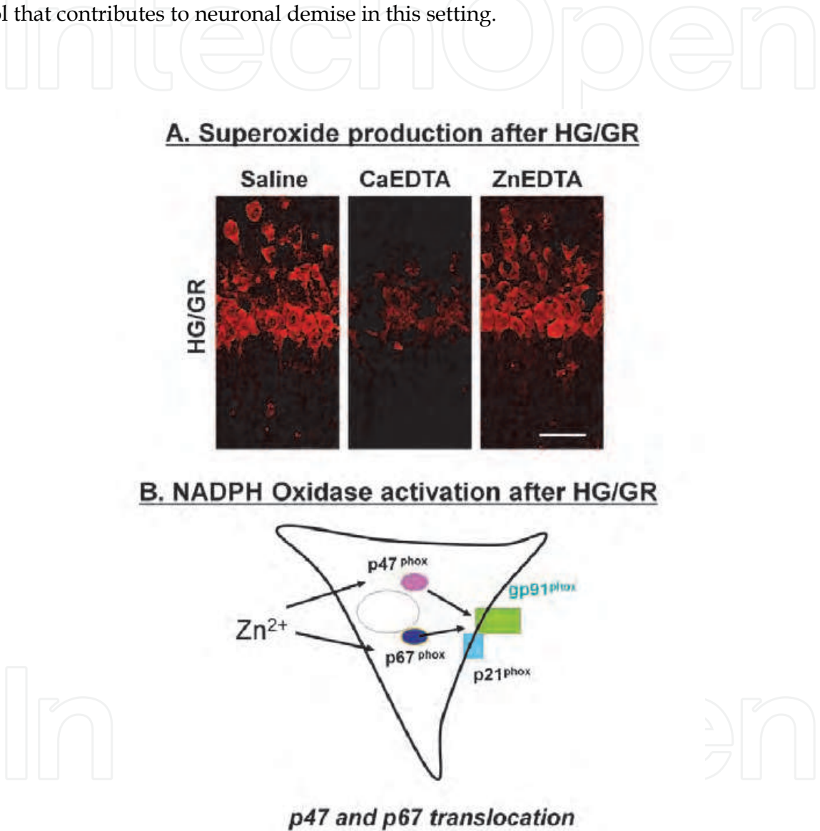
Fig. 4. Hypoglycemia/ glucose reperfusion-induced ROS production is mediated by zinc-induced NADPH oxidase activation. ROS production in neurons detected by ethidium (Et) fluorescence. A) The zinc chelator, CaEDTA, reduces HG/GR-induced Et production in the CA1 neurons. ZnEDTA is the control. Rats were treated with saline, 100 mM CaEDTA, or 100 mM ZnEDTA. Scale bar is 50 \mu m. B) Schematic drawing of p47 phox and p67 phox translocation to plasma membrane by zinc translocation into neuron.
