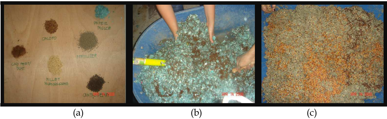
Fig. 3. The hydroseeding components and mixture. (a)Hydroseeding Mix Components(b) Mixing the components(c) Hydroseeding Mixture
