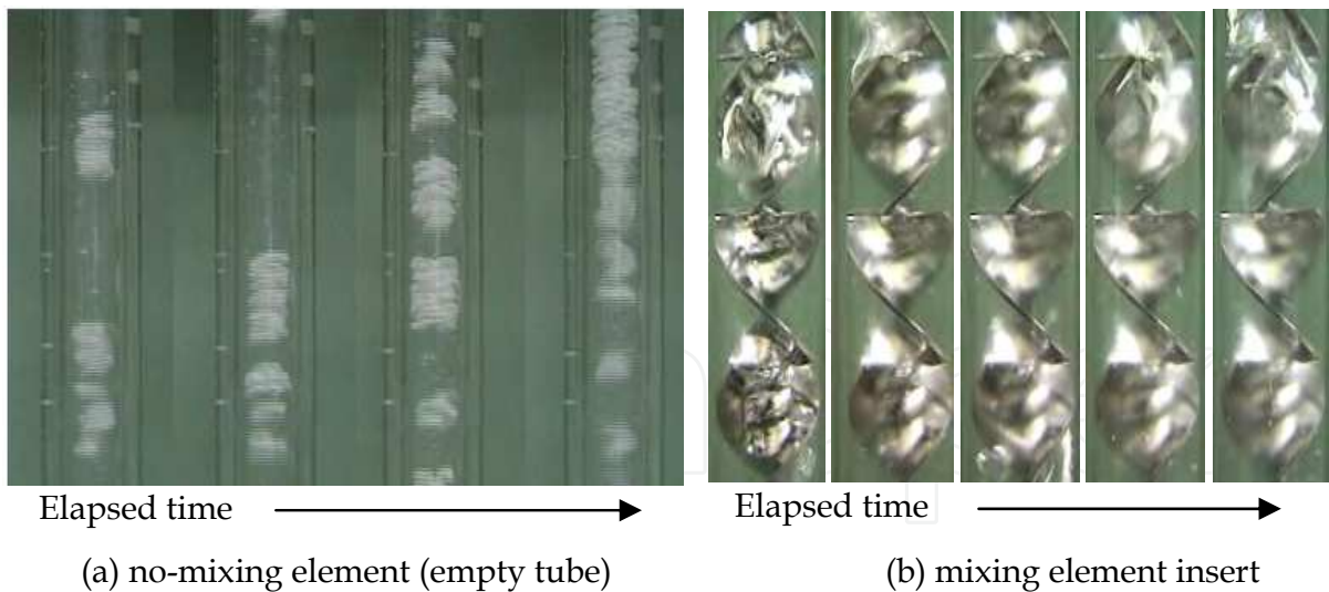
Fig. 2. Static mixing effect on gas hydrate formation from CH 2 FCF 3 gas-water system at 276K and 0.20 MPa with 200 mL/min of gas flow rate)
