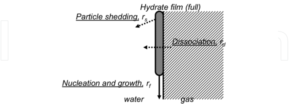
Fig. 9. Speculated mechanisms of hydrate formation in static-mixing type flow reactor (Tajima et al., 2011b)
