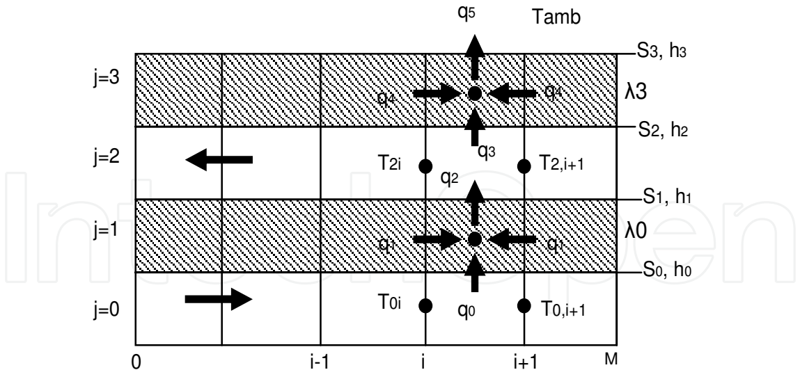
Fig. 18. Real-time model: finite difference scheme.
