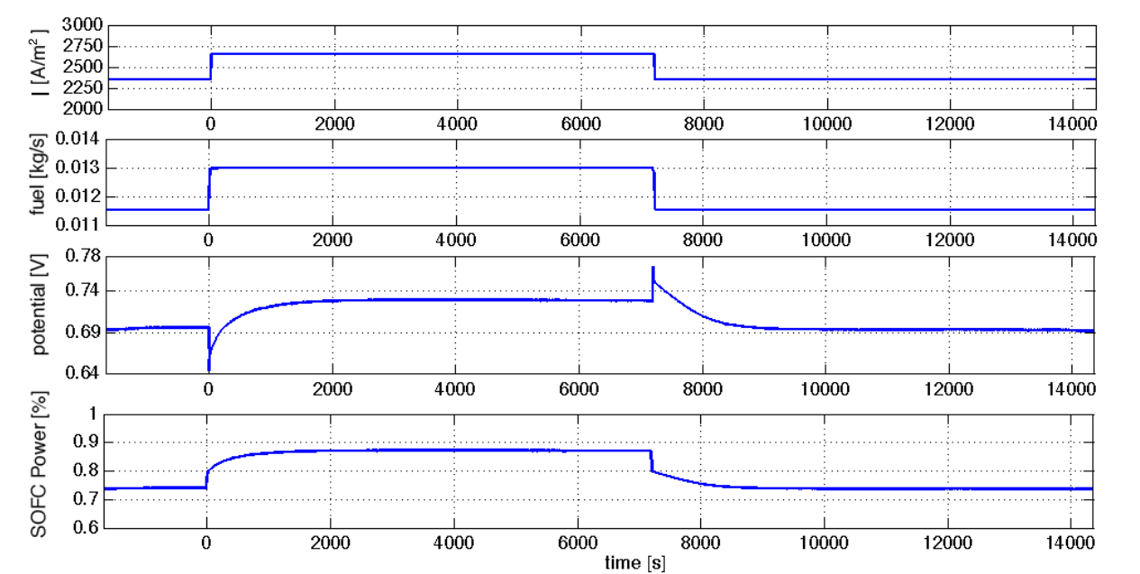
Fig. 12. Emulation test with the real-time model: current density (I), fuel mass flow rate, cell potential, SOFC power (referred to its design value).
