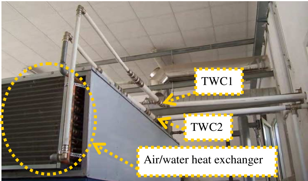
Fig. 14. An air/water heat exchanger with water pipes for compressor inlet temperature control.
