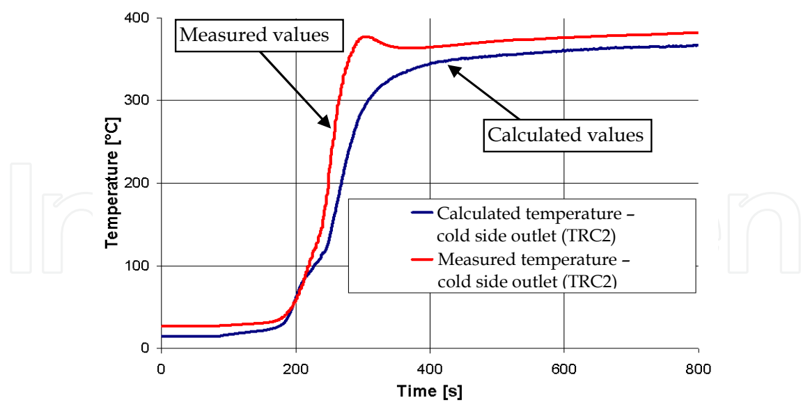
Fig. 19. Recuperator model validation (start-up phase): cold side outlet.
