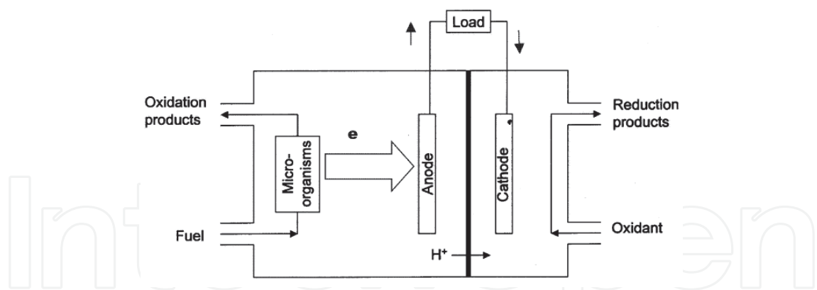
Fig. 1. A typical MFC representing current generation with the help of microorganisms (Shukla et al., 2004)
