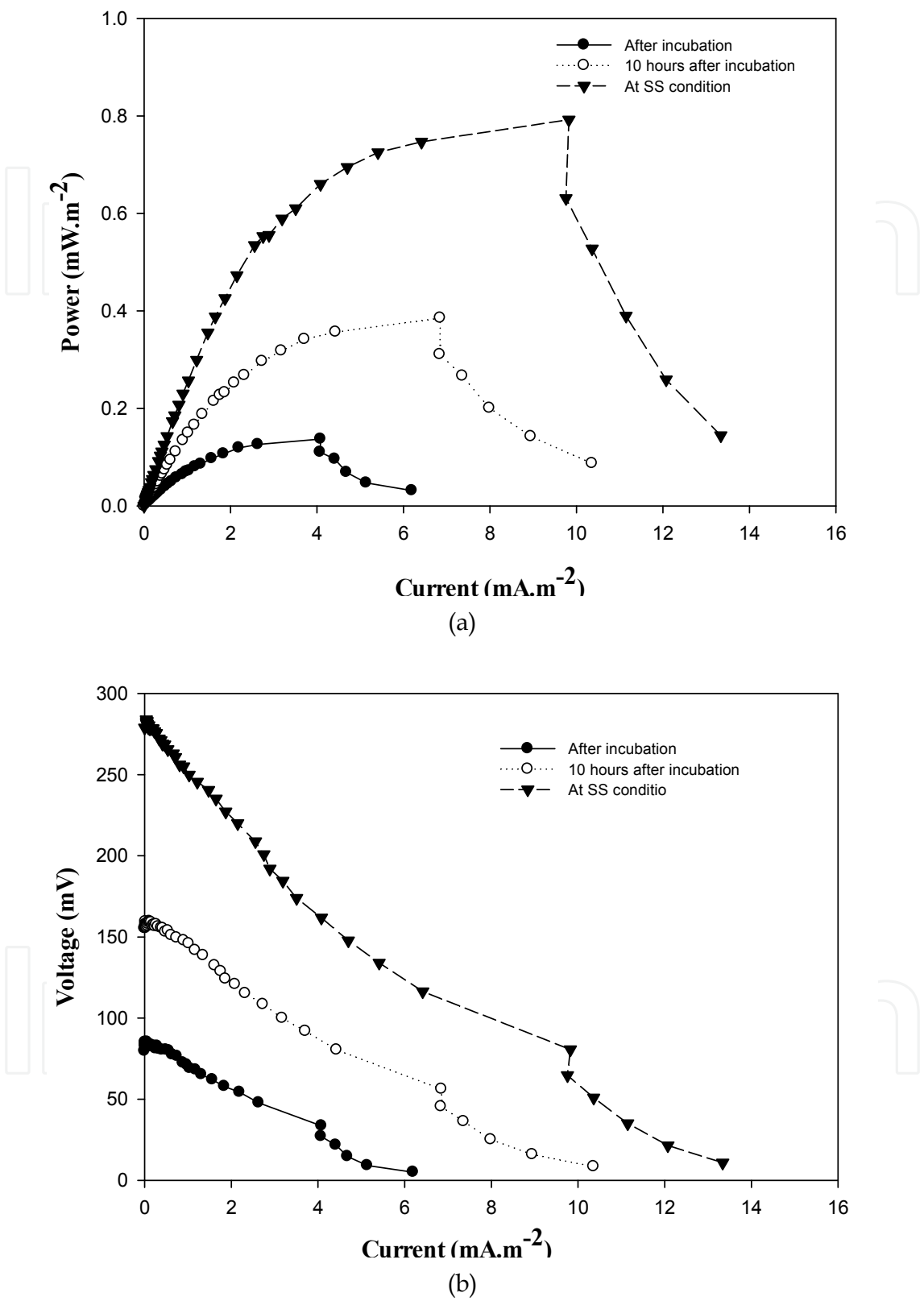
Fig. 3. Generated power density (a) and voltage (b) as function of current density at start up, 10 hours after incubation and at steady state condition
