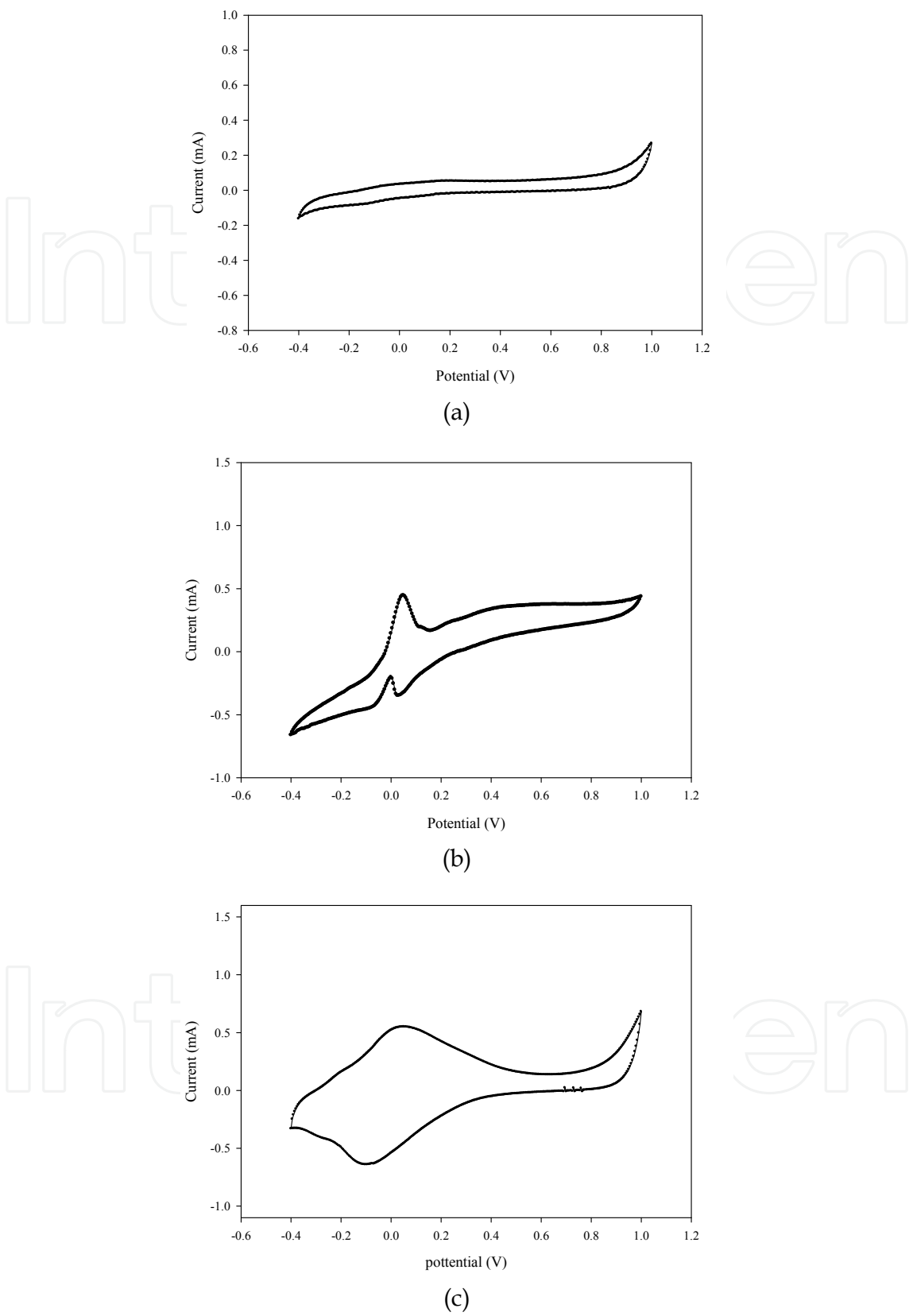
Fig. 7. Effect of active biofilm on anode surface with CV analysis. (a) absence of biofilm ,(b) after formation of biofilm with out mediators and (c) after formation of biofilm with 200 \mu\text{mol.l}^{-1} NR as electron mediators .scan rate was 0.01 V.S -1
