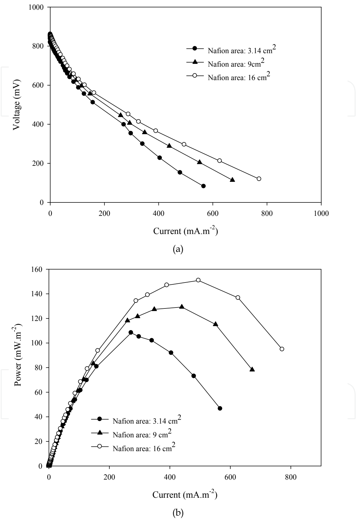
Fig. 5. Effect of mass transfer area on performance of MFC.
