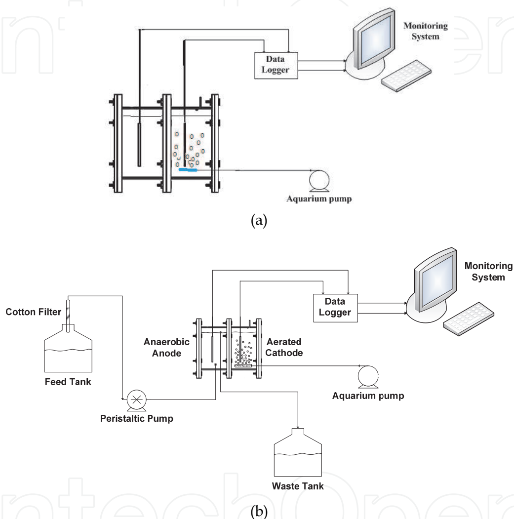
Fig. 2. Schematic diagram of cubic two chamber MFC in batch (a) and continues (b) mode
