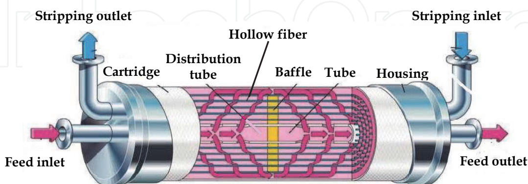
Fig. 1. The hollow fiber module ( http://www.liquicel.com/product-information/gas-transfer.cfm )
