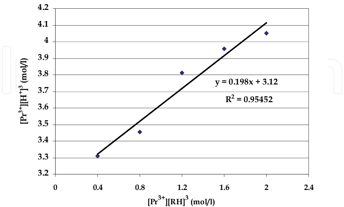
Fig. 7. Extraction of Pr(III) by Cyanex 272 as a function of equilibrium [Pr^{3+}][RH]^3
