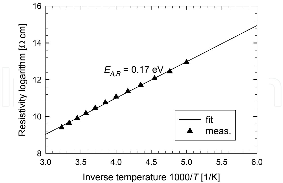
Fig. 5. Arrhenius plot of the van der Pauw measurement conducted on the annealed CZTSSe tablet. E_{A,R} is the extracted activation energy. T is temperature in Kelvin.
