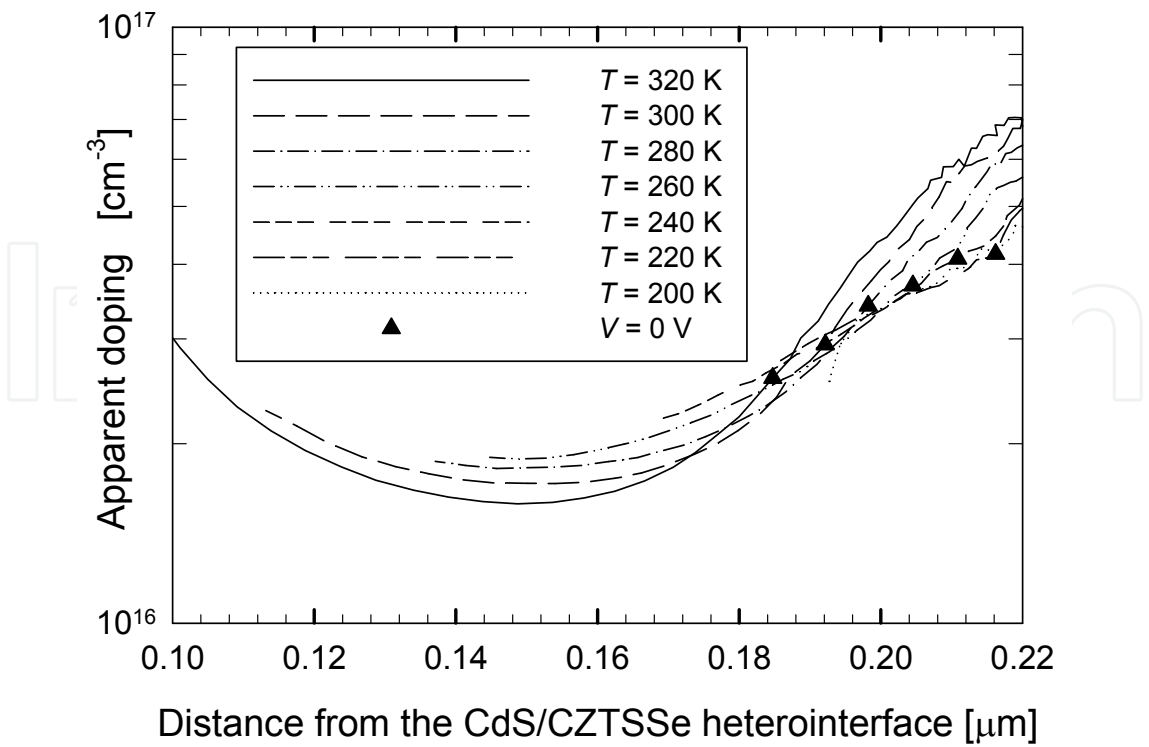
Fig. 4. The apparent doping density p_{SCR} obtained from the bias voltage derivative of the Mott-Schottky plot. The distance from the junction is calculated from the space charge region capacitance. Triangles depict the 0 V bias conditions.
