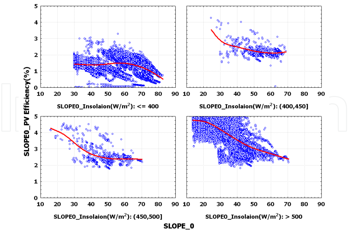
Fig. 26. PV module power efficiency vs. solar incidence angle (SLOPE_0°)
