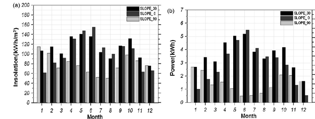
Fig. 8. Monitoring data of PV module depending upon the slope through the mockup model: monthly accumulated data of (a) solar irradiance and (b) power output.
