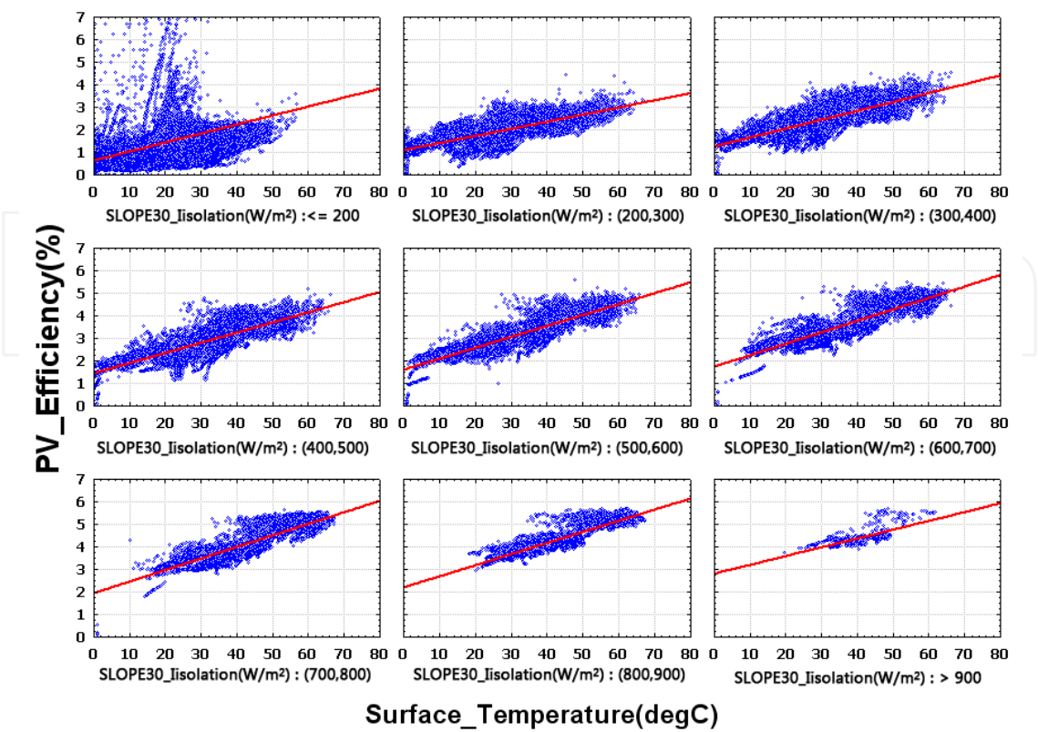
Fig. 22. Correlation between the surface temperature and power efficiency (SLOPE_30°)
