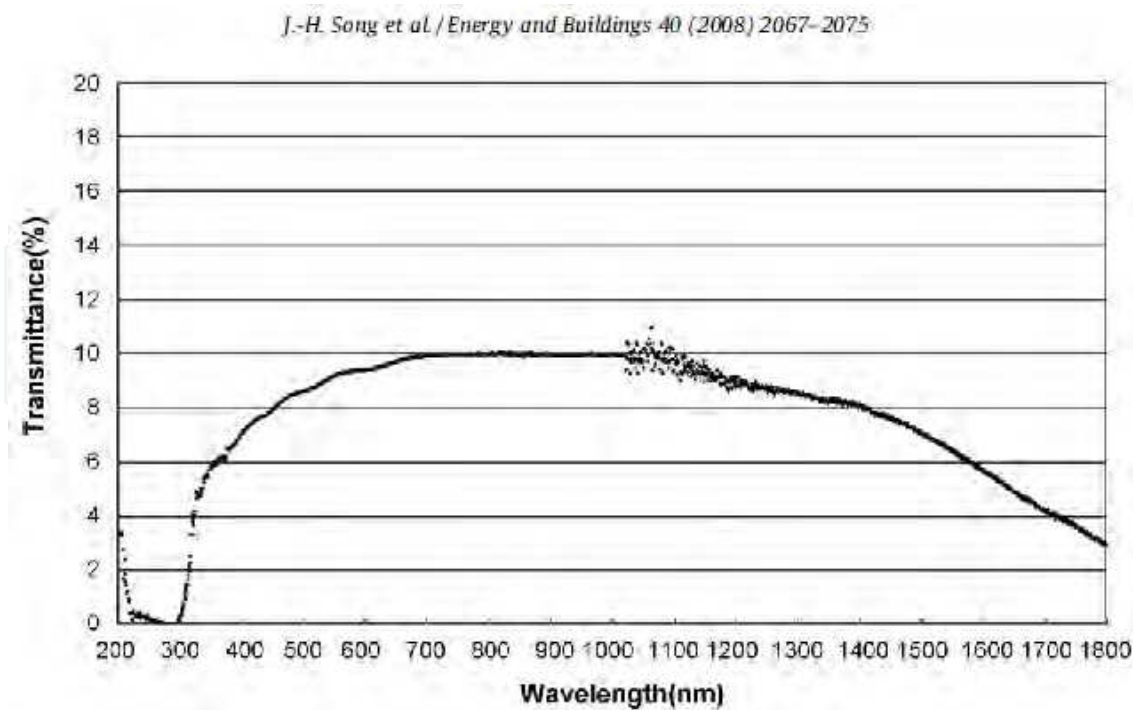
Fig. 1. Transmittance of PV module depending on the wavelength
