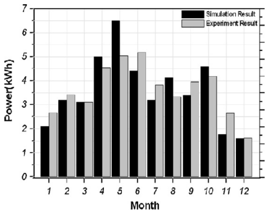
Fig. 14. Power output data calibration by comparing the experimental data to the computed data obtained from the simulation program (TRNSYS).
