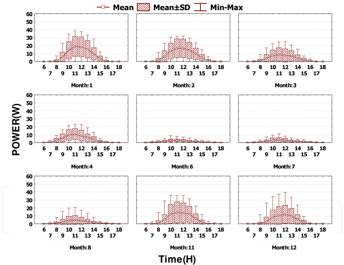
Fig. 10. Power generation of SLOPE 90° in each timestep
