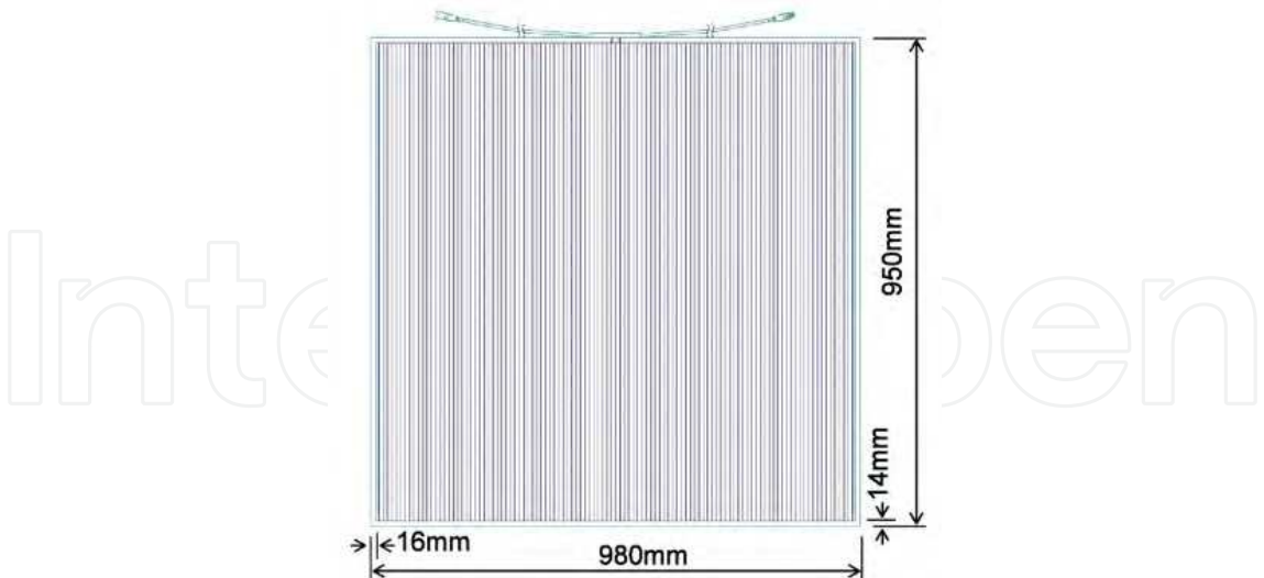
Fig. 4. Plane figure of a single plate PV module.
