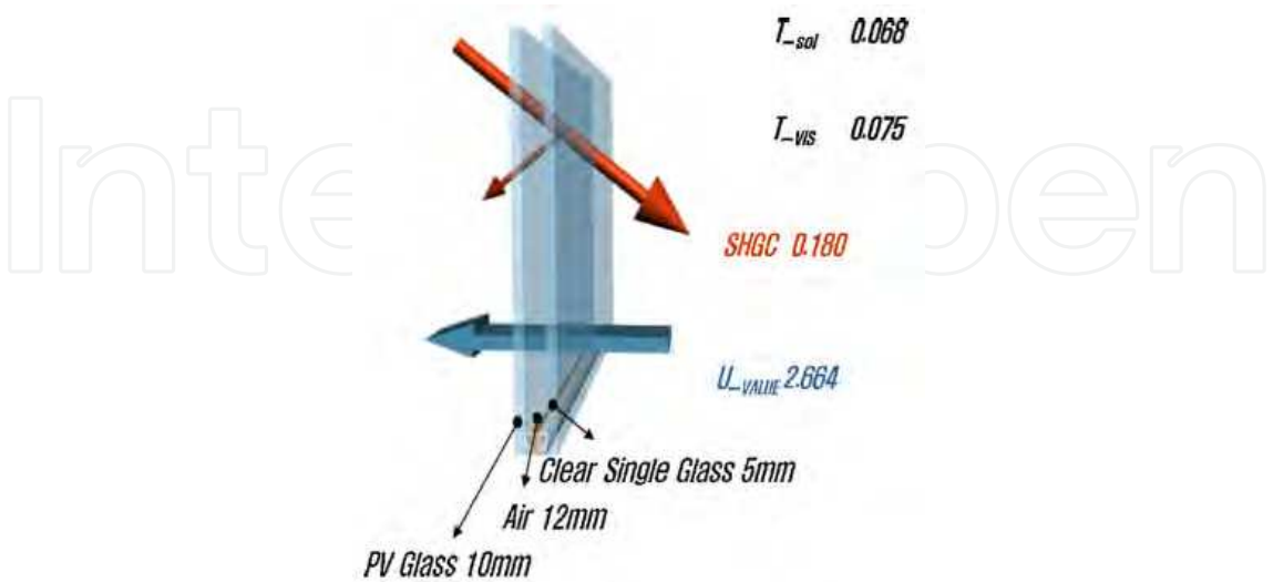
Fig. 3. Optical and thermal characteristics of double-glazed PV module ( T_{sol} is the solar transmittance, T_{vis} is the transmittance of visible radiation, SHGC is the solar heat gain coefficient, and U_value is the thermal transmittance of PV module).module
