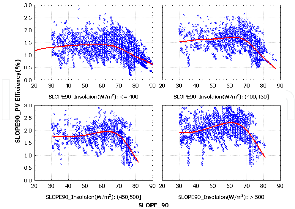
Fig. 24. PV module power efficiency vs. solar incidence angle (SLOPE_90°)
