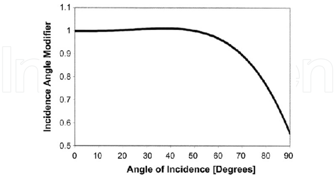
Fig. 18. Correlation of incidence angle modifier given by King et al. (1994).
