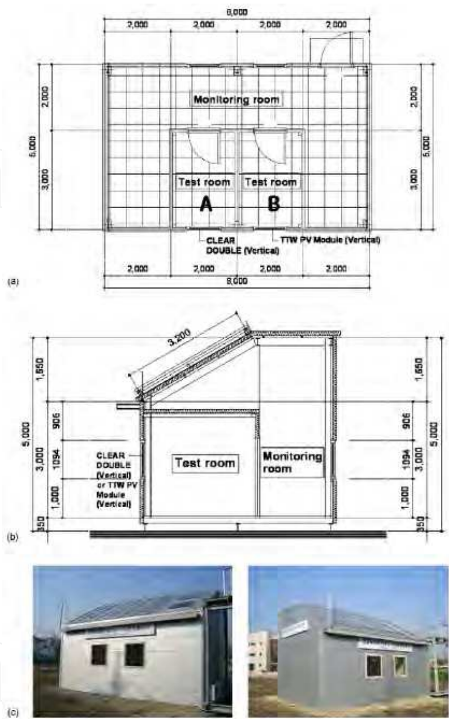
Fig. 5. Full-scale mock-up model: (a) a floor plan view, (b) a cross-sectional view, and (c) photographs of mock-up model.
