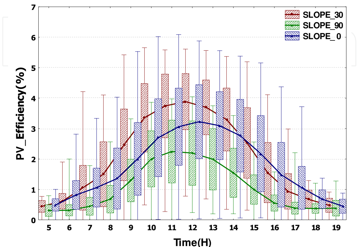
Fig. 19. Annual hourly averaged power efficiency
