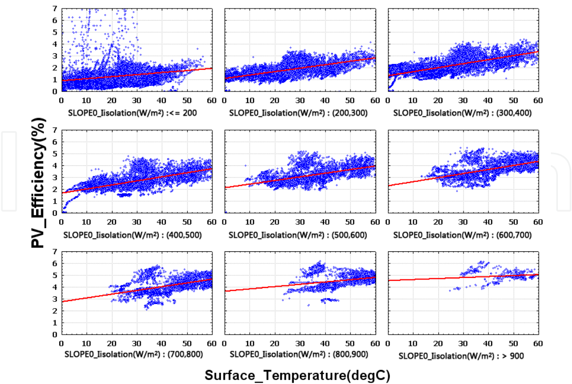
Fig. 23. Correlation between the surface temperature and power efficiency (SLOPE_0°)
