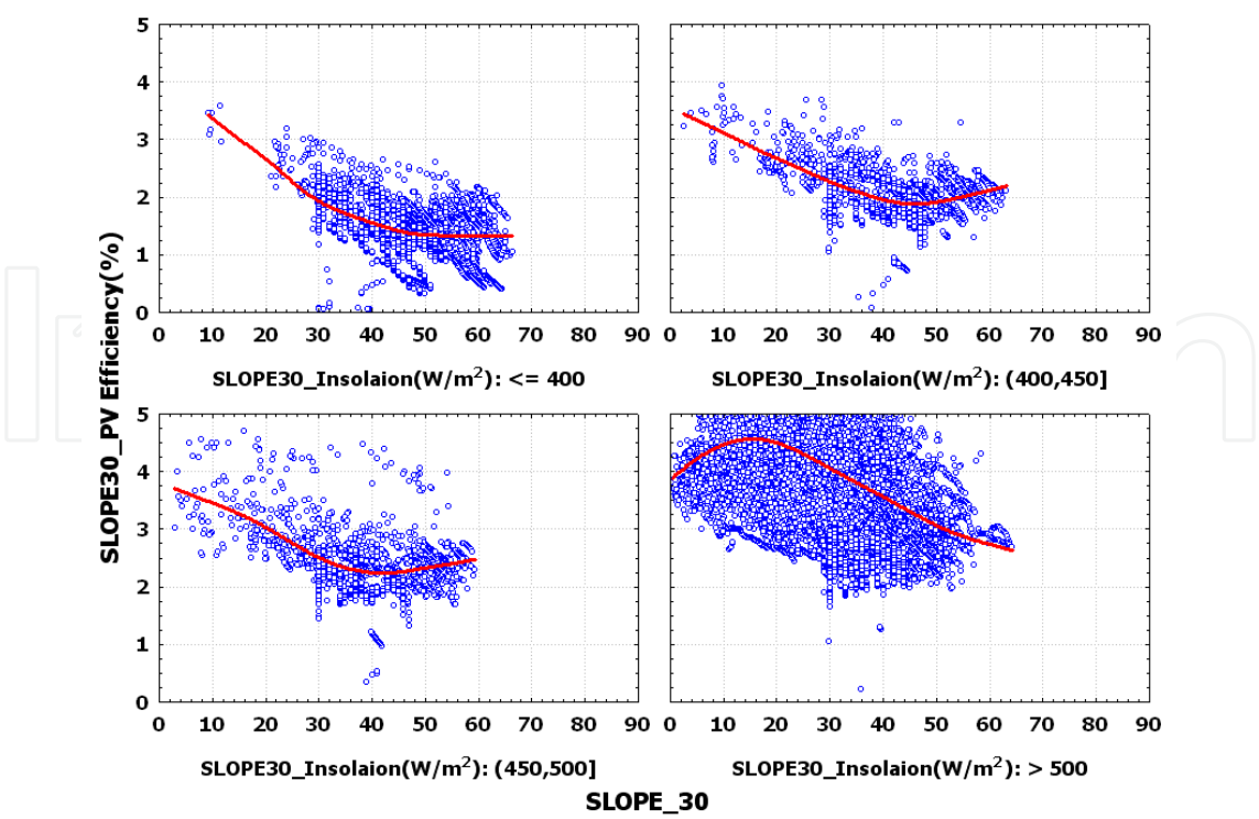
Fig. 25. PV module power efficiency vs. solar incidence angle (SLOPE_30°)
