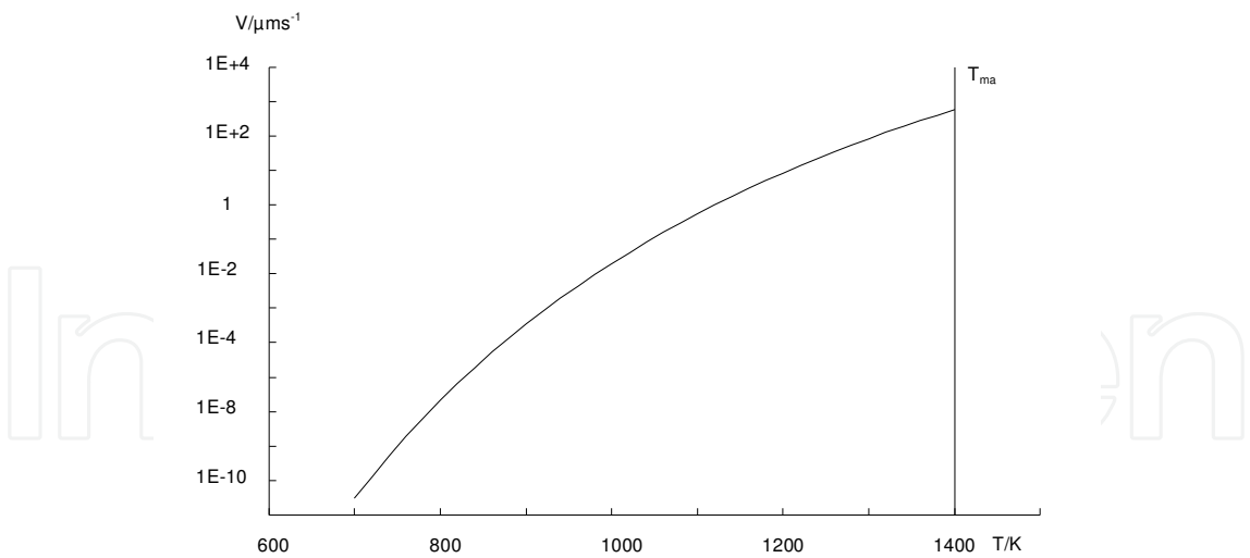
Fig. 7. Speed of a crystallization front in amorphous silicon as depending on temperature
