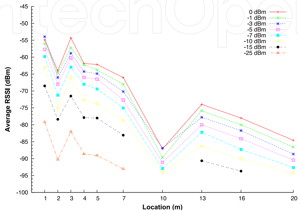
Fig. 2. Effects of sensor locations on RSSI
