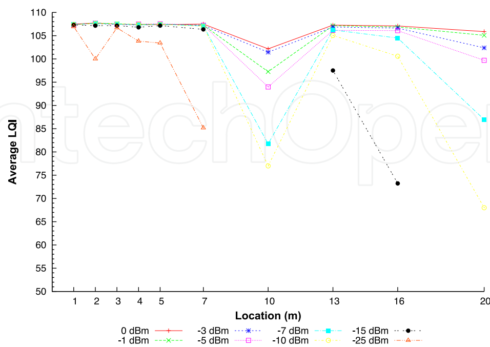
Fig. 3. Effects of sensor locations on LQI
