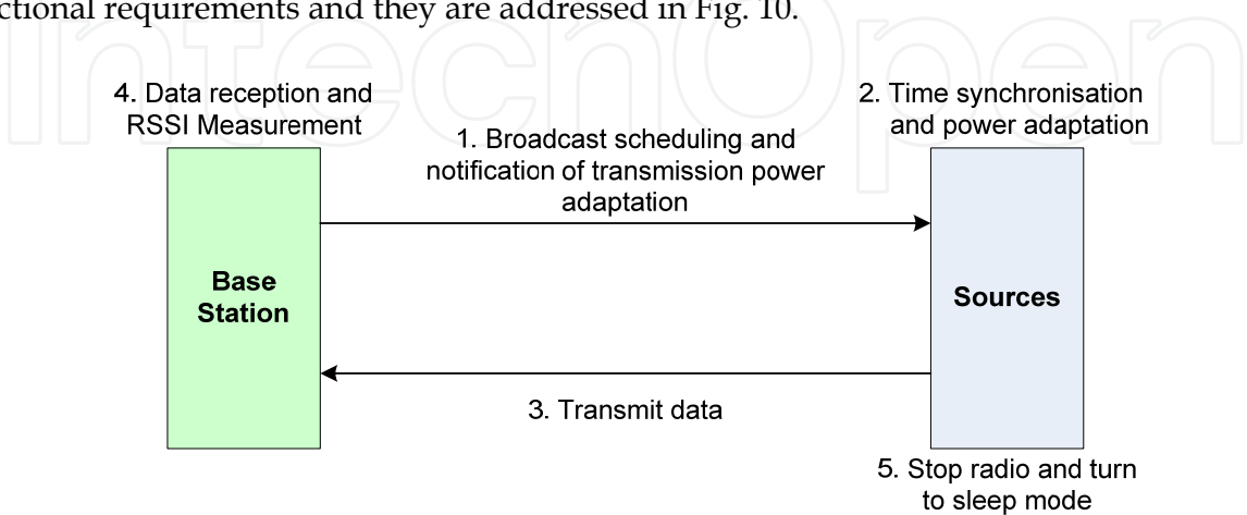
Fig. 10. Interaction between sources and base station
