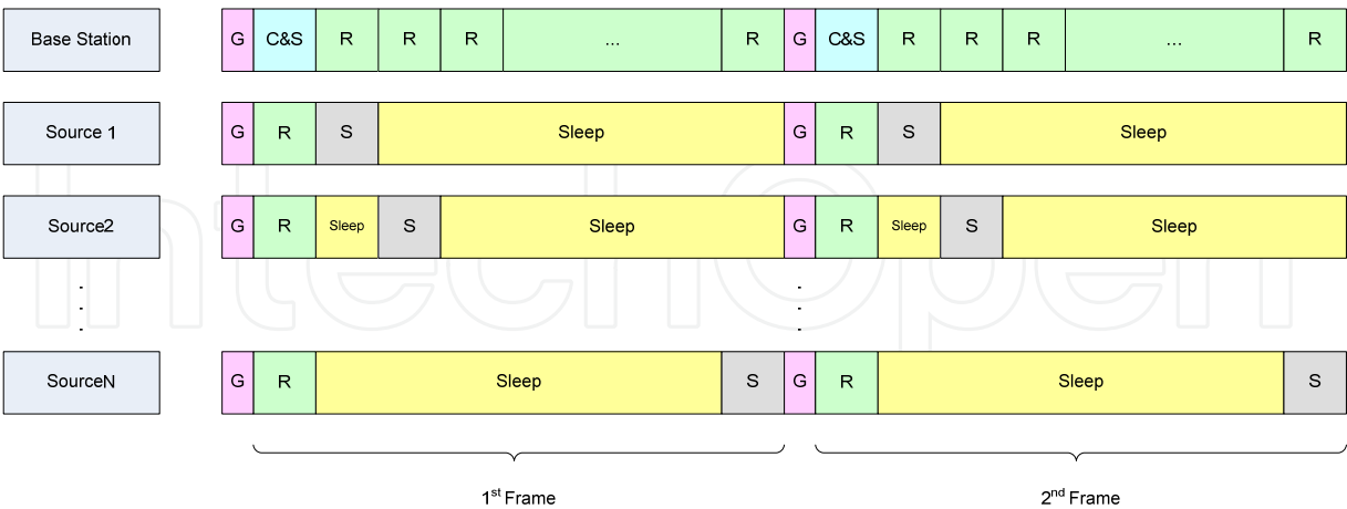
Fig. 15. Mode switching during the data delivery phase
