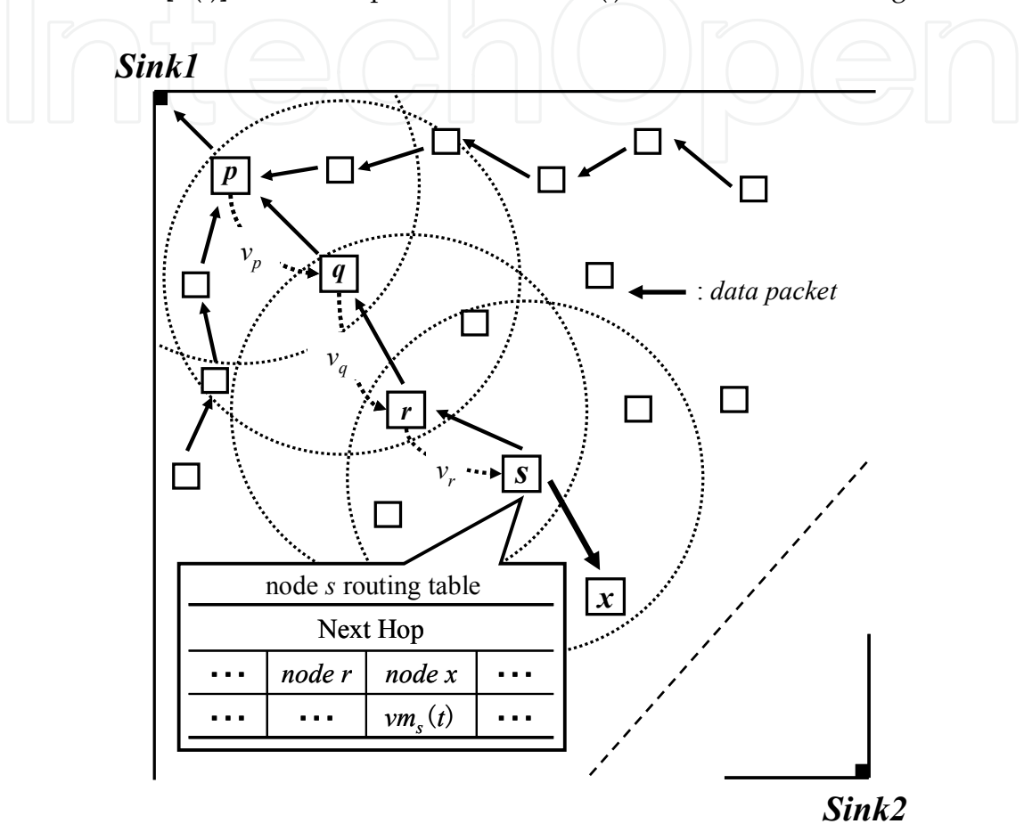
Fig. 2. An example of autonomous load-balancing data transmission to multiple sinks Our scheme (Matsumoto et al., 2010) requires the construction of a data gathering environment in the initial state of a large scale and dense wireless sensor network with multiple sinks, but needs no special communication for network control. The above-mentioned simple mechanism alone achieves autonomously adaptive load-balancing data transmission to multiple sinks, as in Fig.2. The lifetime of a wireless sensor network can be extended by reducing the communication load for network control and solving the node load concentration problem.
