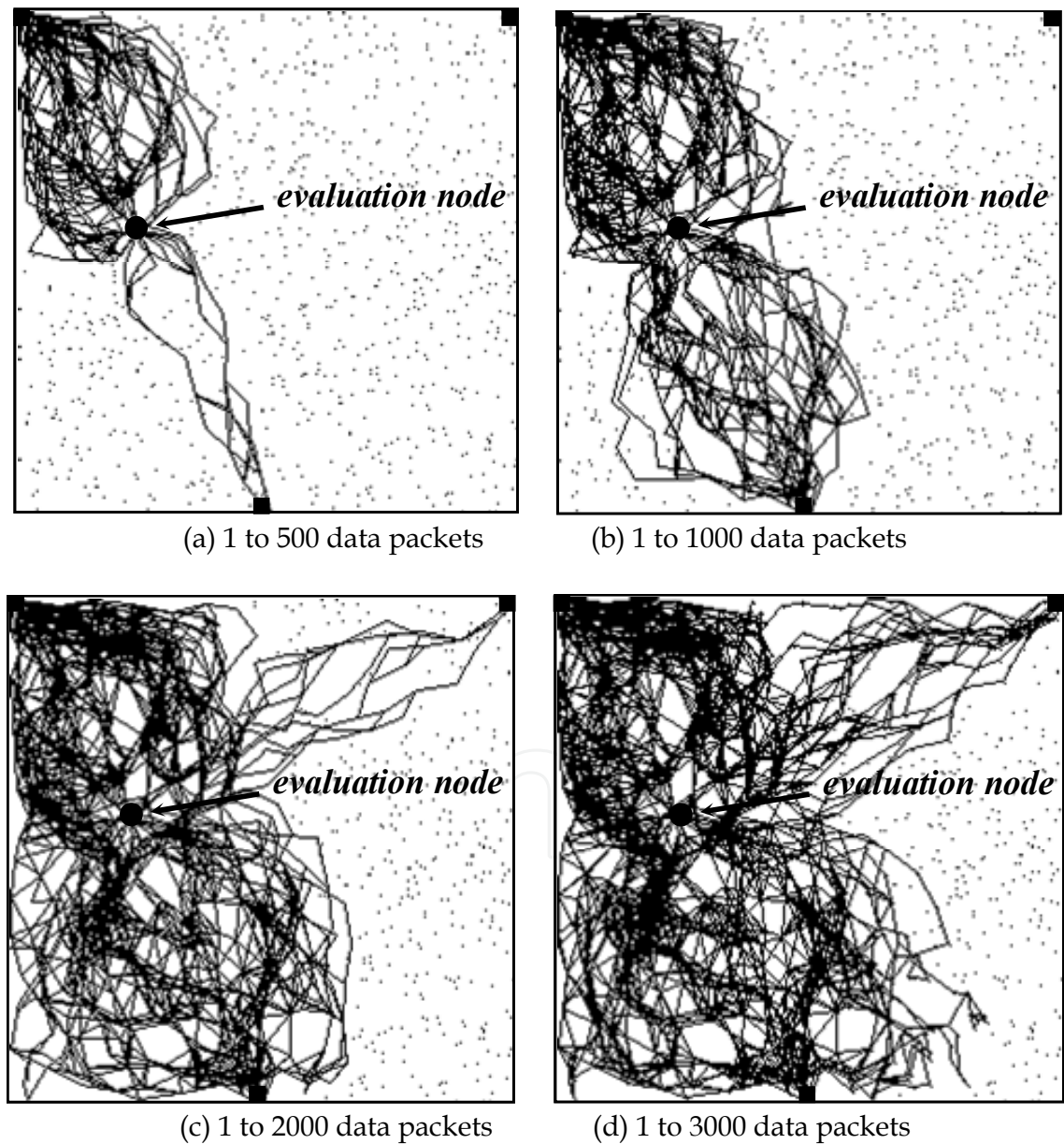
Fig. 9. Routes used by applying our scheme ( T_e = E \times 0.9J )
