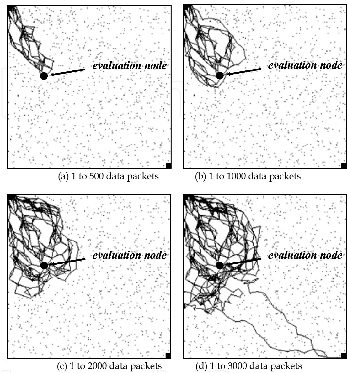
Fig. 5. Routes used by applying our scheme to the simulation model with two sinks
