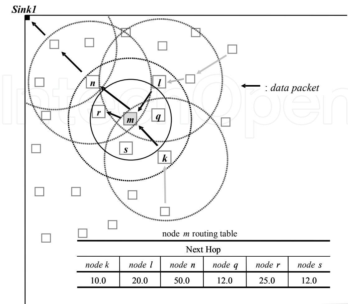
Fig. 3. An example of transmission power control
