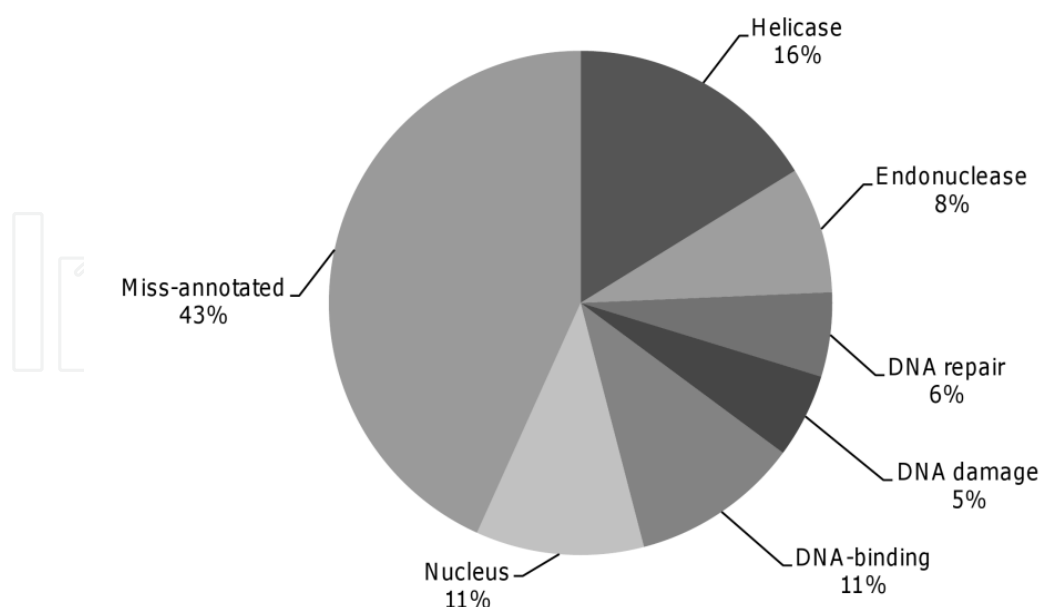
Fig. 2. Functional categorizations of E. histolytica DNA repair genes. Biological processes and molecular functions were determined using David software ( http://david.abcc.ncifcrf.gov/gene2gene.jsp ). Percentage of genes included in individual categories is given.
