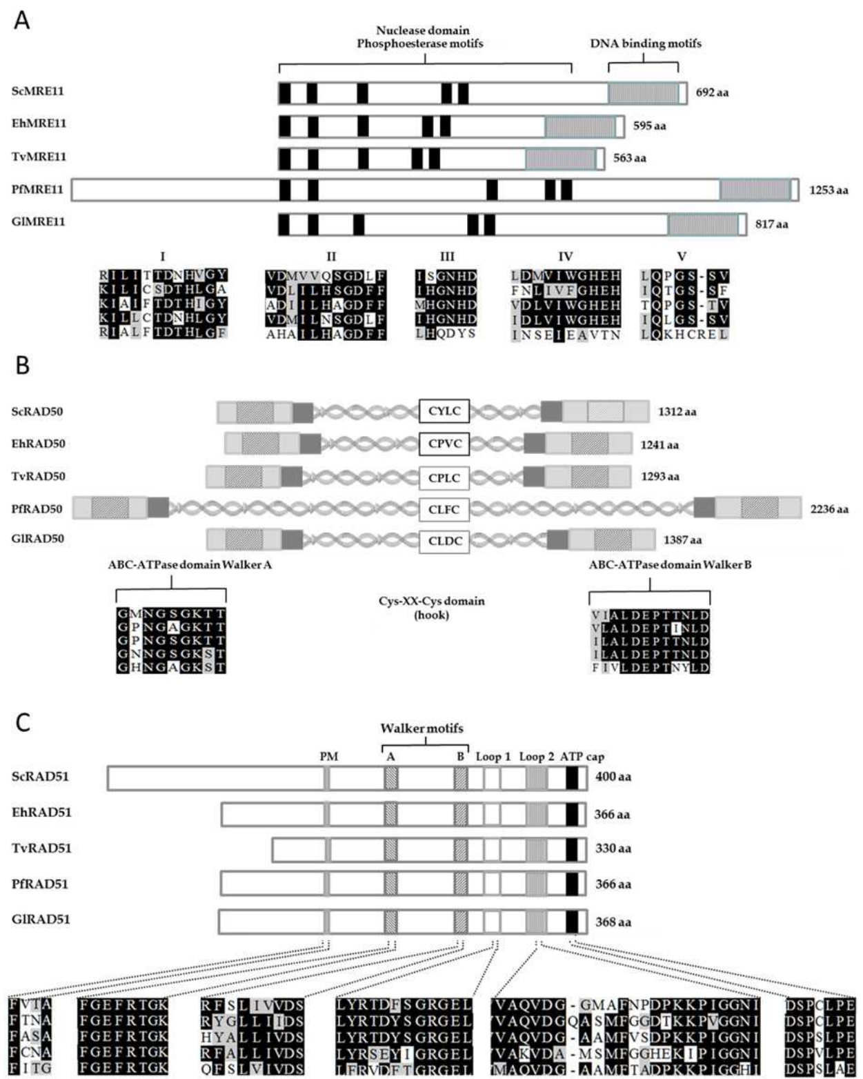
Fig. 5. Comparison of the amino acids sequence of MRE11, RAD50 and RAD51 proteins of S. cerevisiae E. histolytica , T. vaginalis , P. falciparum and G. lamblia . (A). Functional and structural domains of MRE11 proteins. MRE11 phosphoesterase motifs I-V (black
