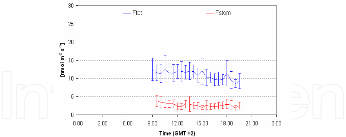
Fig. 6. Mean daily course of the absolute values of total and stomatal ozone fluxes in the second period F_{\text{tot}} (blue line) and F_{\text{stom}} (red line) are the total and the stomatal ozone fluxes when the canopy were completely dry, i.e. excluding the periods where dew was found on the leaves. Vertical bars are the standard deviations.
