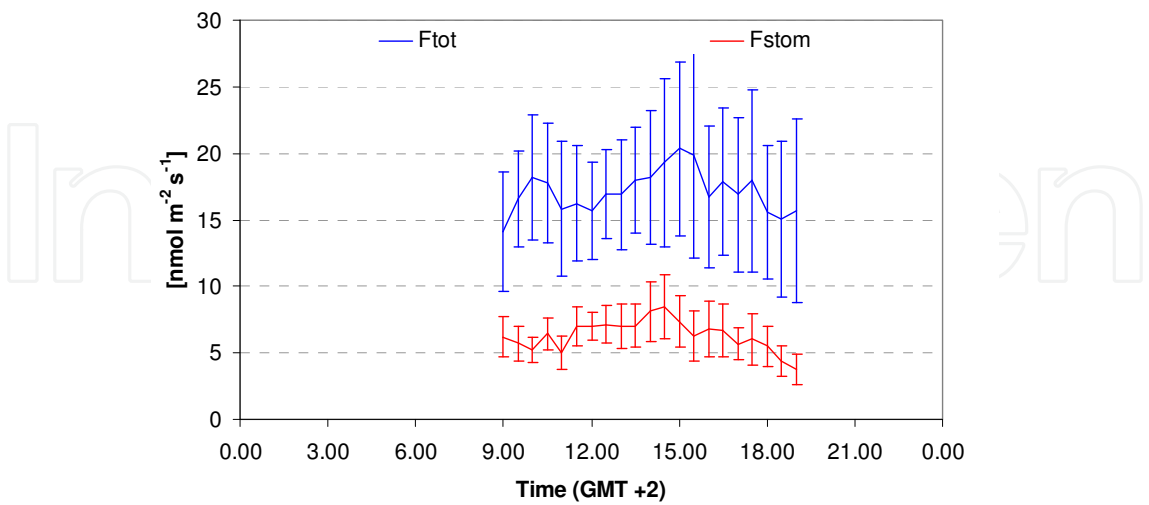
Fig. 5. Mean daily course of the absolute values of total and stomatal ozone fluxes in the first period F_{\text{tot}} (blue line) and F_{\text{stom}} (red line) are the total and the stomatal ozone fluxes when the canopy were completely dry, i.e. excluding the periods where dew was found on the leaves. Vertical bars are the standard deviations.
