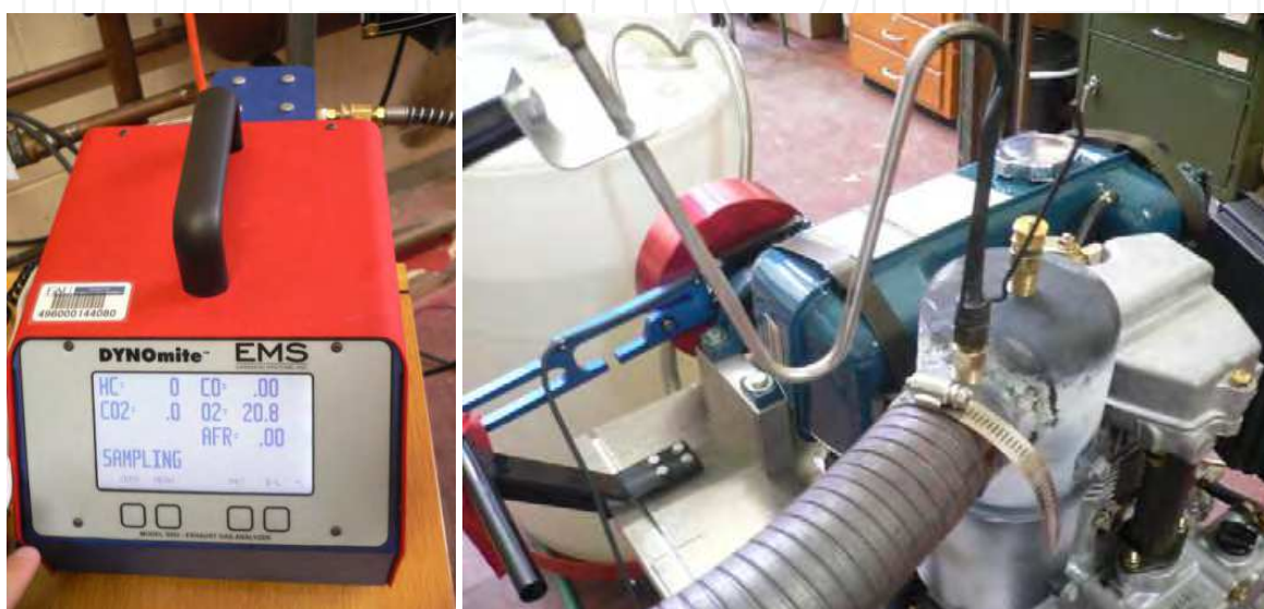
Fig. 9. Gas Analyser and emission probe
