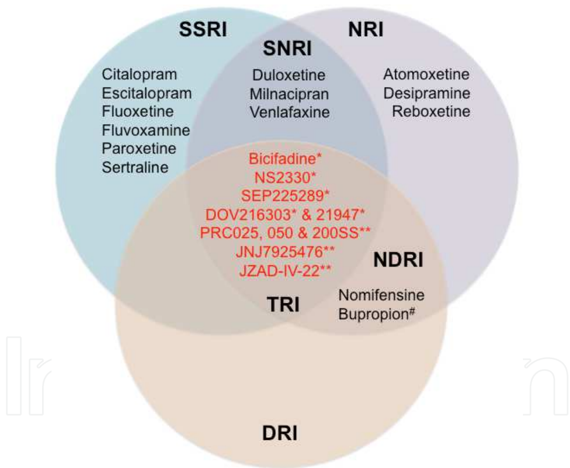
Fig. 2. Monoaminergic antidepressants blocking the serotonin, norepinephrine and/or dopamine transporter. These agents are in various clinical* or preclinical** phases of development in MD or comorbidities. Selective serotonin reuptake inhibitor (SSRI), norepinephrine reuptake inhibitor (NRI), dopamine reuptake inhibitor (DRI), serotonin/norepinephrine reuptake inhibitor (SNRI), norepinephrine/dopamine reuptake inhibitor (NDRI), triple reuptake inhibitor (TRI). #This agent is a dopamine reuptake inhibitor and a norepinephrine releaser (Dong and Blier, 2001).
