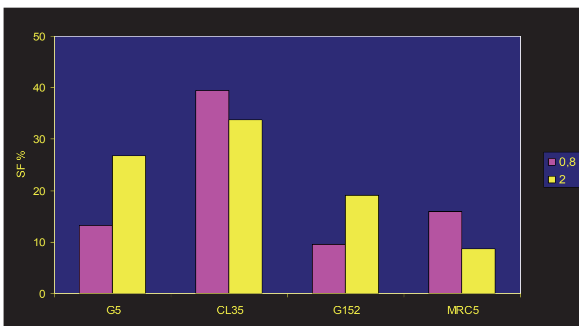
Fig. 3. Survival of human glioma cells following repeated irradiations. G5, CL35, G152 or MRC5 cells were exposed to 0.8 Gy 3 times/day spaced by 4 hr for 2 consecutive days or to 2 Gy once/day for 2 consecutive days. Cell survival was assessed by a clonogenic assay.
