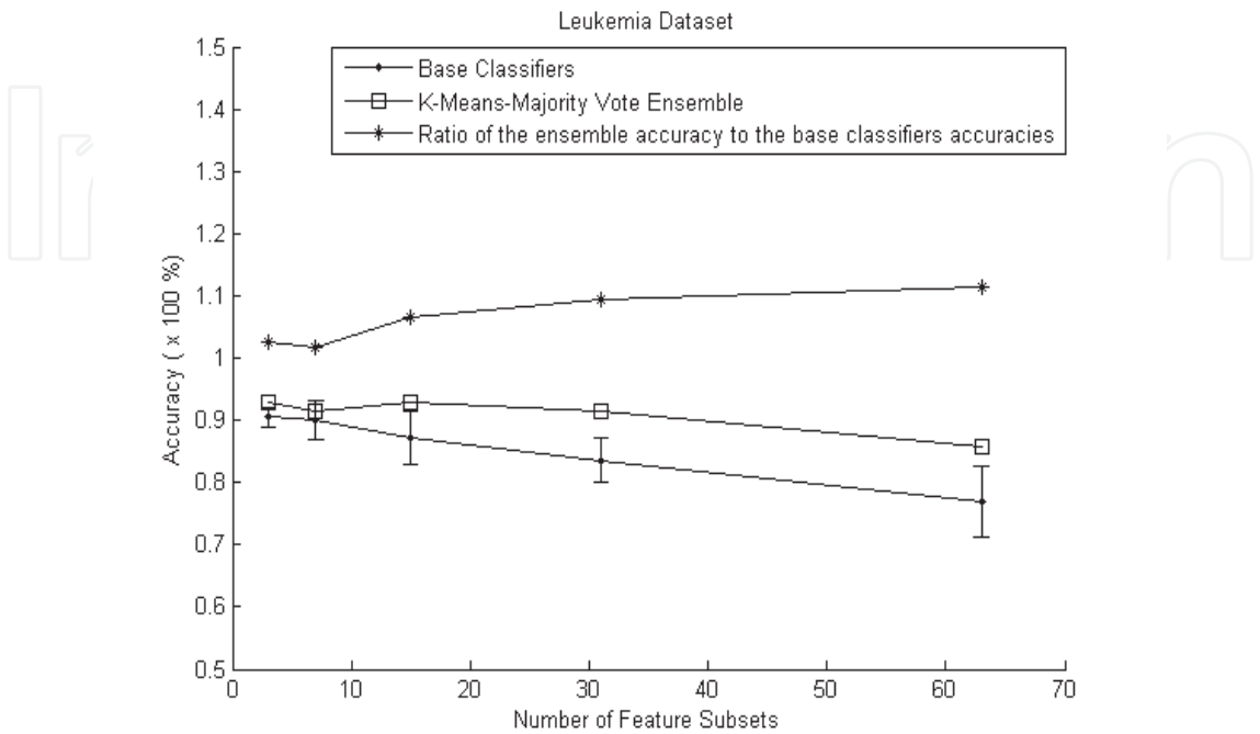
Fig. 7. Results of the k-means-majority vote ensemble.
