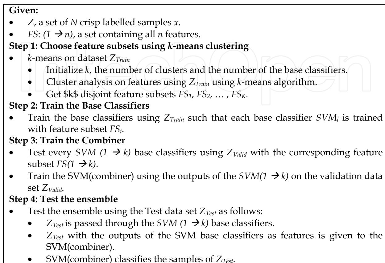
Fig. 5. Ensembles using SVM fusion.
