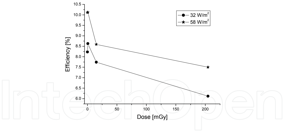
Fig. 15. Dependence of the efficiency on doses (Vasic et al., 2008).
