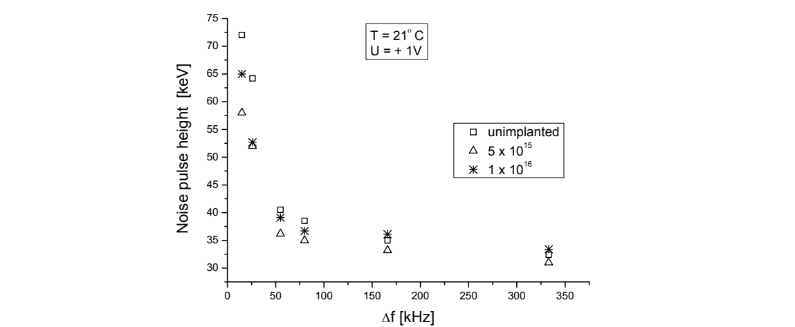
Fig. 2. Frequency noise level for TiN/Ti/Si samples at 21°C (Vasic et al., 2011).
