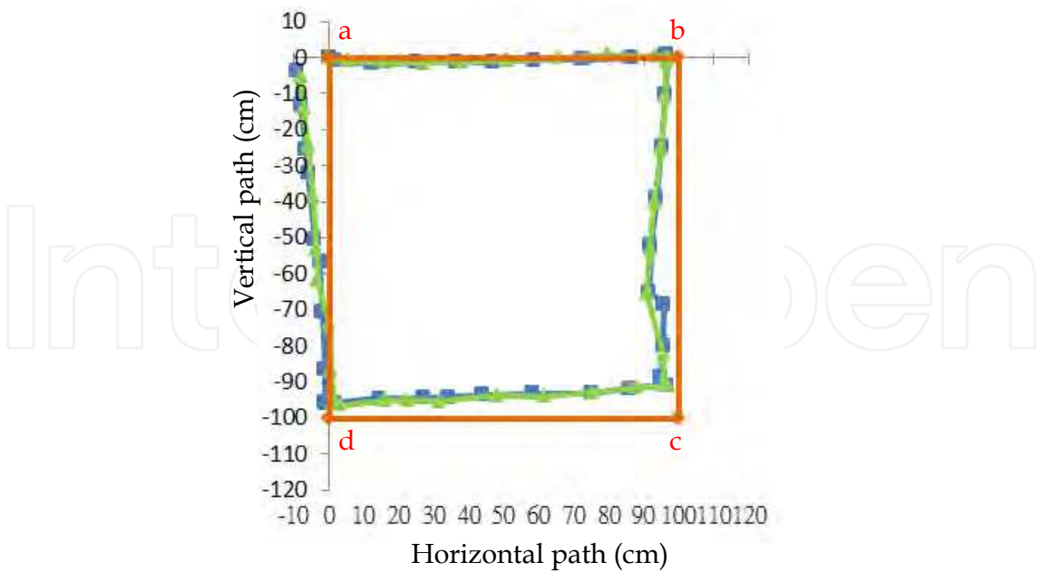
Fig. 20. Rectangular path error without the guidance of the localization system.
