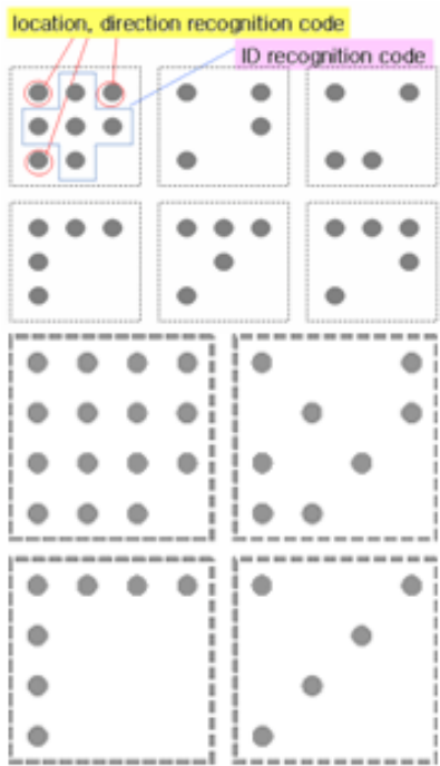
Fig. 12. IR passive landmark (Hagisonic co.)
