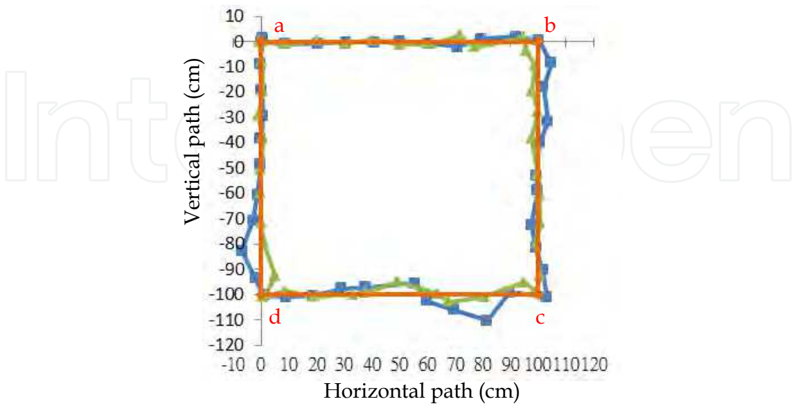
Fig. 21. Rectangular path error with the guidance of the localization system.
