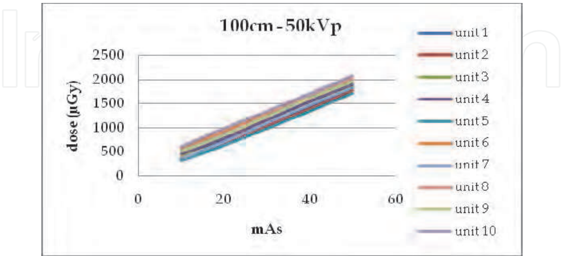
Fig. 8. Measured dose values of 10 x-ray units versus mAs for 50kVp at distance of 100cm.
