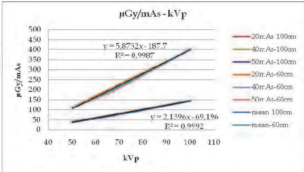
Fig. 16. X-ray tube output changes with kVp (dose values from procedure in Section 3.2). The tube output which is derived from direct measurement can be expressed in equations obtained from Figure 15 and Figure 16, because kVp is related to tube output directly. For distance of 100cm, tube output can be written separately in different two equations that were obtained from graphics in Fig. 15 and Fig. 16.
