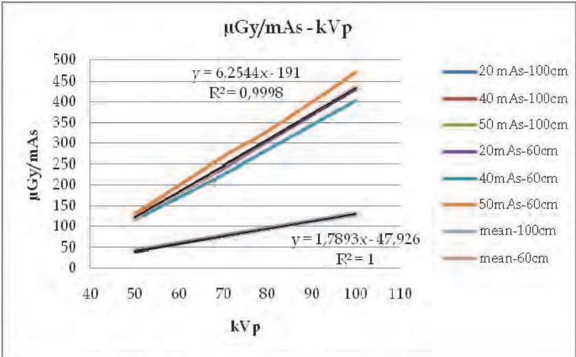
Fig. 15. X-ray tube output changes with kVp (dose values from procedure in Section 3.1).
