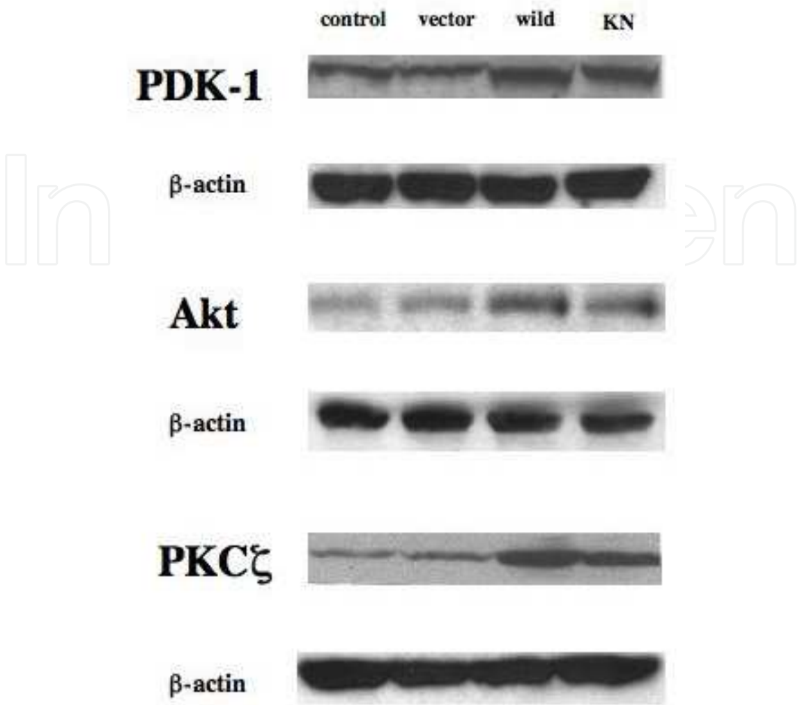
Fig. 1. Overexpression of PDK1, PKCζ and Akt in rat adipocytes. Isolated rat adipocytes were prepared as described in “Materials and Methods”. Adipocytes (50%) were transfected by the electroporation method (5 μg/cuvette) in the presence or absence (control) of eucariocytes expression vector-containing wild and kinase-inactive (KN) cDNA encoding PDK-1, Akt and PKCζ. Transfected adipocytes were incubated at 37°C overnight in Dulbecco’s modified buffer. Each protein was identified by ECL western blotting system as shown in “Materials and Methods”. Equal loading of protein was confirmed by stripping the membrane and staining with anti-β-actin antibody. Transfection with wild type and kinase-negative type (KN) PDK1/PKCζ/ Akt significantly increased immunoreactive PDK1/PKCζ/ Akt 2-3 fold compared with nontransfected cells, respectively. Statistical significance was determined by Fisher’s PLSD test.
