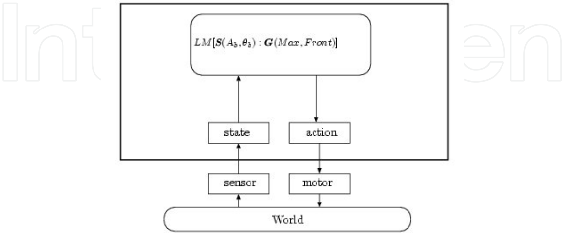
Figure 25. Acquired learning module for task 1
