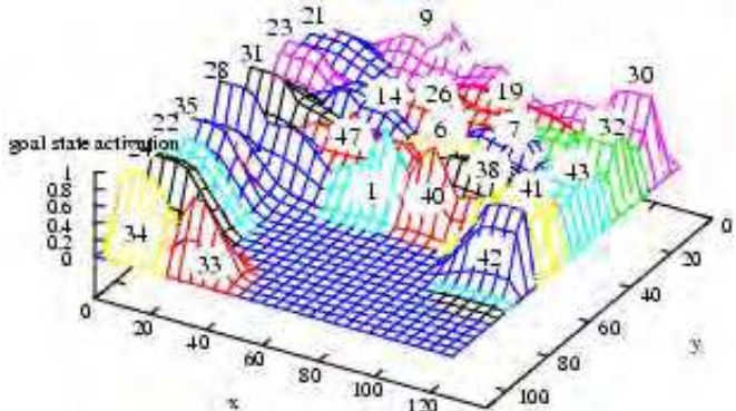
Figure 7. The distribution of learning modules at bottom layer on the normal camera image
