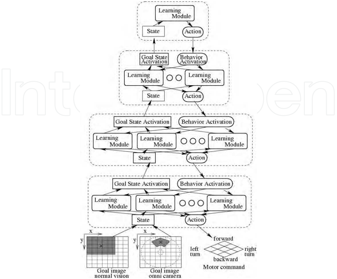
Figure 6. A hierarchical architecture on a monolithic state space
