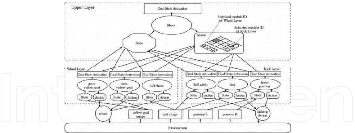
Figure 15. Hierarchical learning system for task 2
