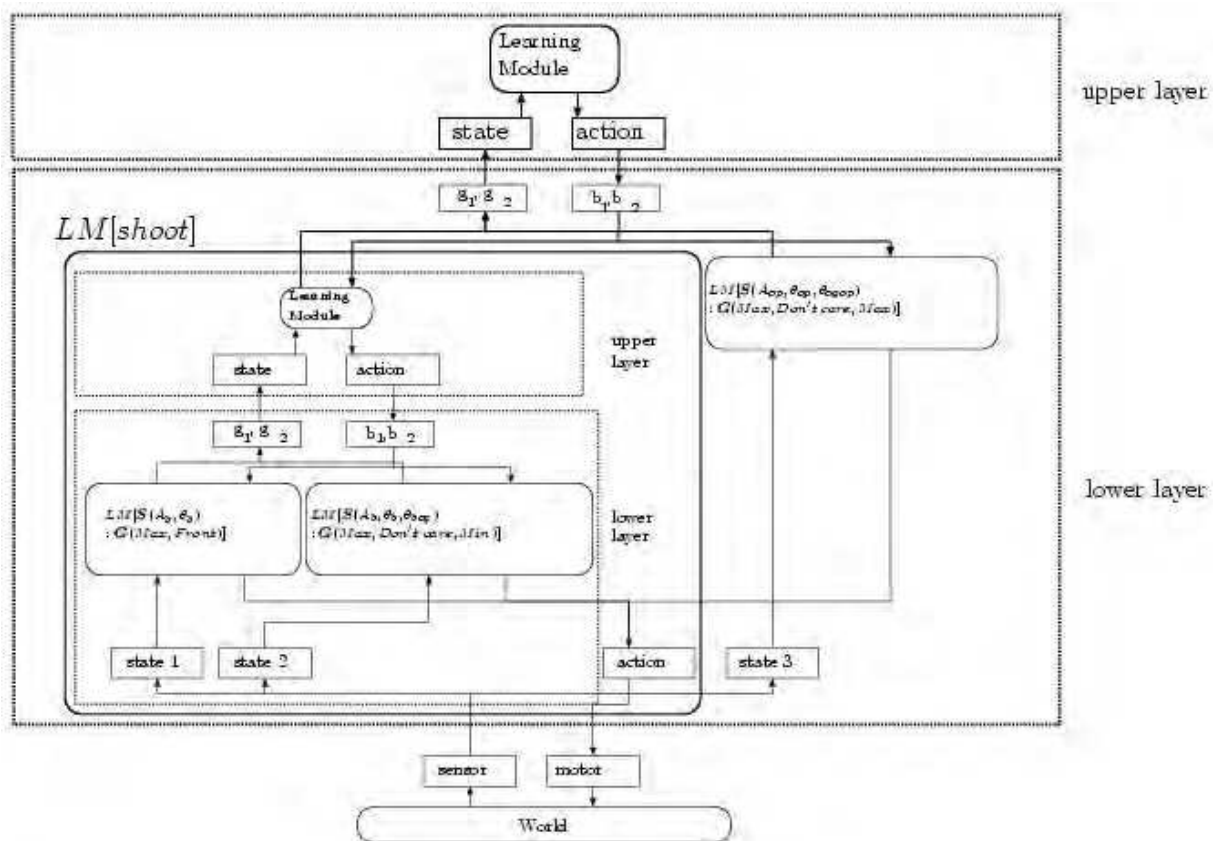
Figure 27. Acquired heirarchical structure for task 3
