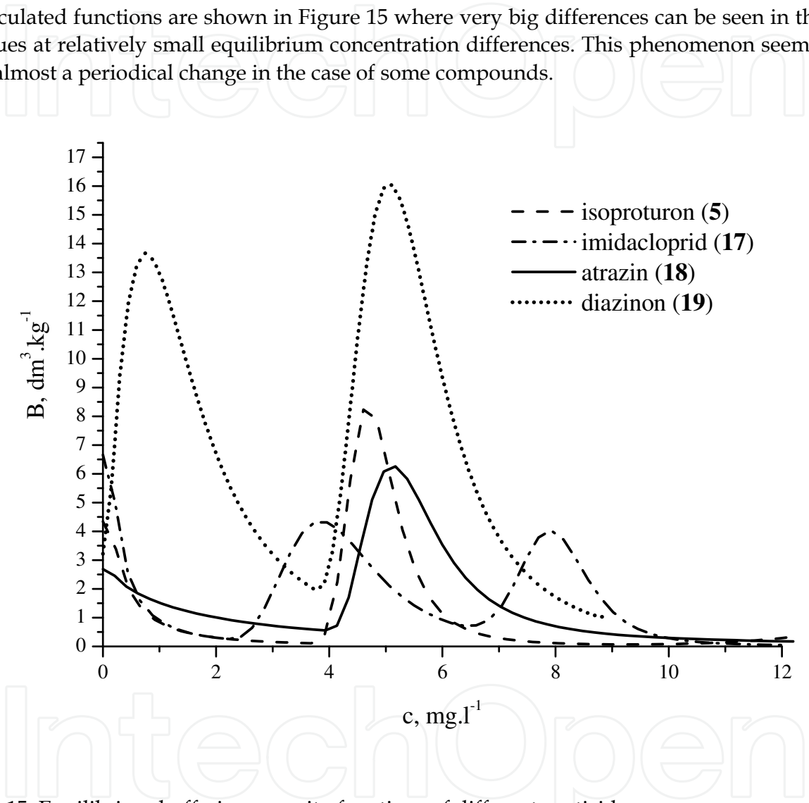
Fig. 15. Equilibrium buffering capacity functions of different pesticides
