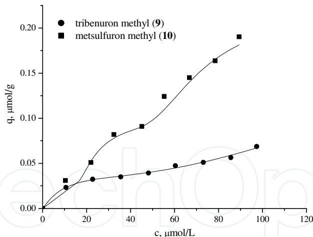
Fig. 13. Adsorption of two sulfonylurea herbicides on chernozem, pH=8.3
