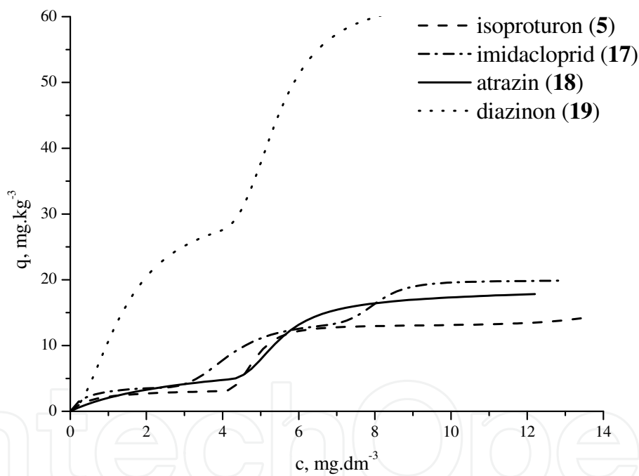
Fig. 14. Adsorption of the investigated pesticides on soil
