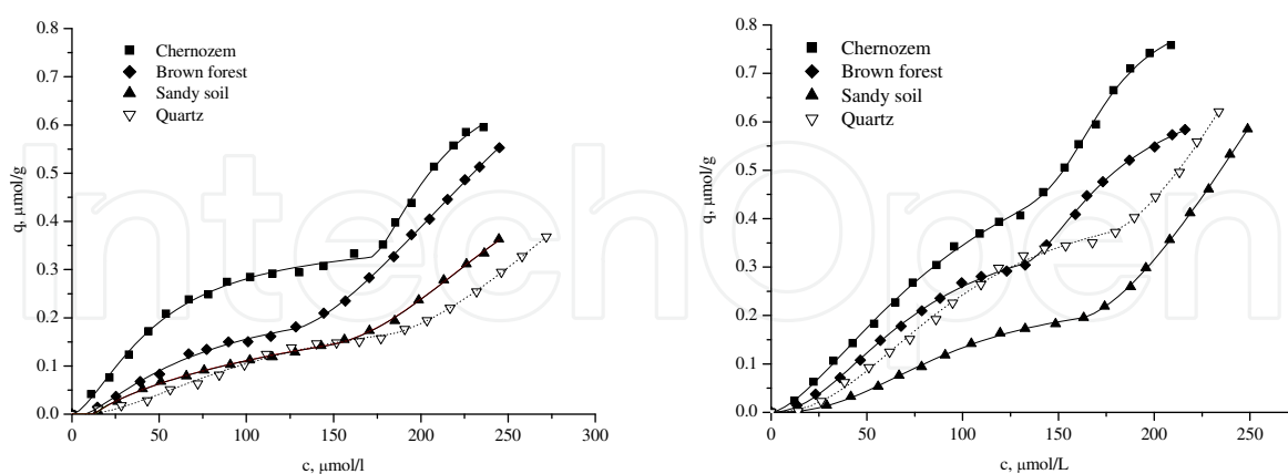
a. Adsorption of acetochlor, pH=7 b. Adsorption of propisochlor, pH=7 Fig. 11. Adsorption of acetochlor ( 1 ) and propisochlor ( 2 ) on different soils and quartz
