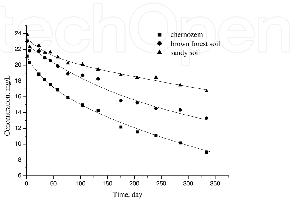
Fig. 4. Degradation of isoproturon in the presence of different soils, pH=7
