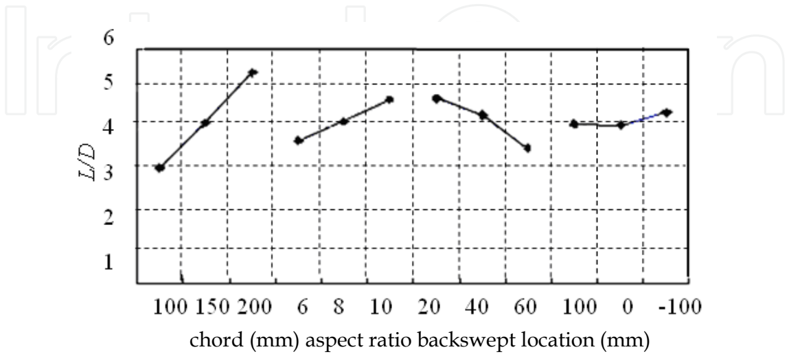
Fig. 6. L/D tendency chart
