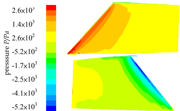
Fig. 20. Pressure distribution chart when angle of attack is 20°
