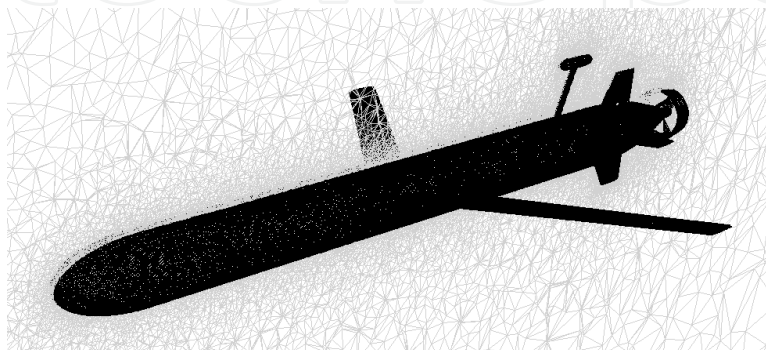
Fig. 5. Whole meshes of the vehicle
