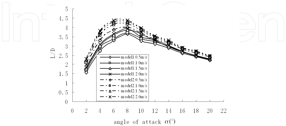
Fig. 28. Lift-to-drag ratio versus angle of attack
