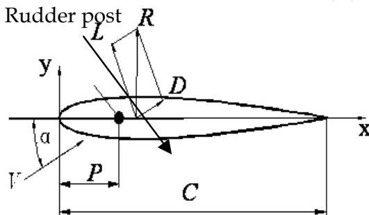
Fig. 14. Foil section and hydrodynamic force
