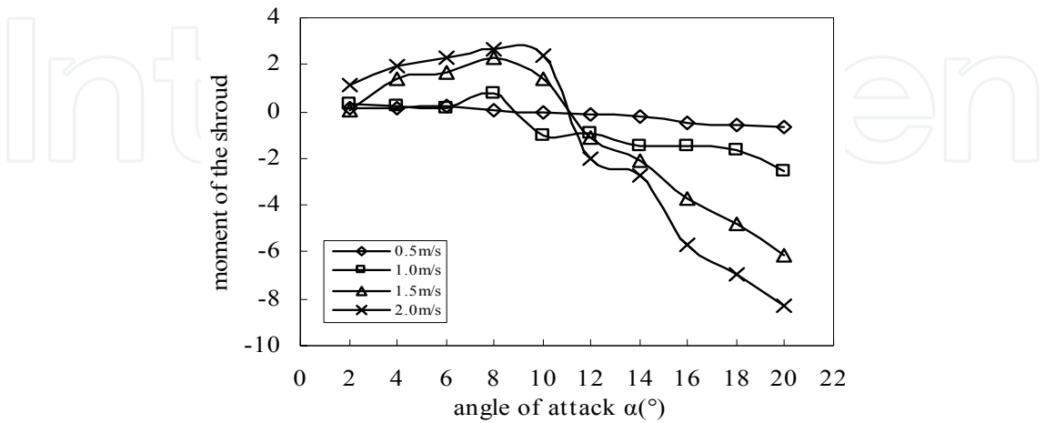
Fig. 31. The moment of the shroud versus angle of attack of model one
