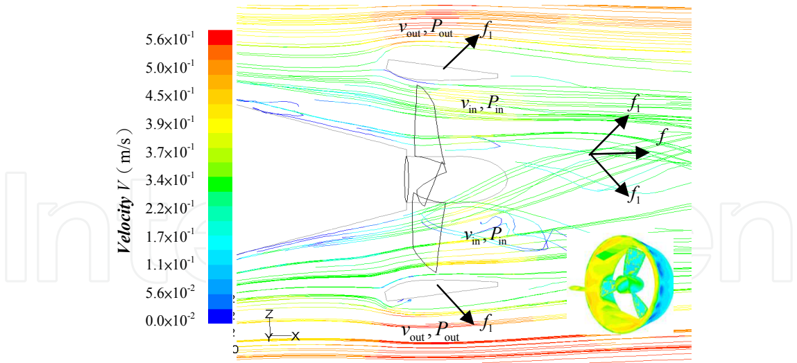
Fig. 27. The local velocity streamline diagram of model1 ( v = 0.5m / s )
