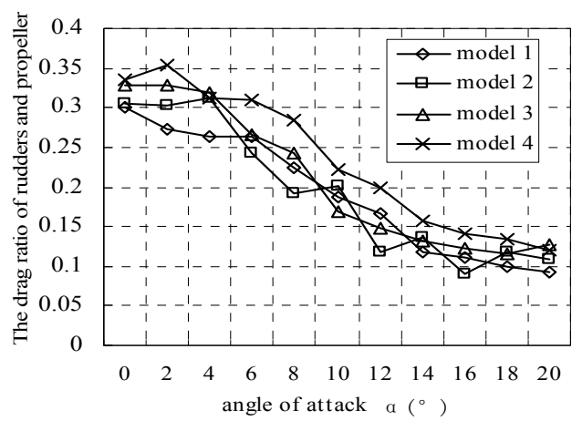
Fig. 11. The drag ratio of rudders and propeller
