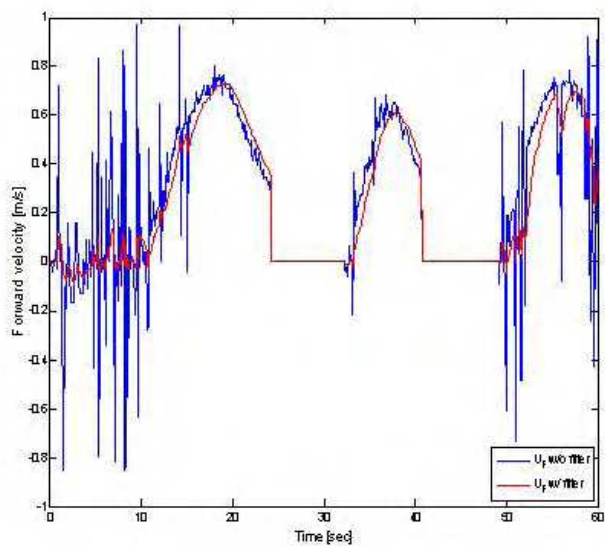
Fig. 14. Calculated forward speeds.
