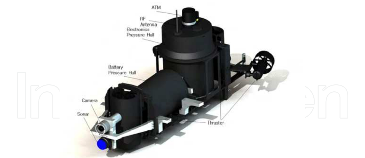
Fig. 2. Mechanical arrangement of P-SURO AUV.
