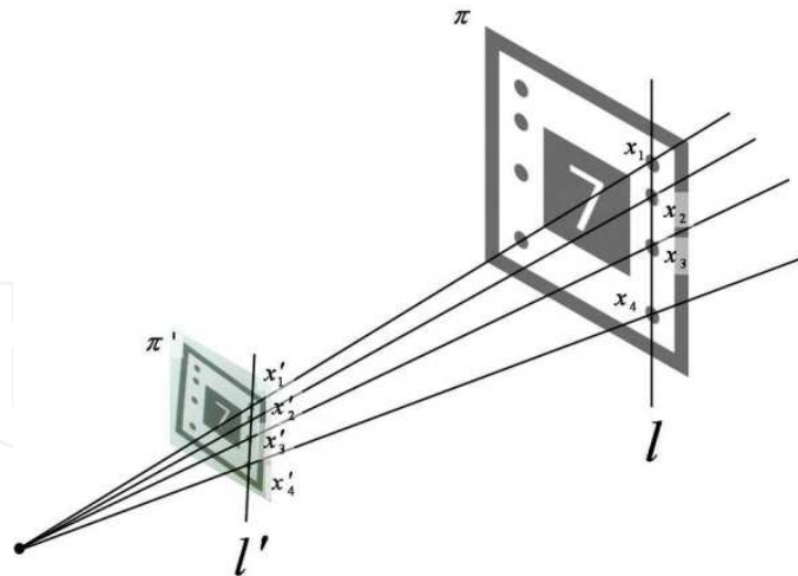
Fig. 6. Cross-ratio in the projective space.
