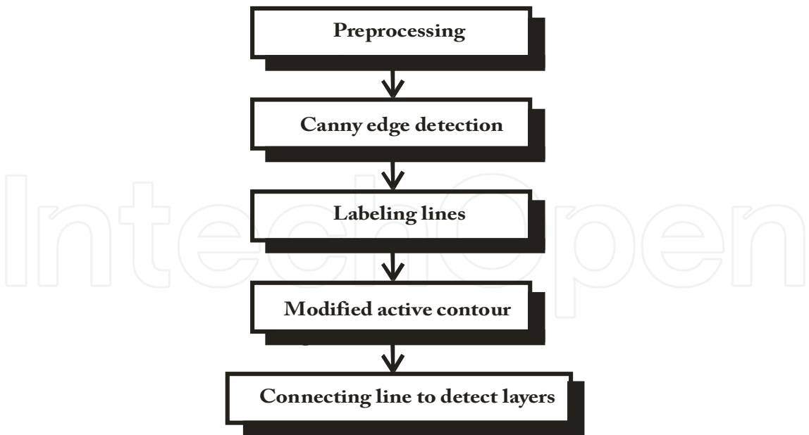
Fig. 8. Block scheme of CCA algorithm
