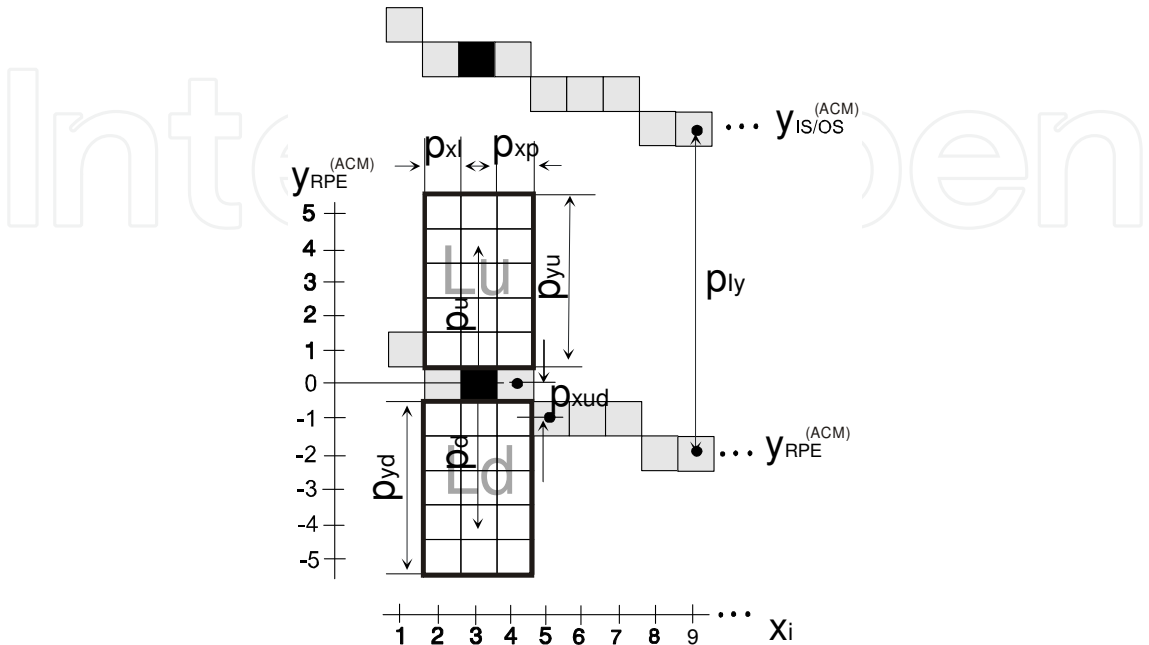
Fig. 6. Scheme of visual values scaling difference of brightness method
