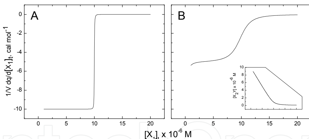
Fig. 5. Titrant-titrant binding in the presence of a competitor. A, simulated 1:1 titrant-titrant binding in the absence of competitor. The parameters are K_1 = 10^{-10} M, \Delta H_1 = -10 kcal mol ^{-1} , and [Y]_t = 10 \mu M. Data representing this level of affinity would be unfit for model-fitting; K_1/[Y]_t = 10^4 . B, in the presence a competitor, X_2 , at 10 \mu M ( K_2 = 10^{-8} M, \Delta H_2 = -5 kcal mol ^{-1} ). Inset, titration of the competitor.
