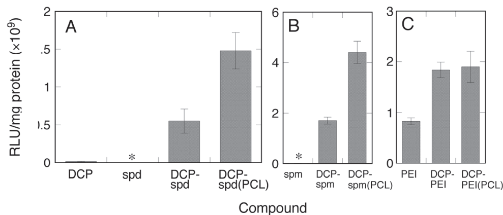
Fig. 4. Transfection efficacy of polyamine-lipid conjugates, DCP-spd (A), DCP-spm (B), and DCP-PEI (C), and their constituents, DCP (A) and polyamines, spermidine (spd, A), spermine (spm, B) and PEI1800 (PEI, C), on COS-1 cells. Efficacy was evaluated with the luciferase activity. The observed values for spermidine and spermine indicated by the asterisks (*) were apparently negligible on the activity scale shown. The conjugates DCP-spd , DCP-spm , and DCP-PEI represent their micellar aggregate forms, and DCP-spd(PCL) , DCP-spm(PCL) , and DCP-PEI(PCL) represent the conjugate-based PCLs (conjugate/DOPE/cholesterol = 1/1/1 (mol/mol/mol)). The nitrogen/phosphate (N/P) ratio was 16/1 for the polyamine conjugate/DNA complexes. For the monoanionic DCP, the molar ratio, DCP/nucleotide = 16/1, was applied as a negative control experiment. Transfection was conducted in the presence of 10% FBS.
