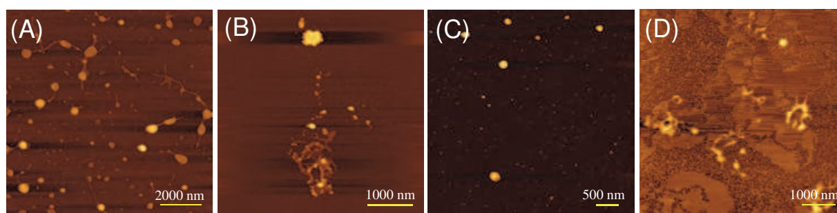
Fig. 7. AFM images of disassembled lipoplexes, DCP-sp d (PCL)/DNA (A and B) and DCP-sp m (PCL)/DNA (C and D) by acidification at pH 4. The acid-treated suspensions of complexes were put on bare mica (A, C) and PLL-mica (B and D). After removal of the solution the images were acquired. Scale bars: 2000 nm (A), 1000 nm (B), 500 nm (C), 1000 nm (D).
