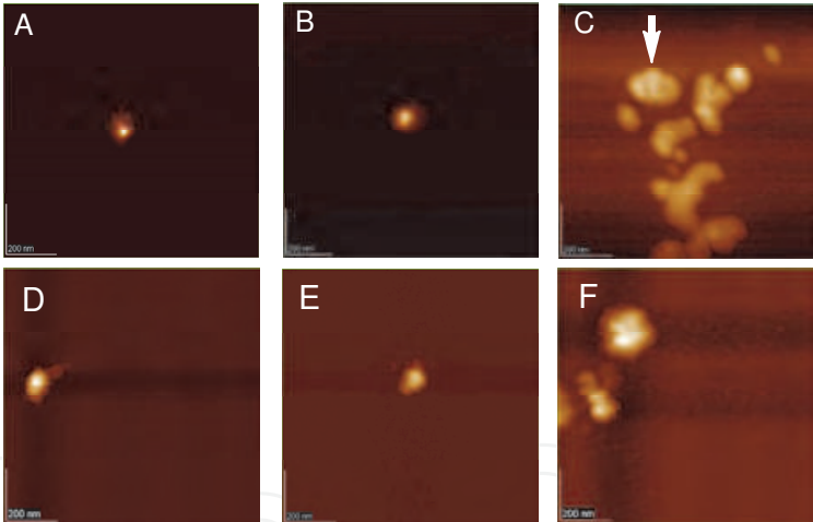
Fig. 2. AFM images of arrays of compounds, DCP-spd (A), DCP-spm (B), DCP-PEI (C), DPPA-spd (D), DPPA-spm (E), and DPPA-PEI (F). The compound was suspended in distilled water then dropped onto a mica surface by spin coating. All scale bars represent 200 nm. The object indicated by the arrow is discussed in the text.
