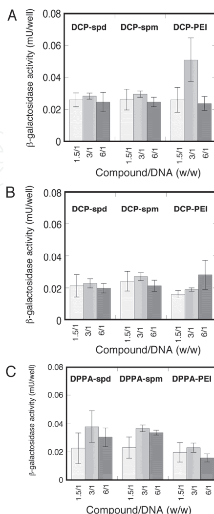
Fig. 1. Transfection efficacy of polyamine-DCP (A and B) and polyamine-DPPA conjugates (C) on VSMC, in the absence (A and C) and the presence of 20% of FBS (B). The ratios of compound/ \beta -galactosidase plasmid DNA (w/w) were 1.5/1, 3/1, and 6/1, respectively.
