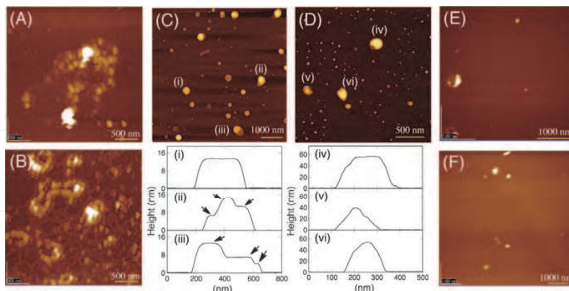
Fig. 6. AFM images of PCL/plasmid DNA (ColE1; 6646 bp) lipoplexes: (A), DCP-sp d (PCL)/DNA (N/P = 5); (B), DCP-sp m (PCL)/DNA (N/P = 5); (C), DCP-sp d (PCL)/DNA (N/P = 24); (D), DCP-sp m (PCL)/DNA (N/P = 24); (E and F), DCP-PEI (PCL)/DNA complex (N/P = 24). Scale bars shown in the images are 500 nm (A, B, and D) and 1000 nm (C, E, and F). The PCL/DNA complexes were applied to PLL-mica (A and B) and bare mica (C, D, E, F). All images were taken under an ambient air conditions. Height profiles of the objects (i)-(iii) in C and (iv)-(v) in D are shown below these images. Arrows in (ii) and (iii) indicate step-like profiles discussed in the text. Images E and F for DCP-PEI (PCL)/DNA were taken from a different area of the bare mica surface.
