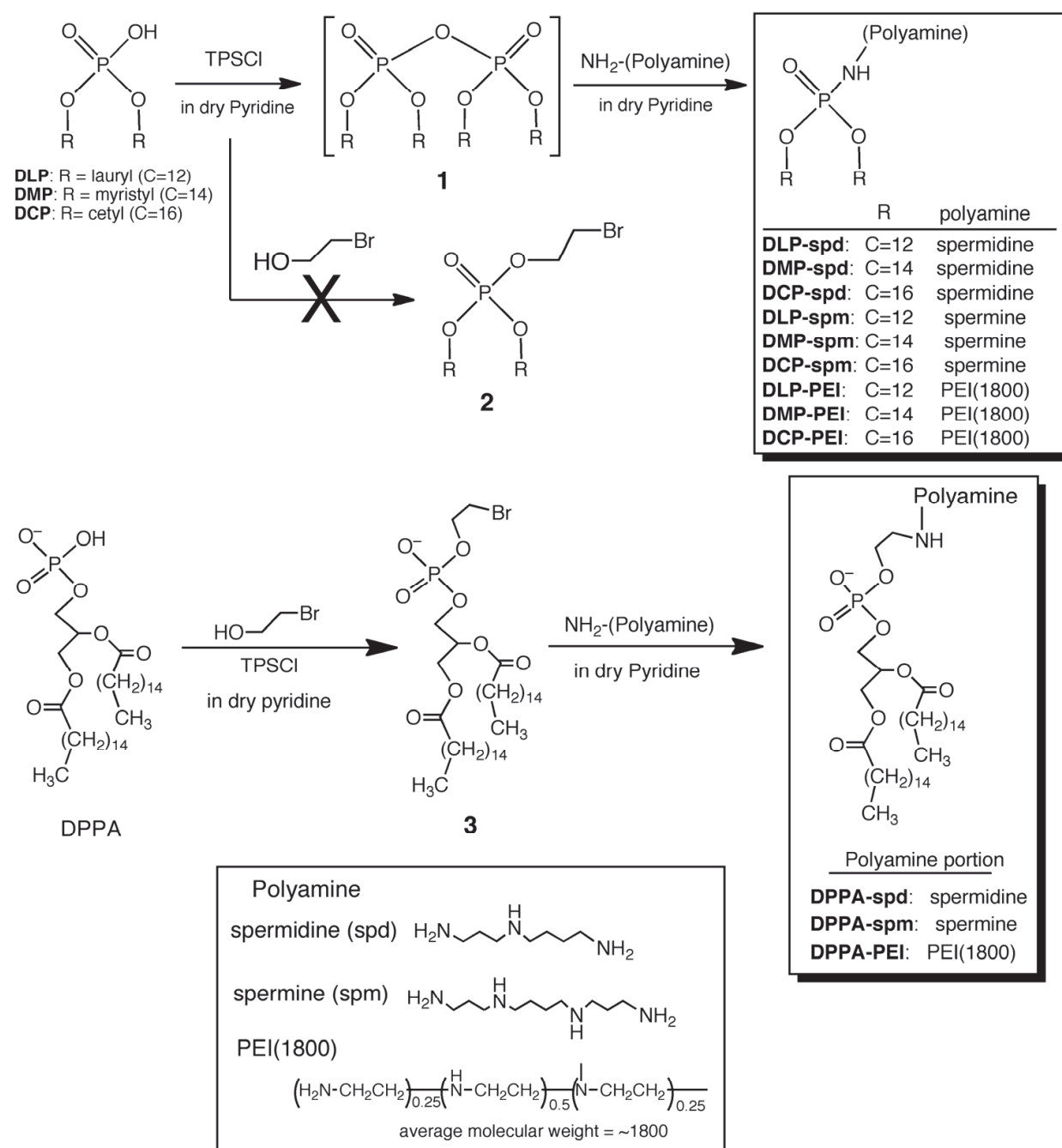
Scheme 1. Synthetic Strategy for Polyamine-lipid Conjugates.
