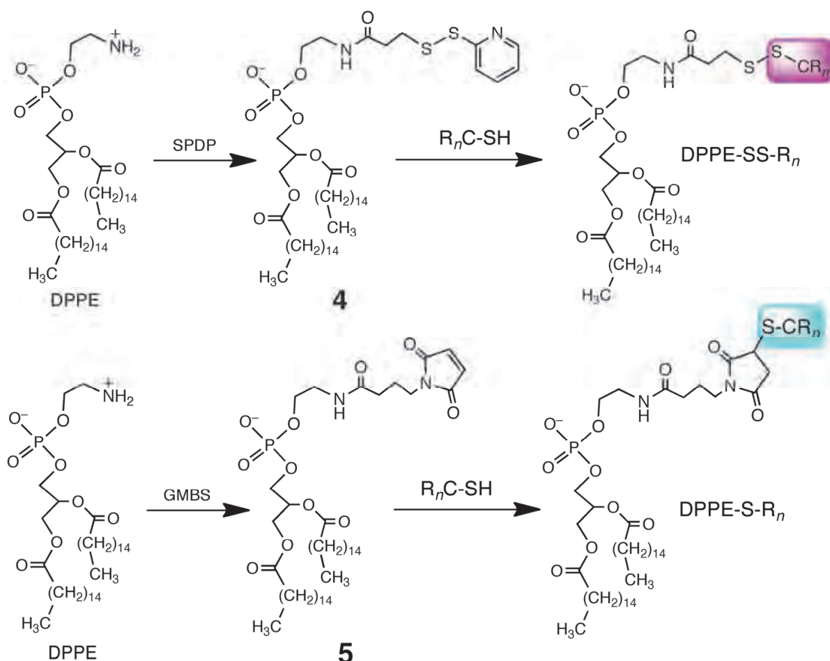
Scheme 2. Synthetic strategy for peptide-phospholipid conjugates
