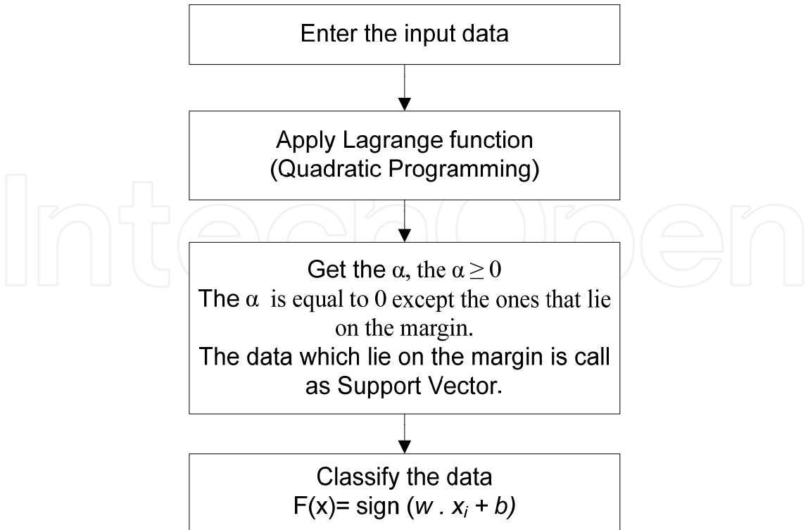
Fig. 13. Flowchart of SVM algorithm.
