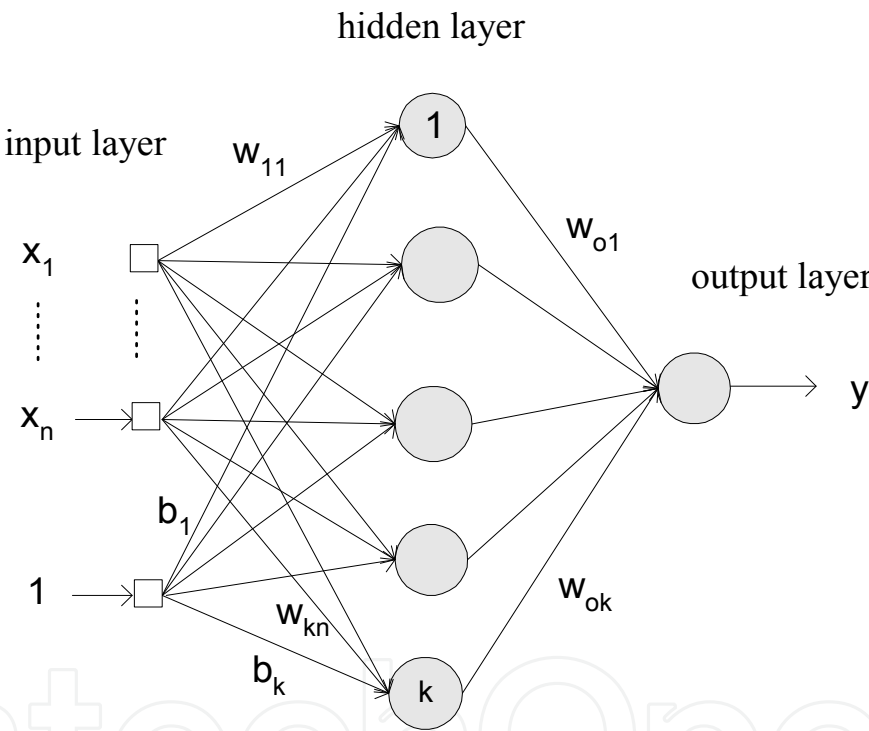
Fig. 11. A Typical multilayer feedforward neural network structure.
