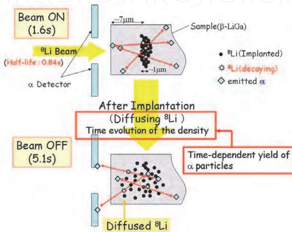
Fig. 2. Schematic view of the principle for measuring diffusion coefficients in \beta\text{-LiGa} (a typical sample of the inter-metallic Li compounds presently used) when the short-lived \alpha -emitting ^8\text{Li} was used as the diffusion tracer. The yield of \alpha particles measured at a time is a measure of the diffused distribution of ^8\text{Li} primarily implanted in the sample with a depth of about 7\mu\text{m} .
