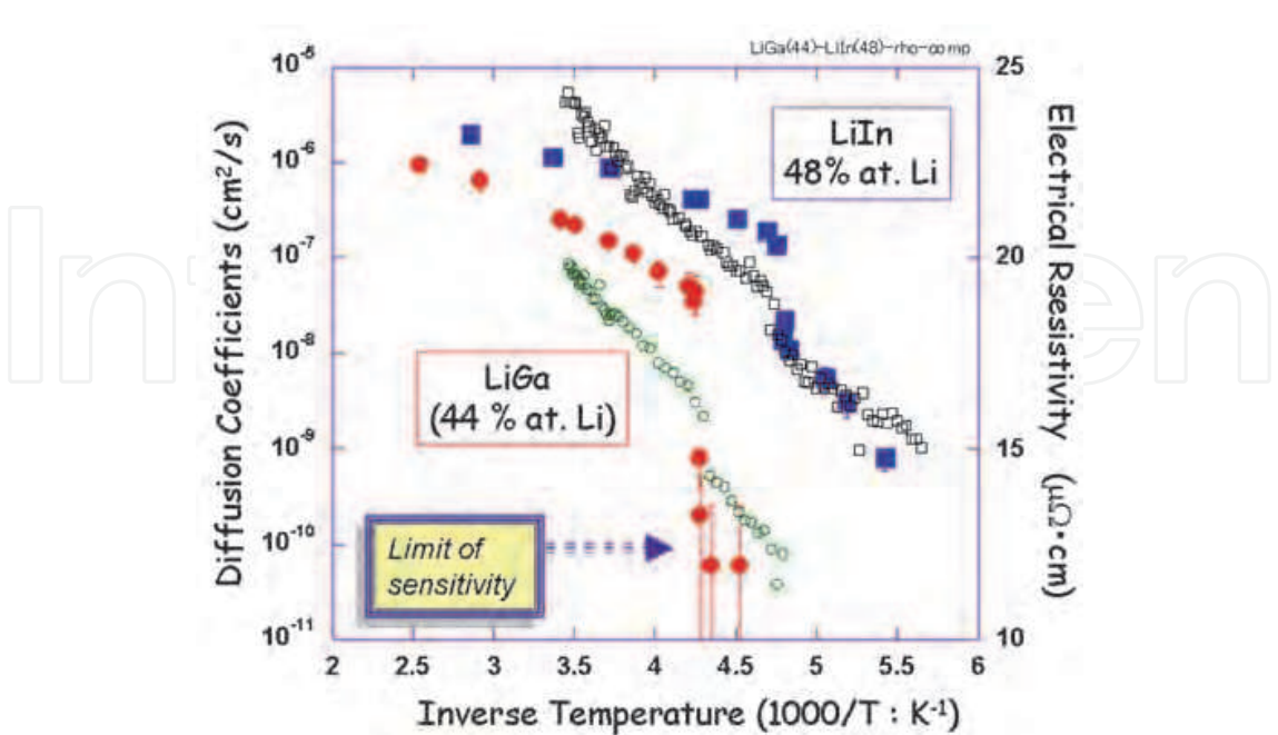
Fig. 11. Temperature-dependence of diffusion coefficients (closed symbols) and electrical resistivity (open symbols) for \beta -LiGa with 44 at. % Li, and \beta -LiIn with 48 % at. Li.
