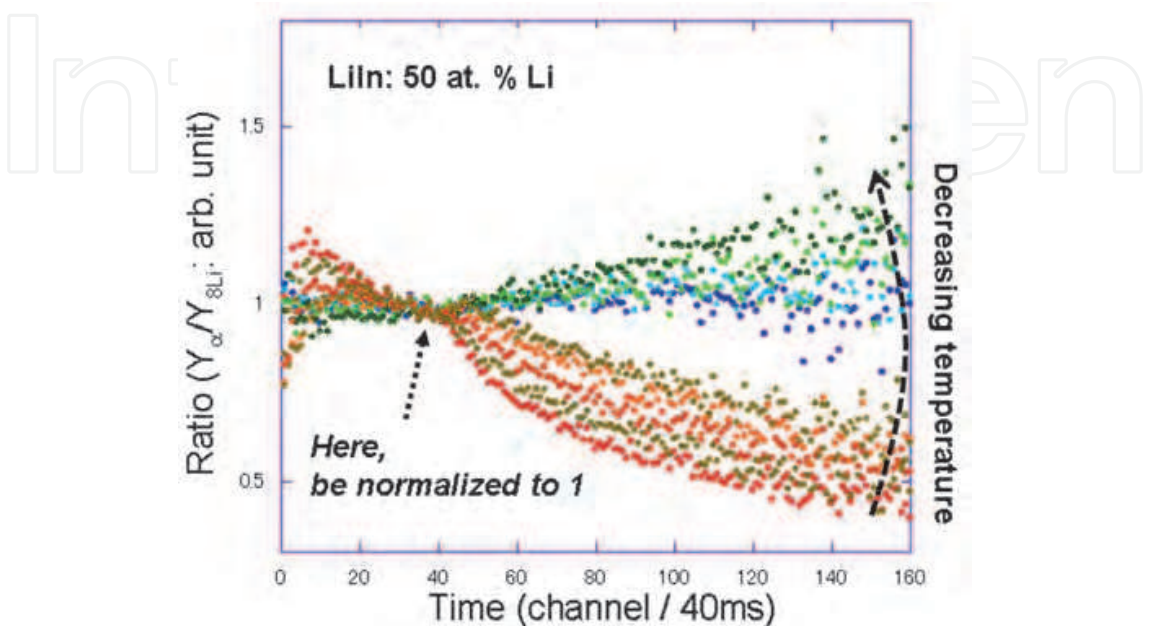
Fig. 10. Time spectra of \alpha -particle yields measured at various temperatures for LiIn. The spectra were corrected for removing trivial time dependence and further normalized properly for easy comparison.
