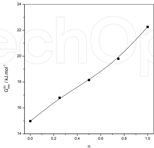
Fig. 4. Variation of Gibbs free energy at the air/water interface, G_{\min}^{(s)} of the amphiphilic drug IMP at different concentration (mole fraction) of TX-100.
