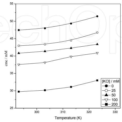
Fig. 8. Effect of temperature on the cmc of IMP solutions.
