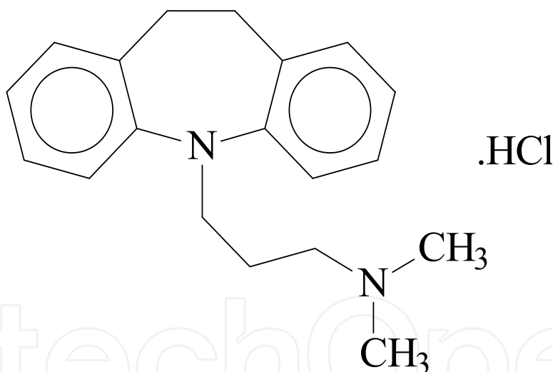
Scheme 1. The molecular structure of amphiphilic tricyclic antidepressant drug, 5-[3-(dimethylamino)propyl]-10,11-dihydro-5 H -dibenz[ b,f ]azepine hydrochloride (imipramine hydrochloride, IMP) used in the present study.
