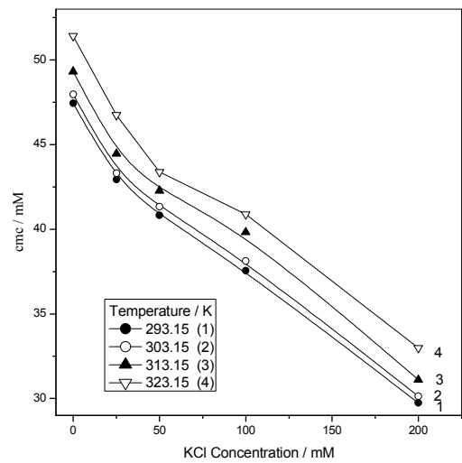
Fig. 7. Effect of KCl concentrations on the cmc of IMP solutions.
