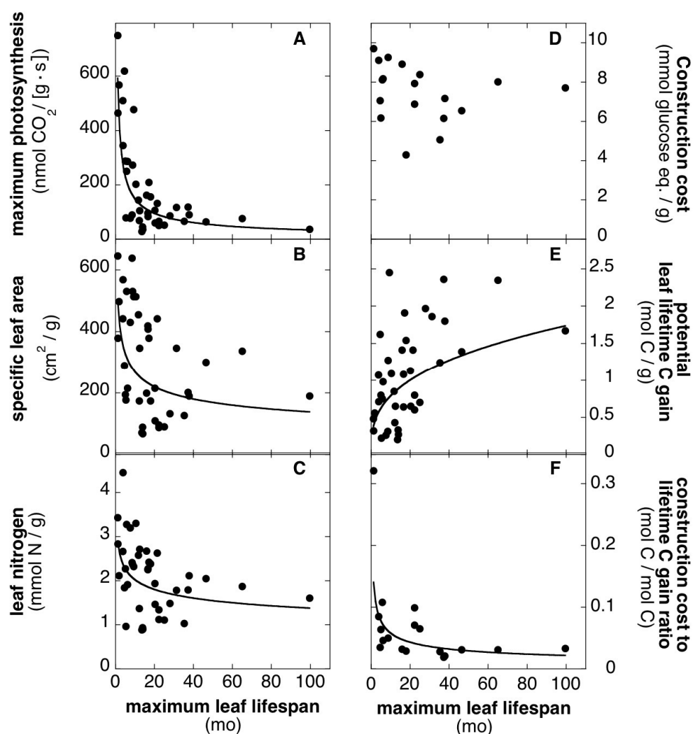
Fig. 6. Interspecific variation in leaf lifespan versus (A) P_{\text{max}} , (correlation coefficient, r=0.82 ), (B) SLA, ( r=0.51 ), (C) N_L , ( r=0.47 ), (D) leaf CC, (Non-significant correlation), (E), estimated P_{\text{life}} , ( r=0.54 ), and (F) a carbon-based leaf cost/benefit ratio ( \text{CC}/P_{\text{life}} ; r=0.80 ). Each datapoint is the mean from 3-4 observations made on each of 40 (A, B, C and E) species or a subset of 18 species (D and F) in controlled environment mesocosms in Biosphere2 in Arizona, U.S.A. Lines of best-fit for power functions are plotted when the association between variables was significant ( P < 0.05 ) with correlation coefficients ( r ) as reported above.
