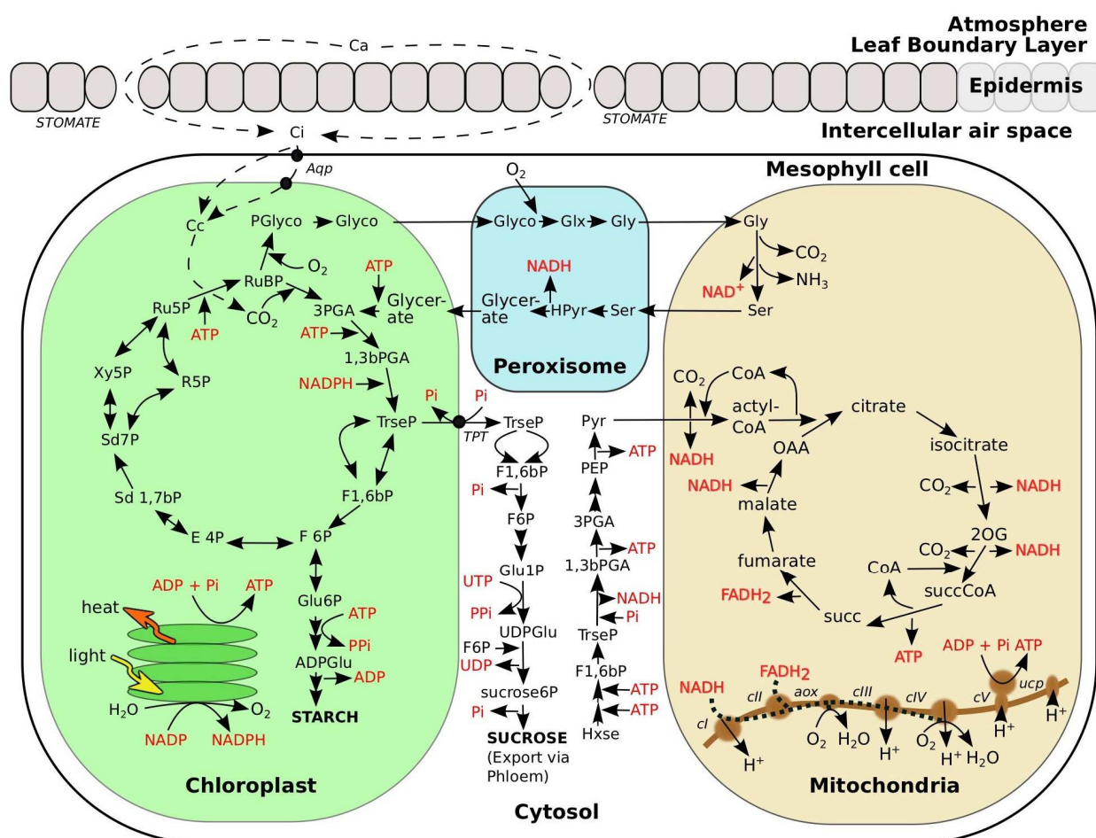
Fig. 3. Primary carbon metabolism in a photosynthetic C 3 leaf. An abbreviated depiction of foliar CO 2 uptake, chloroplastic light-reactions, chloroplastic carbon fixation (Calvin cycle), chloroplastic starch synthesis, cytosolic sucrose synthesis, cytosolic glycolysis, mitochondrial citric acid cycle, and mitochondrial electron transport. The photorespiration cycle spans reactions localized in the chloroplast, the peroxisome, and the mitochondria. Stacked green ovals (chloroplast) represent thylakoid membranes. Dashed arrows near figure top represent the CO 2 diffusion path from the atmosphere (Ca), into the leaf intercellular airspace (Ci), and into the stroma of the chloroplast (Cc). Solid black arrows represent biochemical reactions. Enzyme names and some substrates and biochemical steps have been omitted for simplicity. The dotted line in the mitochondria represents the electron transport pathway. Energy equivalent intermediates (e.g., ADP, UTP, inorganic phosphate; Pi) and reducing equivalents (e.g., NADPH, FADH 2 , NADH) are labeled in red. Membrane transporters Aqp (CO 2 conducting aquaporins) and TPT (triose phosphate transporter) are labeled in italics. Mitochondrial inner-membrane electron transport and proton transport proteins are labeled in small case italics.
