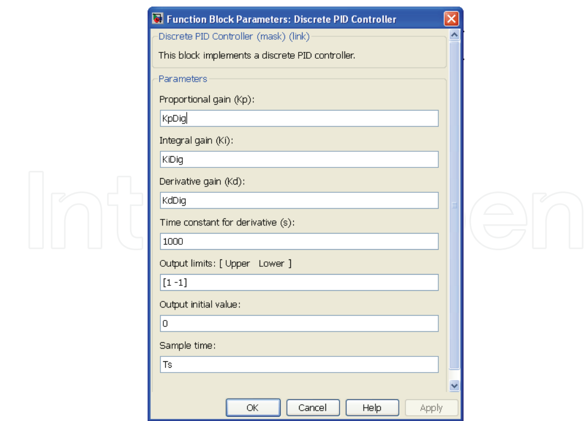
Fig. 7. Configuration Window Discrete PID
