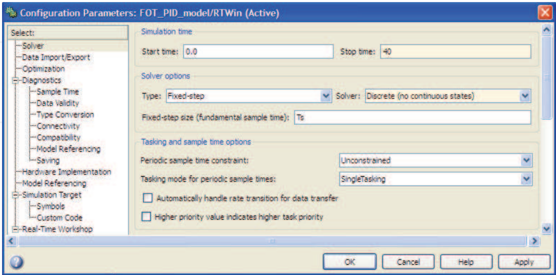
Fig. 3. Solver configuration
