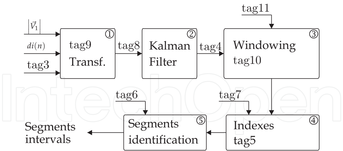
Fig. 6. Example of data segmentation and proposed detection index.
