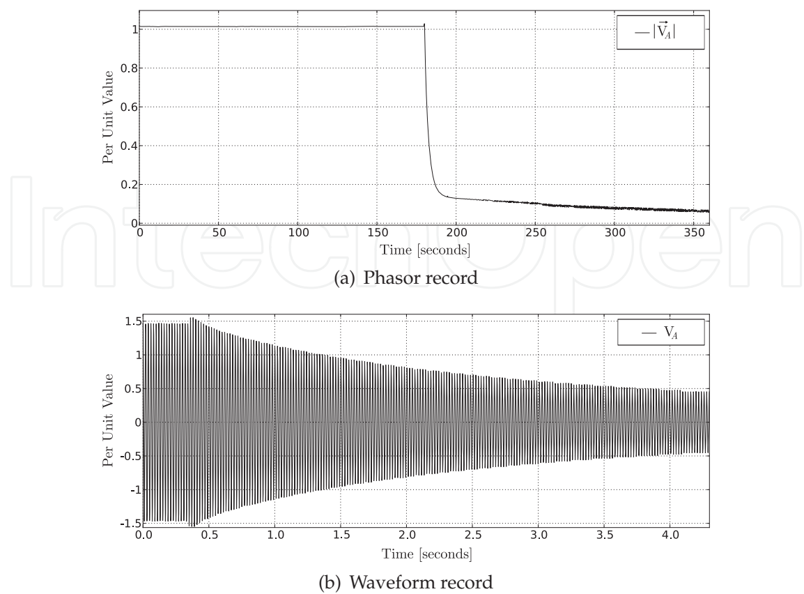
Fig. 2. A disturbance in phasor and waveform record.
