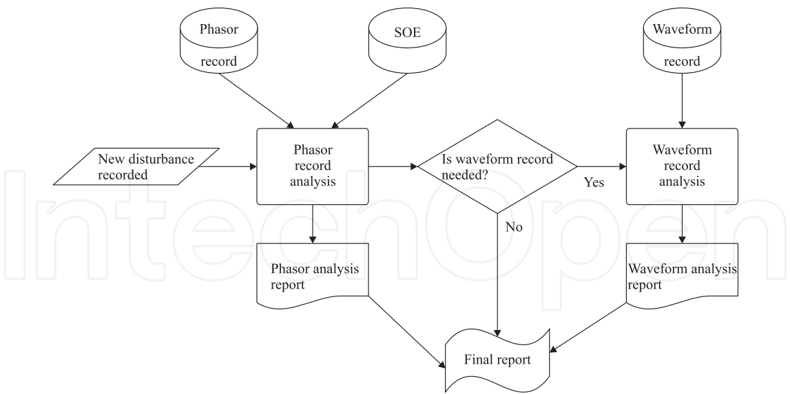
Fig. 3. Structure of the proposed scheme.
