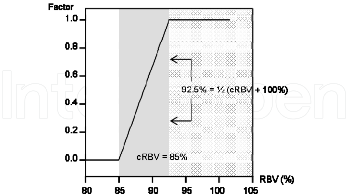
Fig. 3. BVM® algorithm (from Fresenius). This figure illustrates an example where the cRBV is set at 85%. When the actual RBV is 85% or less (white area), factor is 0 and UF stops. When RBV is greater than halfway between cRBV and 100% (here, halfway between 85% and 100% is 92,5%), the factor is 1,0 and UF is maximal (shaded area). In between (gray area), factor is between 0 and 1, and UF is not maximal.
