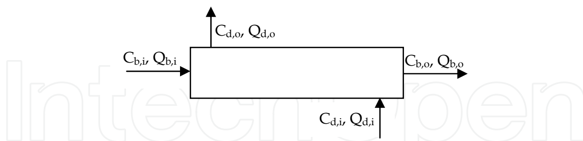
Fig. 1. Schematic description of concentration and flows in dialyzer.
