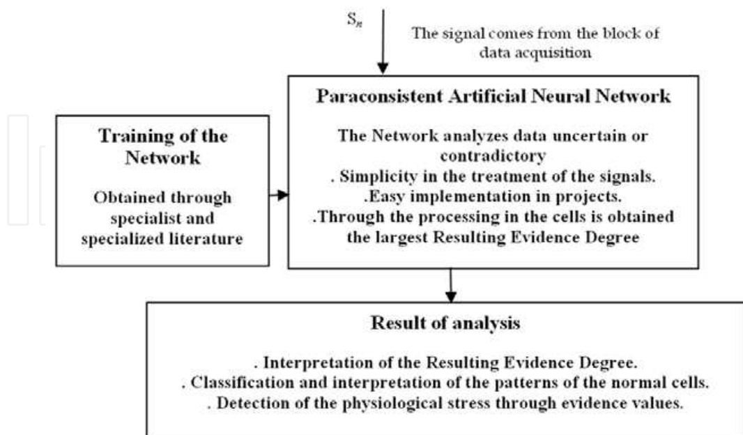
Fig. 8. Diagram in blocks of the Expert system with Paraconsistent Artificial Neural Networks applied to the method of obtaining the physiological stress cells.
