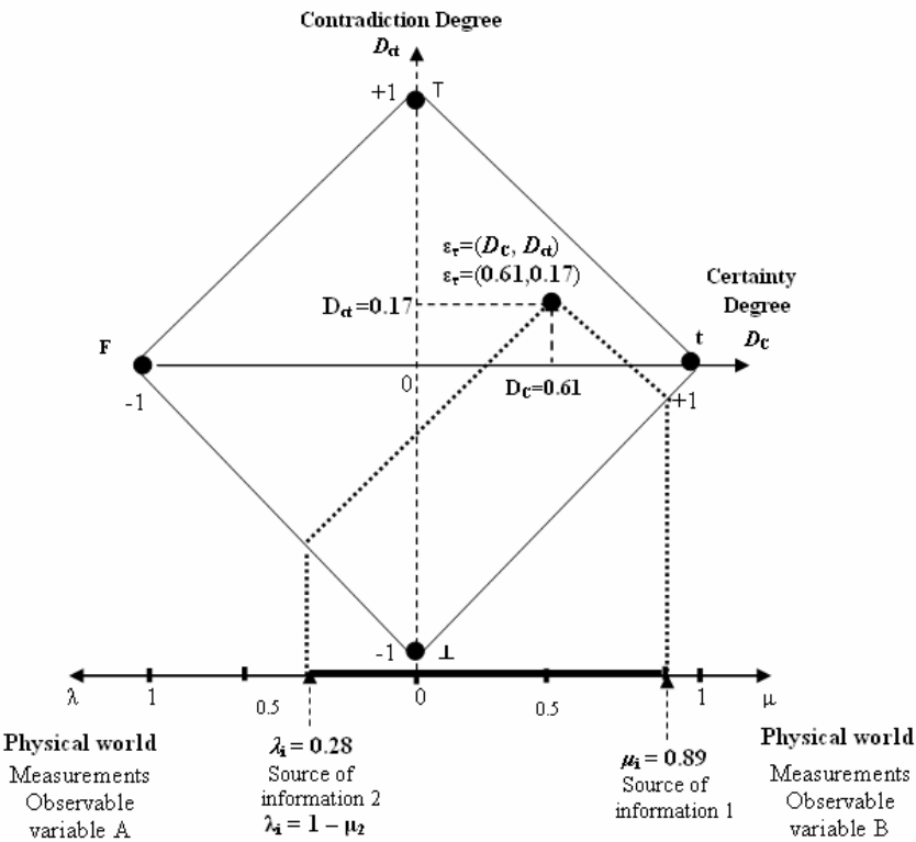
Fig. 2. Paraconsistent logical state \varepsilon_t in the Lattice associated of the PAL2v.
