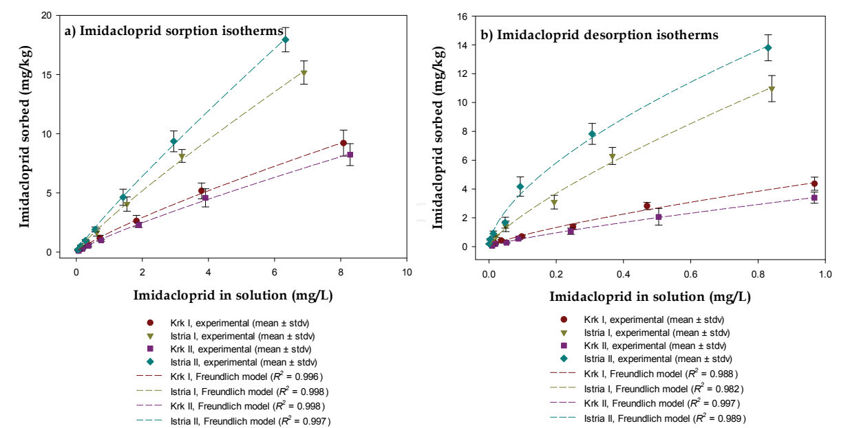
Fig. 6. a) Sorption and b) desorption isotherms of IMI in the tested soils represented by the Freundlich model. Values are means ± standard deviations. Symbols represent the experimental data, while lines represent the theoretical curves described by the Freundlich model.
