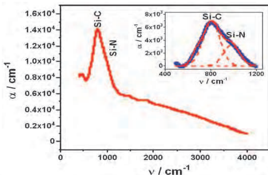
Fig. 3. FTIR spectra of PECVD \text{SiC}_x\text{N}_y film grown at 973 K: total view and deconvolution of the main adsorption band into components.
