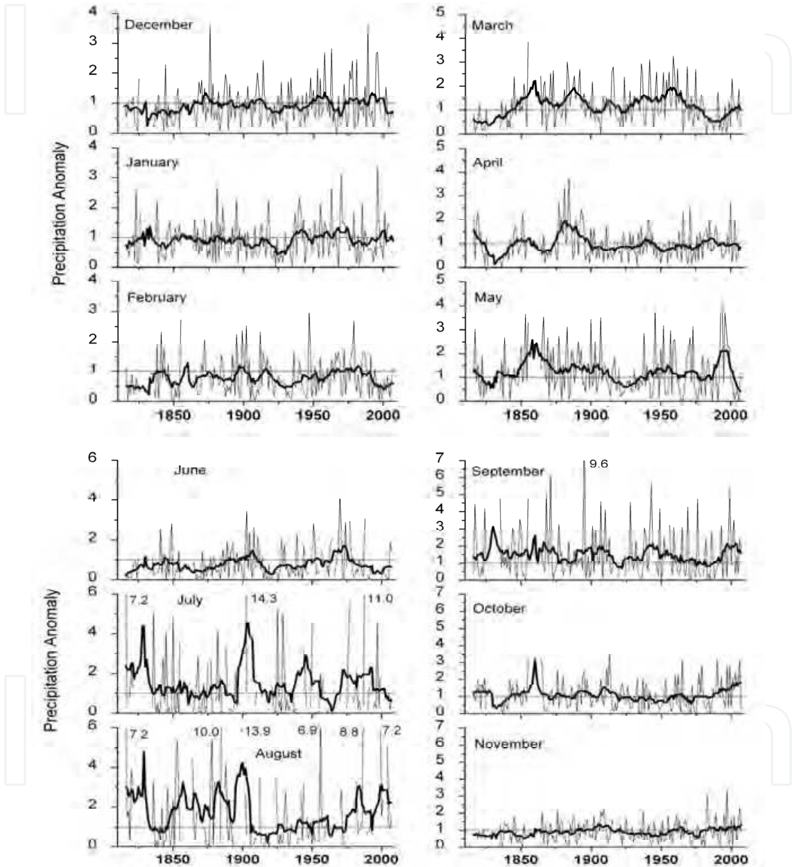
Fig. 11. Monthly precipitation anomaly from instrumental data in Portugal. Non dimensional units, the anomaly being expressed as a ratio with the 1961-1990 reference period. The 1-line level corresponds to the 1961-1990 average. Thin black lines refer to instrumental observations, thick black lines to 11-year running averages. Numbers on the side of peaks indicate the top level, external to the scale. The precipitation (Fig.12) in all the Spanish stations shown in Fig.1 largely differs from month to month, including the reaction to the last three decades of GW, i.e. after 1980. In
