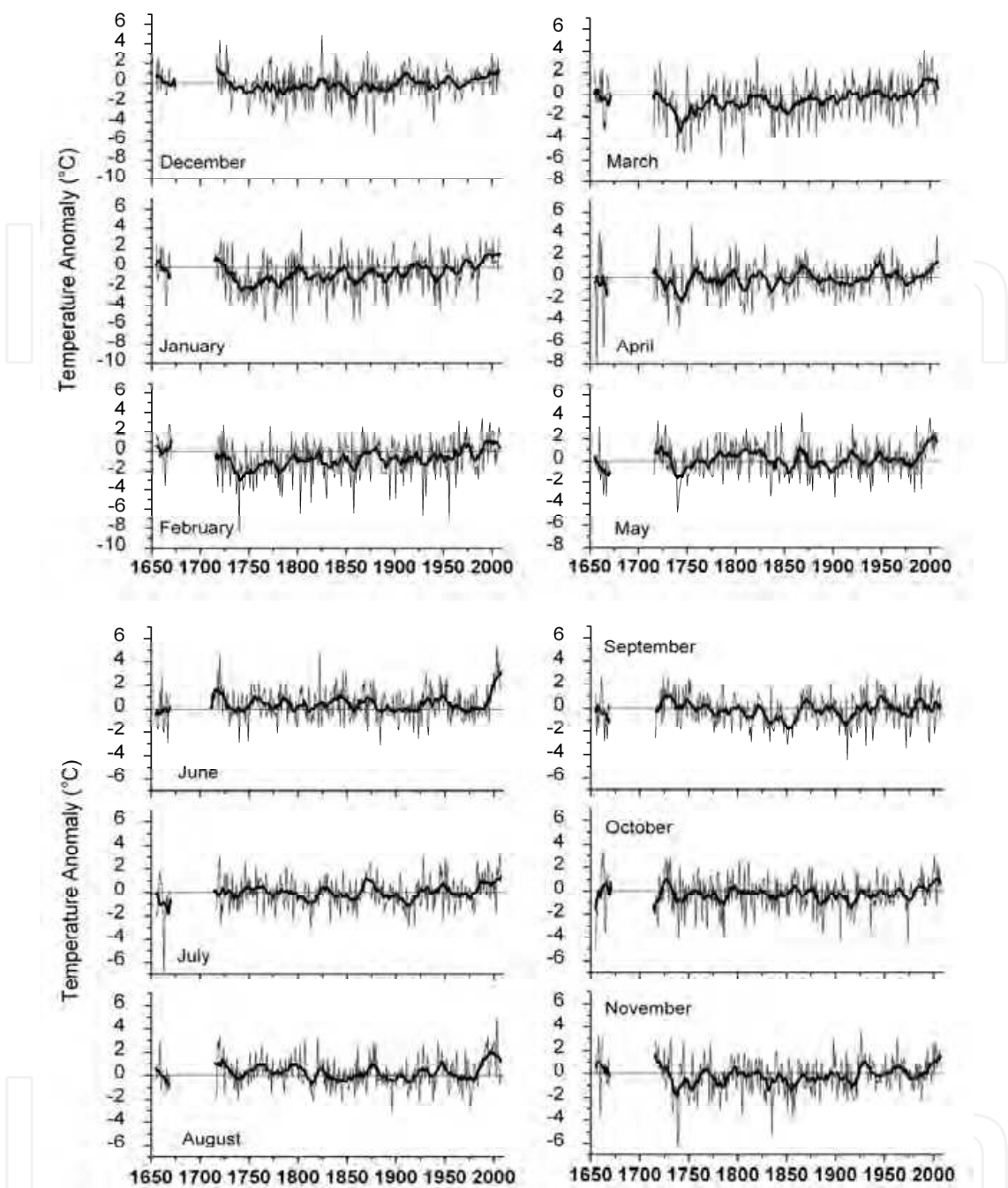
Fig. 9. Monthly temperature anomaly (°C) from instrumental data in Northern-Central Italy. Zero level, thin and thick lines as in Fig.7.
