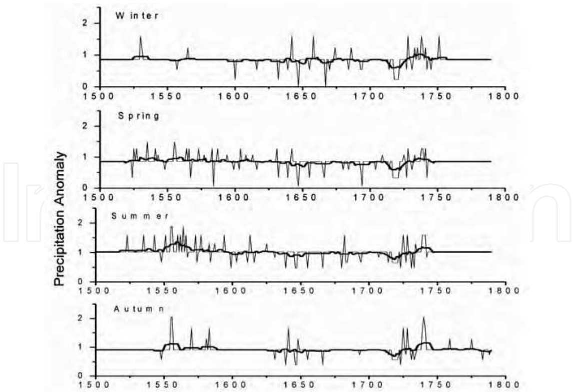
Fig. 5. Seasonal precipitation anomaly from documentary proxy data in Southern France. Symbols as in Figure 2.
