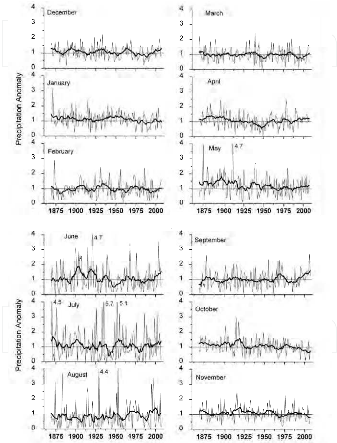
Fig. 15. Monthly precipitation anomaly from instrumental data in Southern Italy. Units and symbols as in Fig.11.
