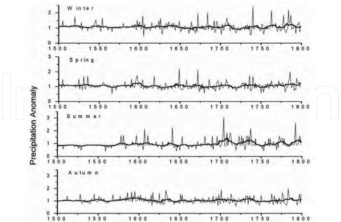
Fig. 4. Seasonal precipitation anomaly from documentary proxy data in Spain. Symbols as in Figure 2.
