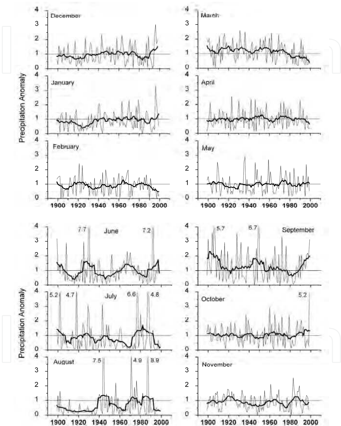
Fig. 12. Monthly precipitation anomaly from instrumental data in Spain. Units and symbols as in Fig.11.
