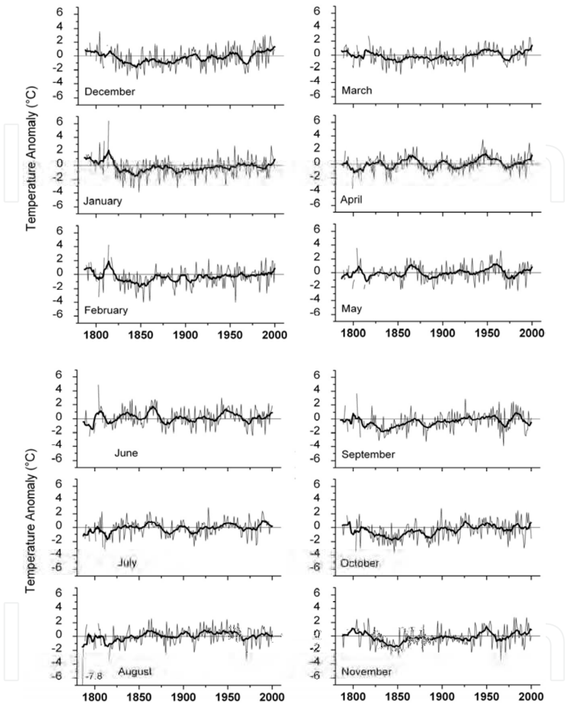
Fig. 7. Monthly temperature anomaly (°C) from instrumental data in Spain. The zero level corresponds to the average of the 1961-1990 reference period. Thin black lines refer to instrumental observations, thick black lines to 11-year running averages.
