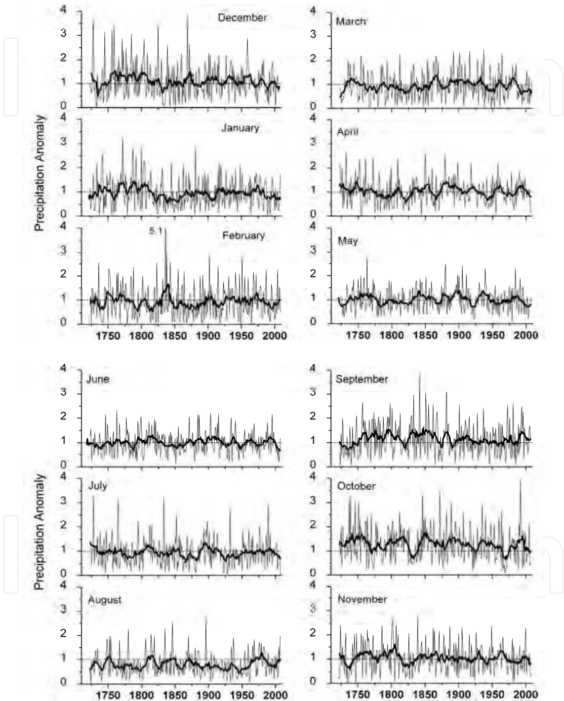
Fig. 14. Monthly precipitation anomaly from instrumental data in Northern-Central Italy. Units and symbols as in Fig.11.
