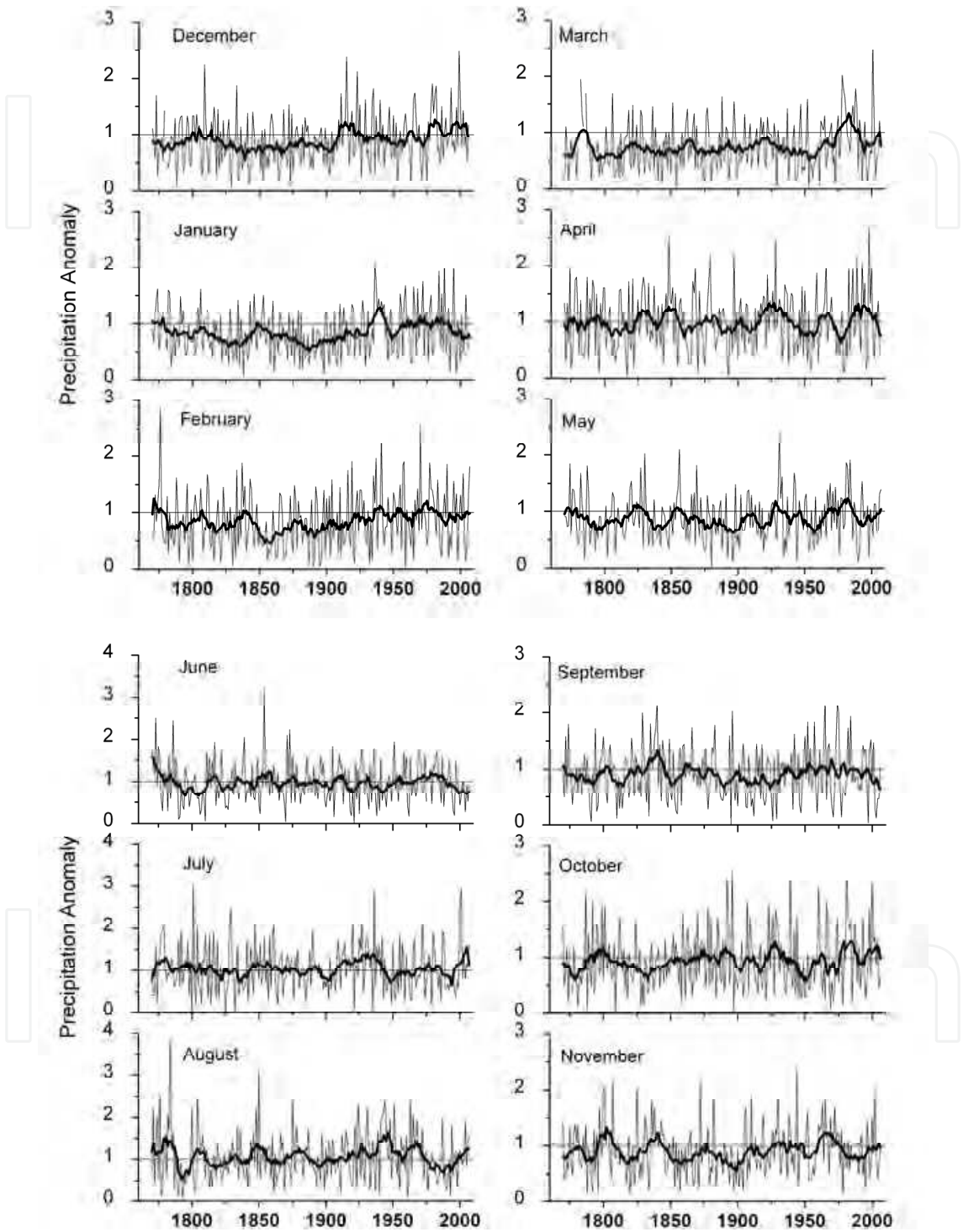
Fig. 13. Monthly precipitation anomaly from instrumental data in Southern France. Units and symbols as in Fig.11.
