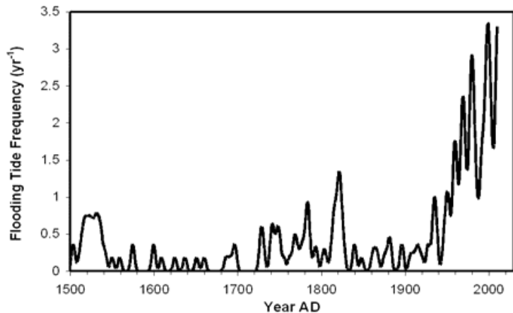
Fig. 17. Occurrence of the flooding tides (i.e. sea level 110 cm higher than the average in 1897) at Venice over the last 500 years. The graph reports the number of independent floods, i.e. one flooding tide per surge disregarding the short-term interruptions and repetitions for the astronomical tide modulation.
