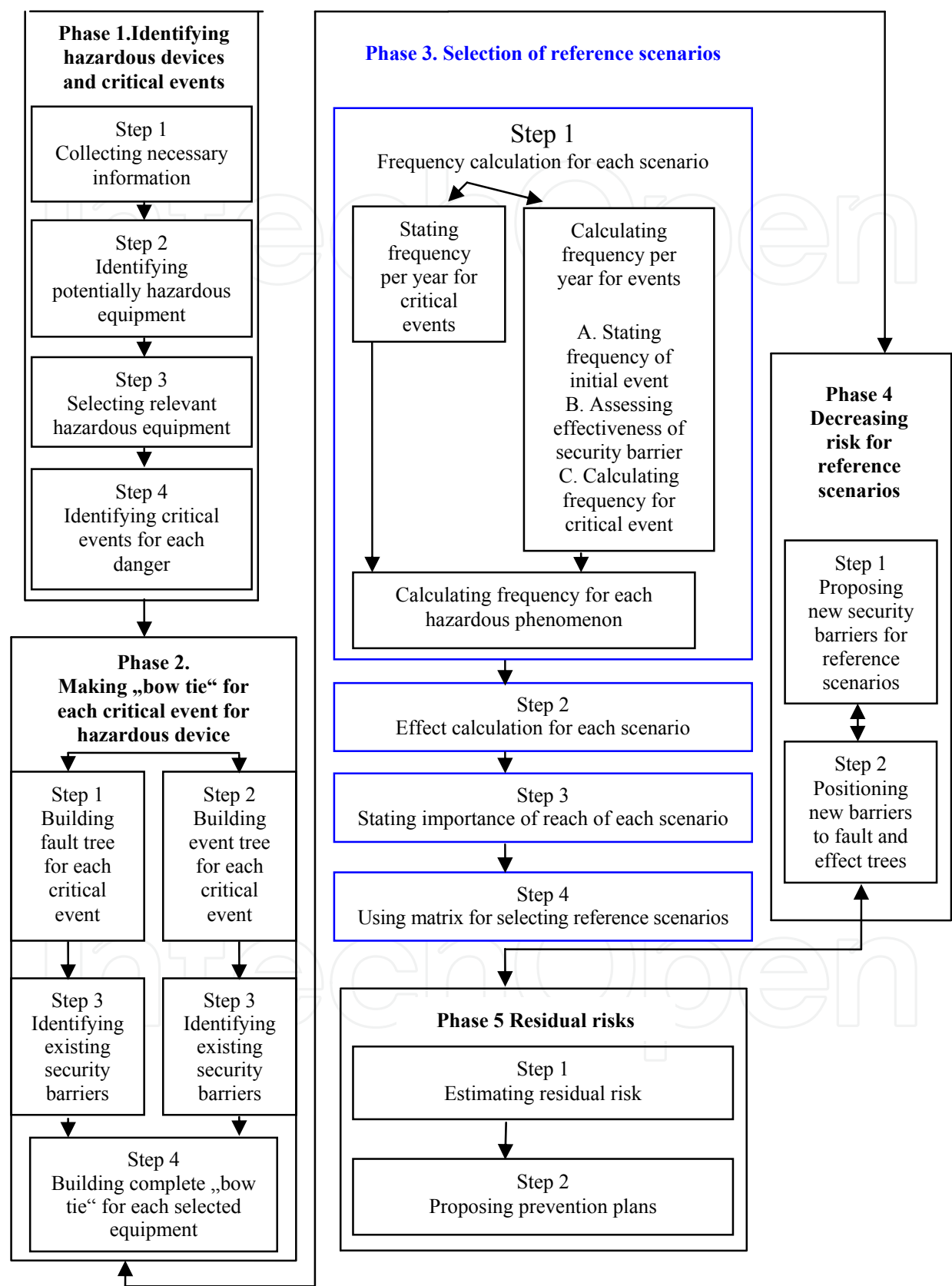
Fig. 3. Systematic approach ARAMIS (ARAMIS final user guide)
