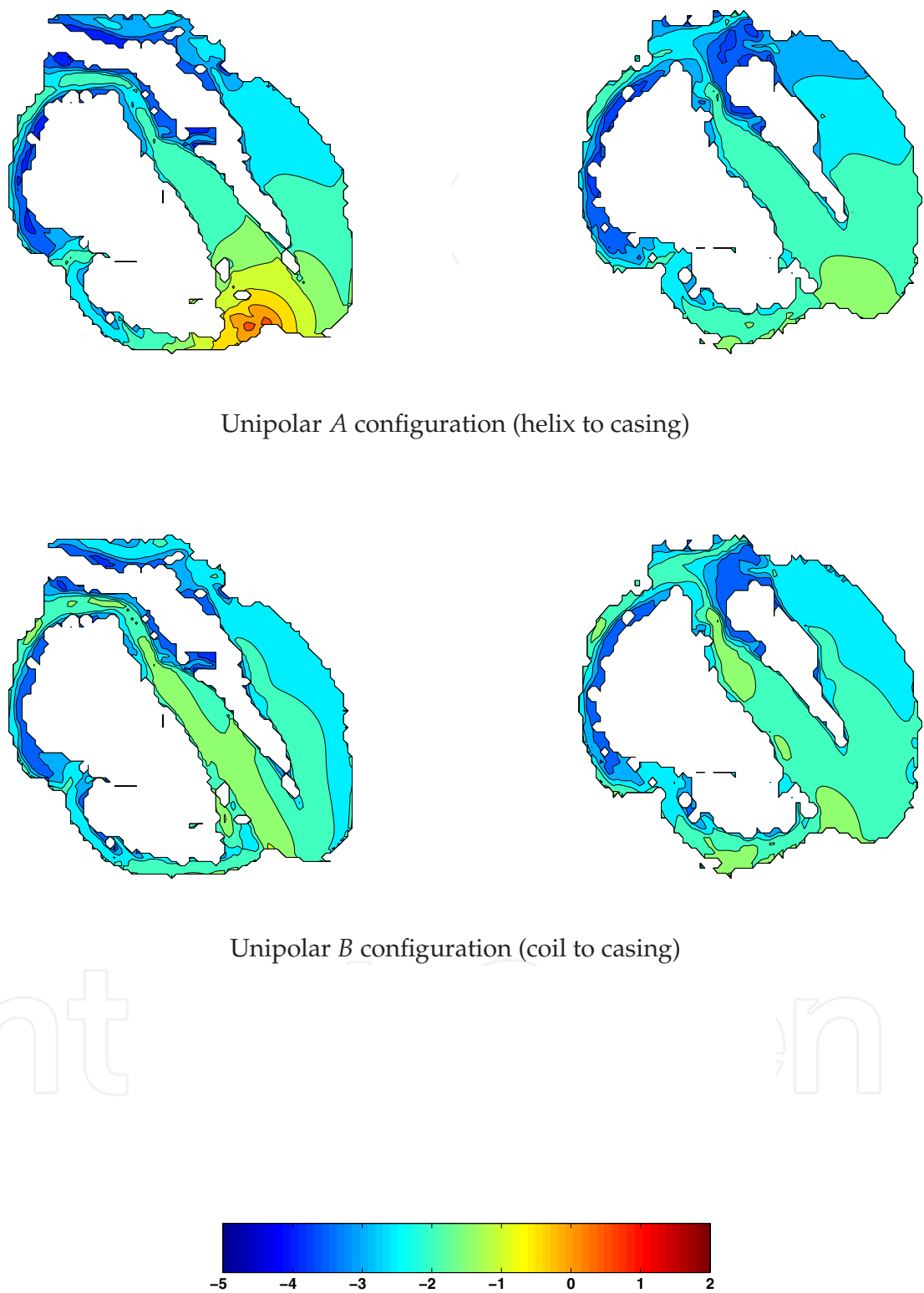
Fig. 1. Sensitivity distributions of unipolar intracardiac configurations at two cross-sections of the heart (arbitrary units, logarithmic scale).
