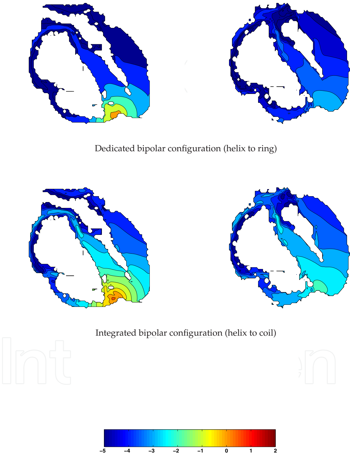
Fig. 2. Sensitivity distributions of bipolar intracardiac configurations at two cross-sections of the heart (arbitrary units, logarithmic scale).
