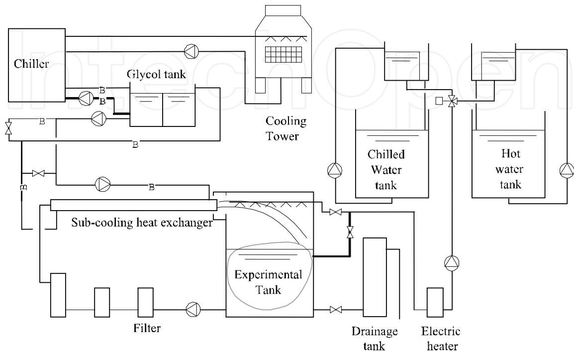
Fig. 13. Schematic diagram of the experimental setup for slurry ice storage
