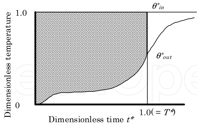
Fig. 2. Response-based efficiency \eta
