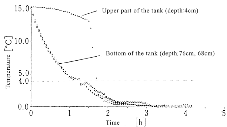
Fig. 7. Freezing process in the experiment using the ice-on-coil ice storage tank
