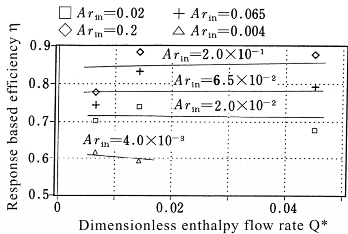
Fig. 11. Relationship between response-based efficiency \eta and inlet conditions
