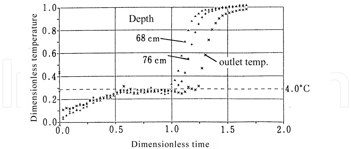
Fig. 9. Melting process for large Archimedes number and moderate inlet enthalpy flow rate
