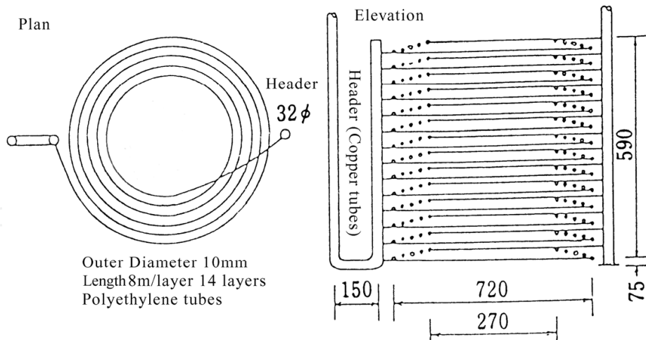
Fig. 6. Structure of the ice making coil
