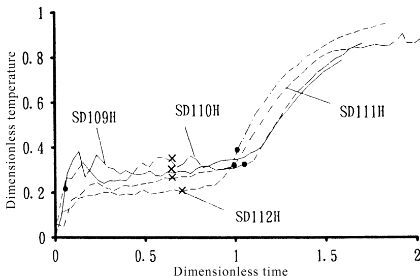
Fig. 16. Dimensionless response of the melting process of slurry ice storage for small inlet enthalpy flow rate
