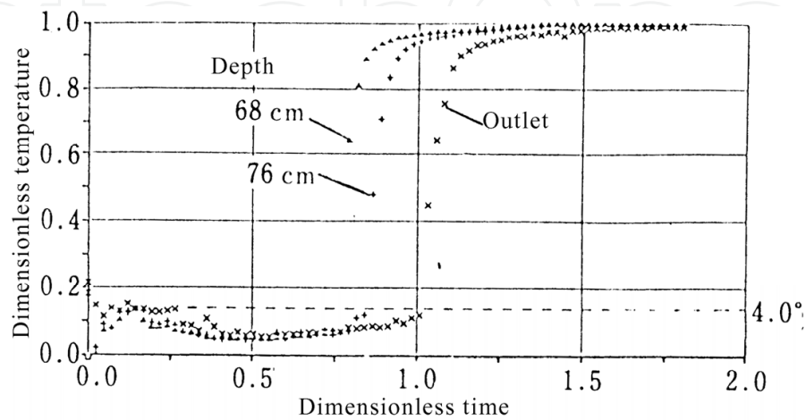
Fig. 8. Melting process for large Archimedes number and inlet enthalpy flow rate
