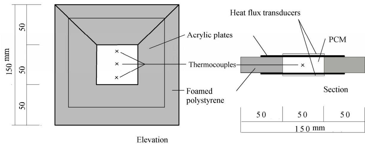
Fig. 17. Experimental apparatus used to measure the thermal properties of the mixtures The apparatus was placed in a small thermal chamber in which both temperature and humidity could be controlled. The temperature inside the chamber was raised from -5^{\circ}\text{C} to 30^{\circ}\text{C} over seven hours. The temperature inside the chamber was maintained at 30^{\circ}\text{C} for three hours and decreased to -5^{\circ}\text{C} over seven hours, before being maintained constant for seven hours. One cycle of the experiment was continued over 24 hours, and seven cycles were repeated for each measurement. The first and last cycles were not used for analysis because of the instability of the experimental conditions.
