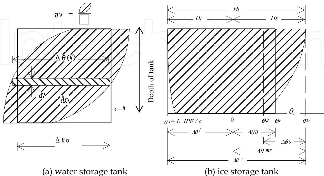
Fig. 4. Definition of tank volume efficiency
