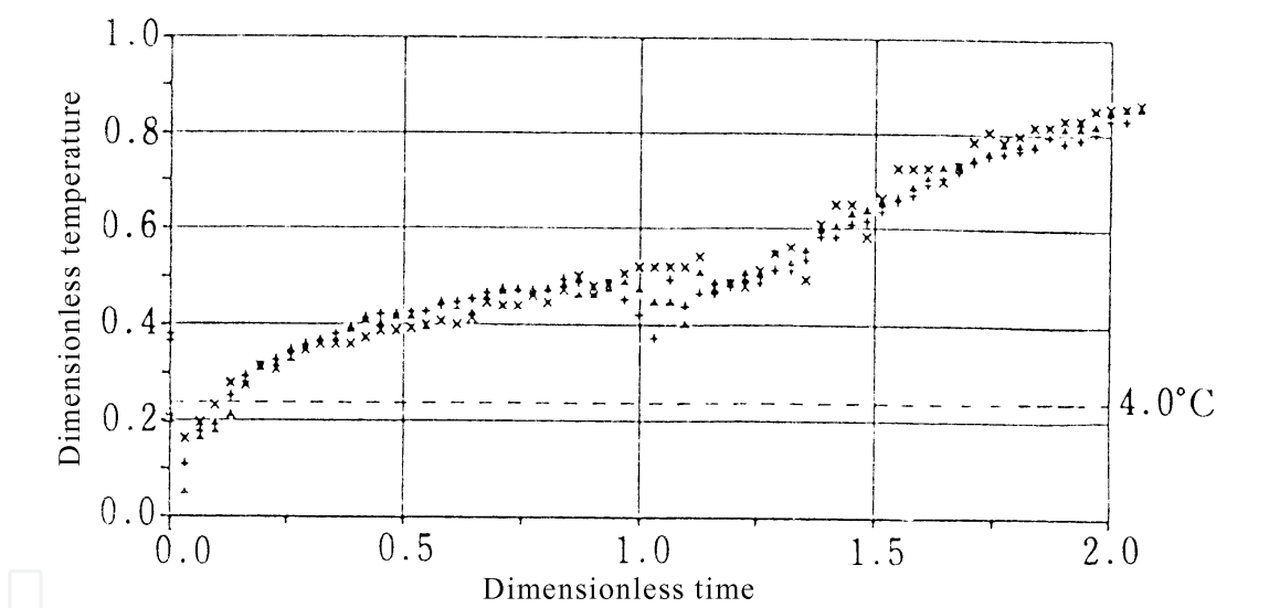
Fig. 10. Melting process for small Archimedes number
