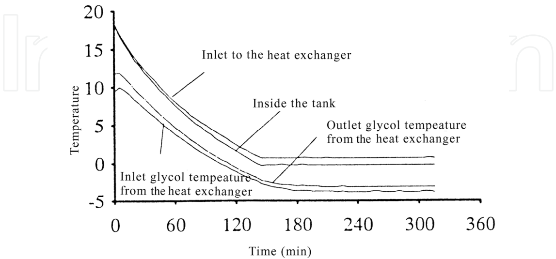
Fig. 14. Freezing process of the slurry ice storage tank
