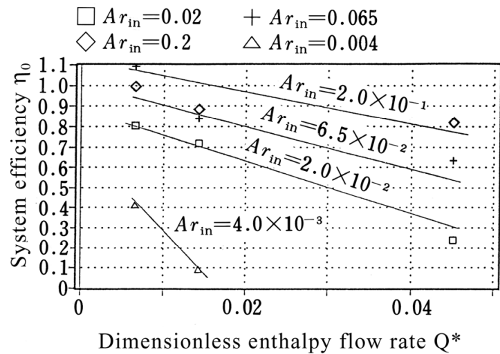
Fig. 12. Relationship between system efficiency \eta_0 and inlet conditions
