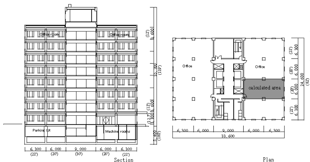
Fig. 19. Section and plan of the building used for simulation
