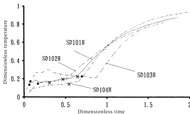
Fig. 15. Dimensionless response of the melting process for slurry ice storage for large inlet enthalpy flow rate
