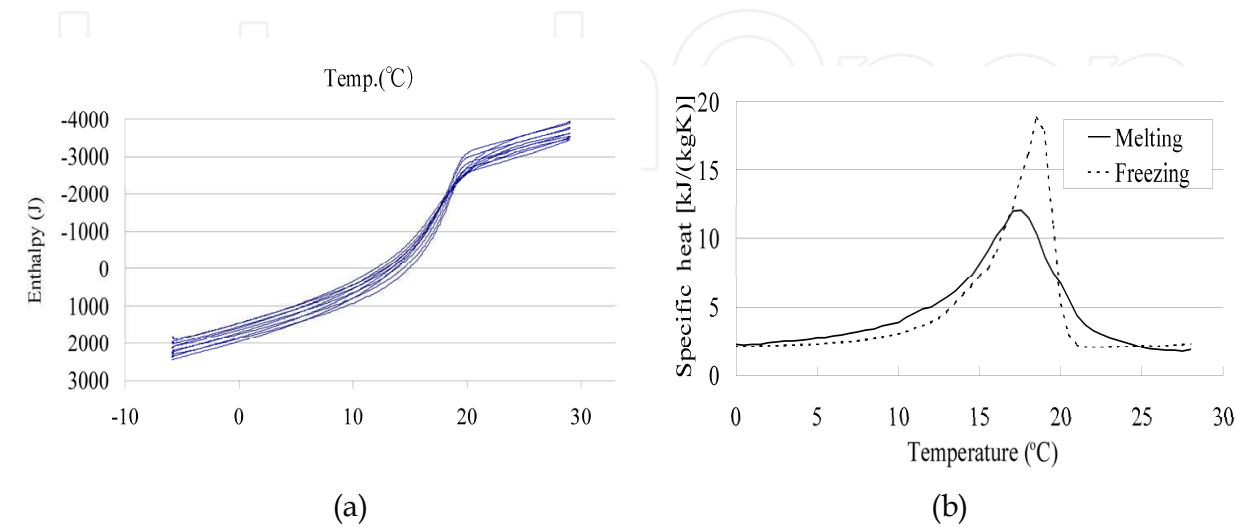
Fig. 18. Results for the MT17 mixture
